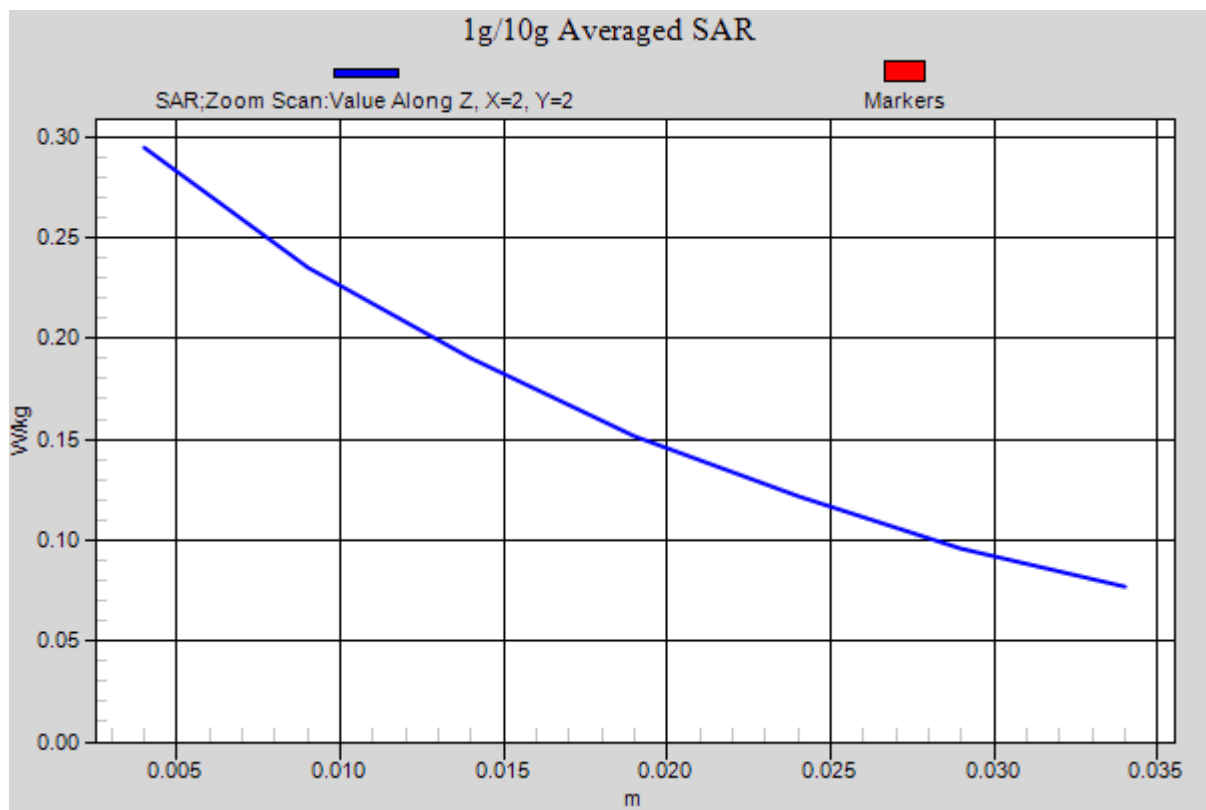
Figure 24 Right Hand Touch Cheek GSM 850 DTM Channel 190
