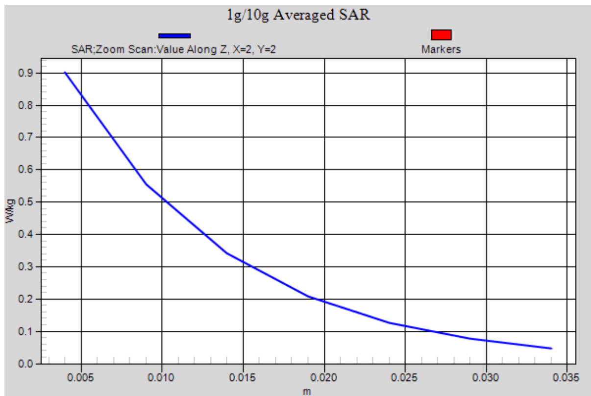
Figure 37 Body, Back Side, LTE Band 4 1RB Channel 20300
