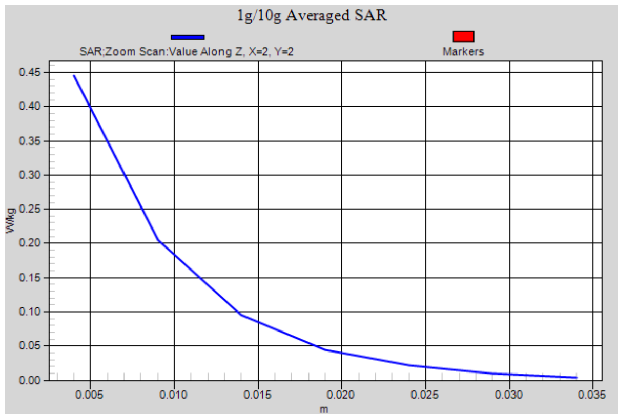
Figure 40 Left Hand Touch Cheek 802.11b Channel 6
