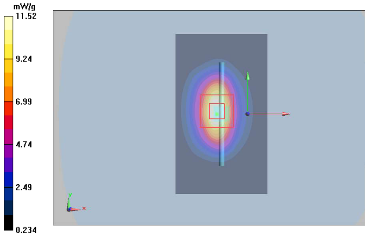
Figure 15 System Performance Check 1900MHz 250mW
