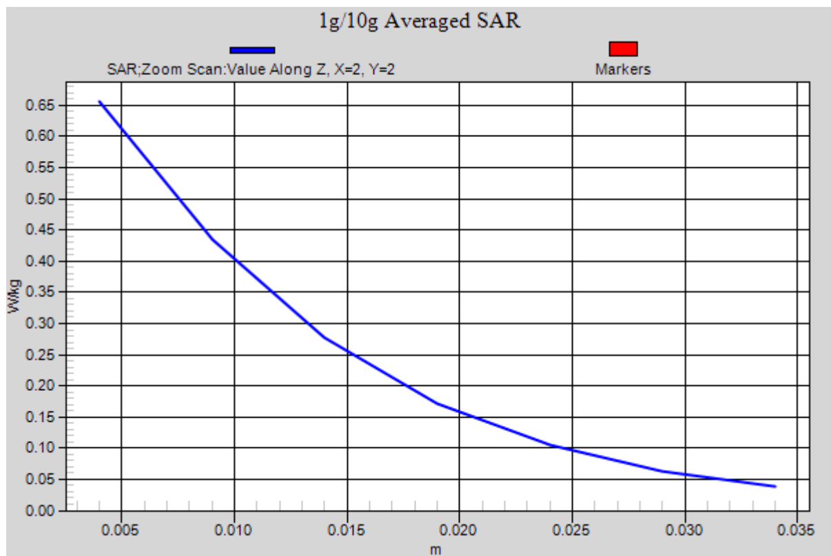
Figure 27 Body, Back Side, GSM 1900 GPRS (4Txslots) Channel 810
