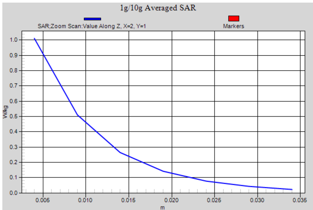
Figure 38 Left Hand Touch Cheek LTE Band 7 1RB Channel 21100
