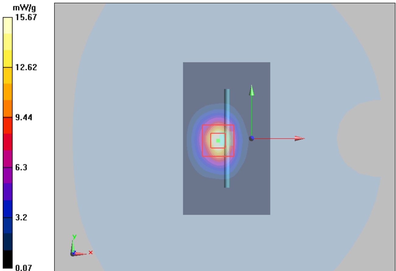
Figure 21 System Performance Check 2600MHz 250mW
