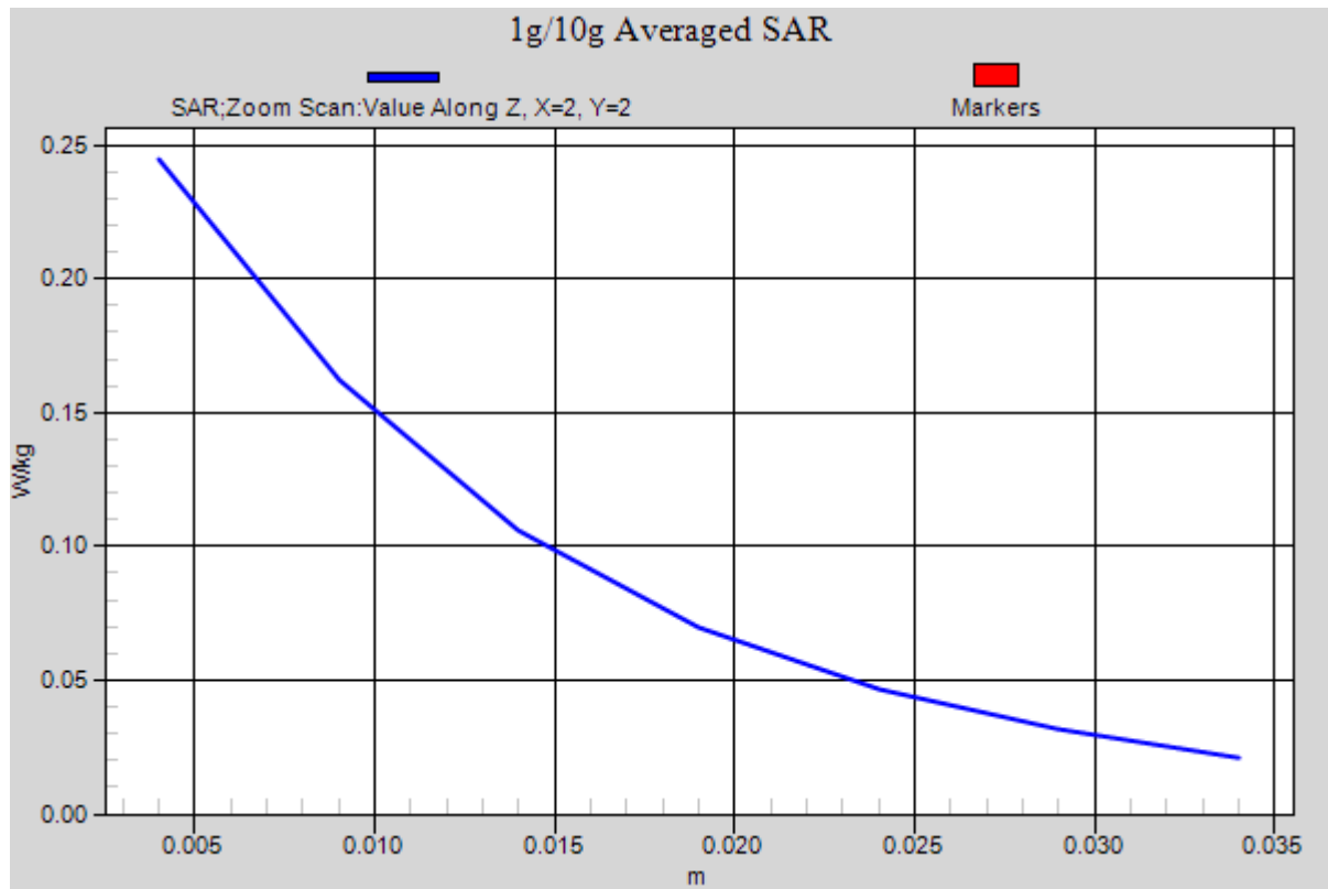
Figure 26 Left Hand Touch Cheek GSM 1900 Channel 661
