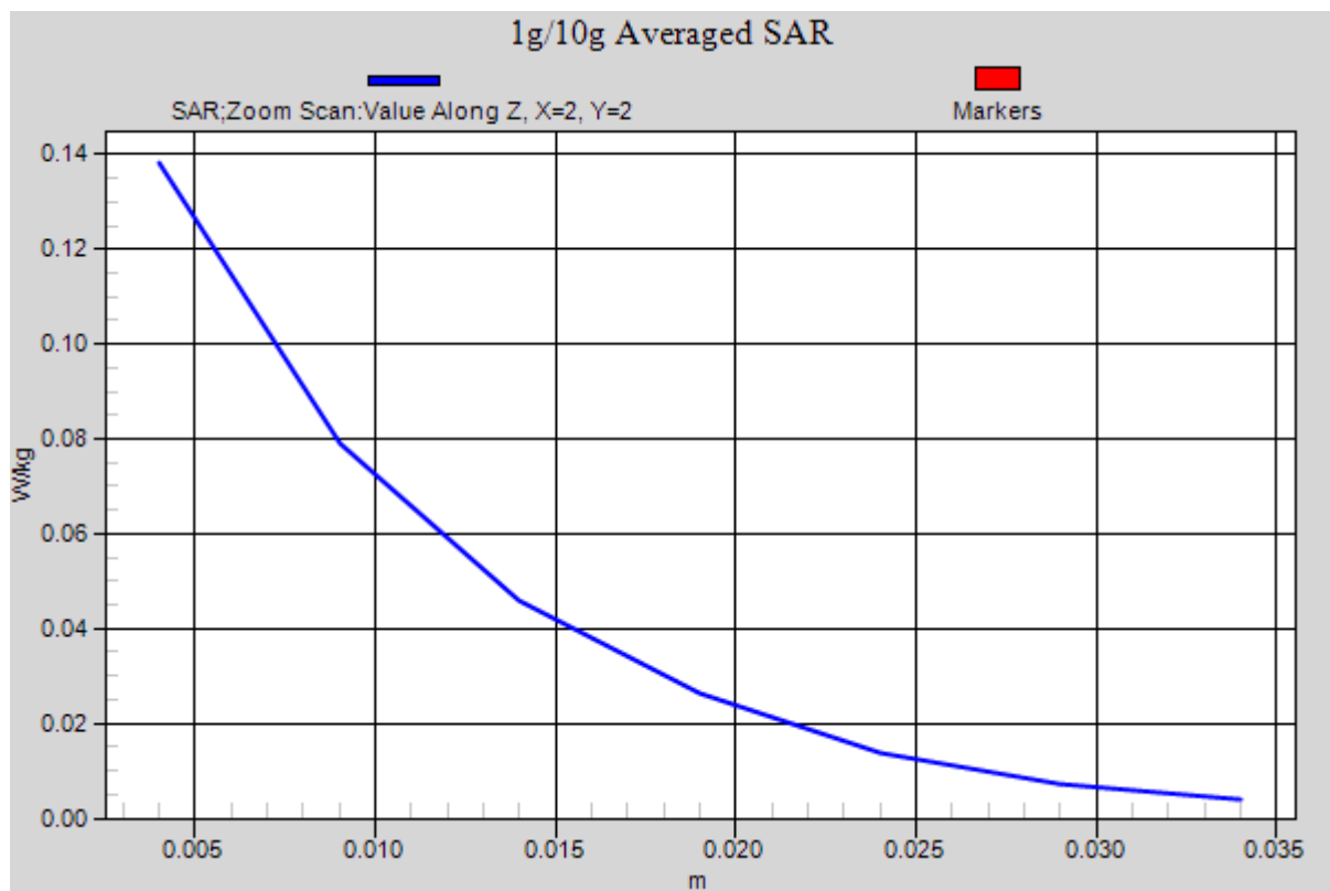
Figure 41 Body, Back Side, 802.11b Channel 6
