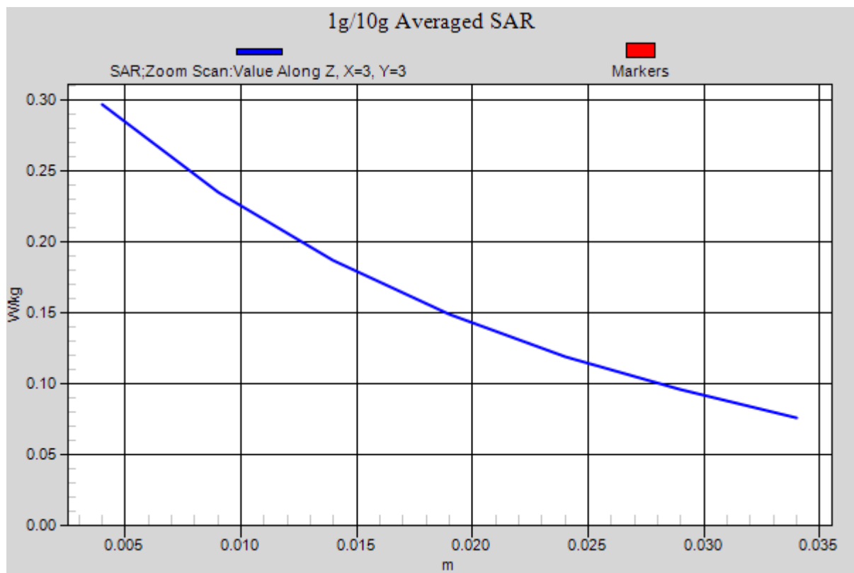
Figure 32 Right Hand Touch Cheek UMTS Band V Channel 4182
