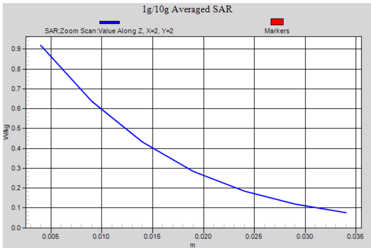
Figure 35 Body, Back Side, LTE Band 2 1RB Channel 18700
