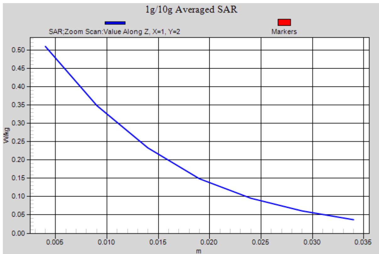
Figure 29 Body, Back Side, GSM 1900 DTM Channel 661
