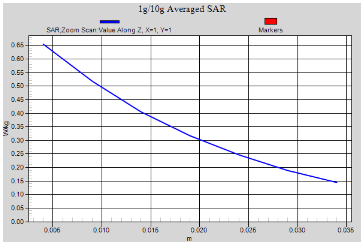
Figure 25 Body, Back Side, GSM 850 DTM Channel 128
