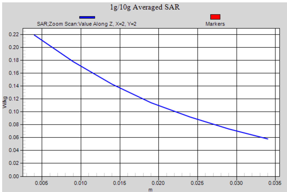
Figure 22 Right Hand Touch Cheek GSM 850 Channel 190
