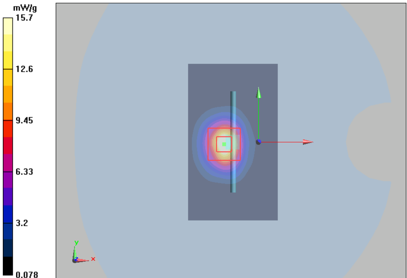
Figure 20 System Performance Check 2600MHz 250mW
