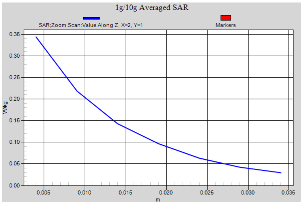
Figure 28 Left Hand Touch Cheek GSM 1900 DTM Channel 661
