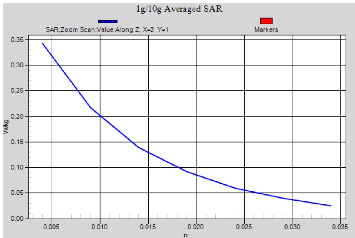
Figure 36 Left Hand Touch Cheek LTE Band 4 1RB Channel 20175
