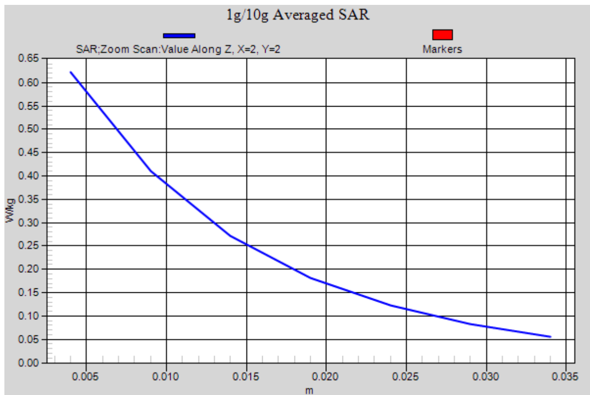
Figure 34 Left Hand Touch Cheek LTE Band 2 1RB Channel 19100
