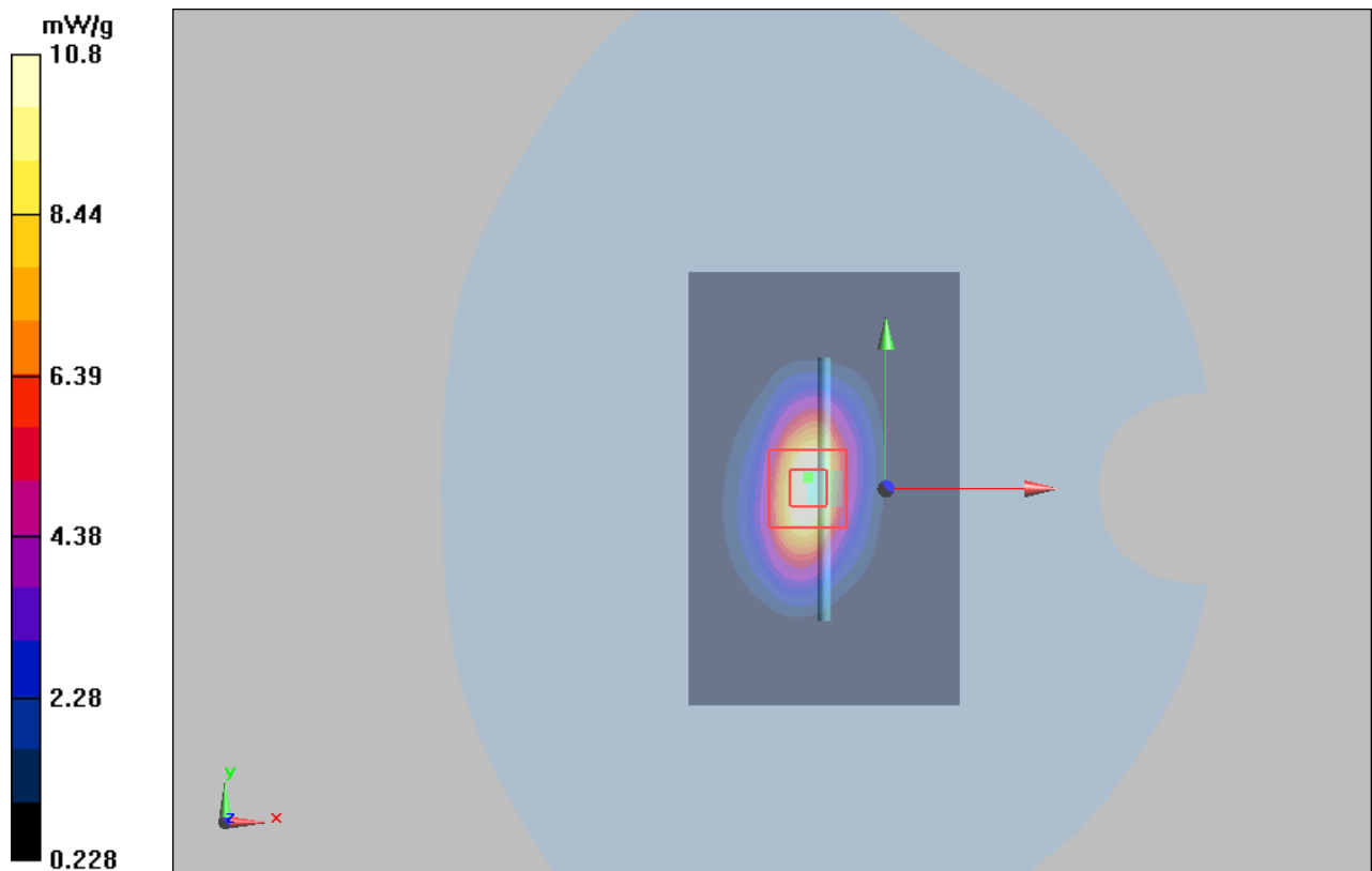
Figure 11 System Performance Check 1750MHz 250mW
