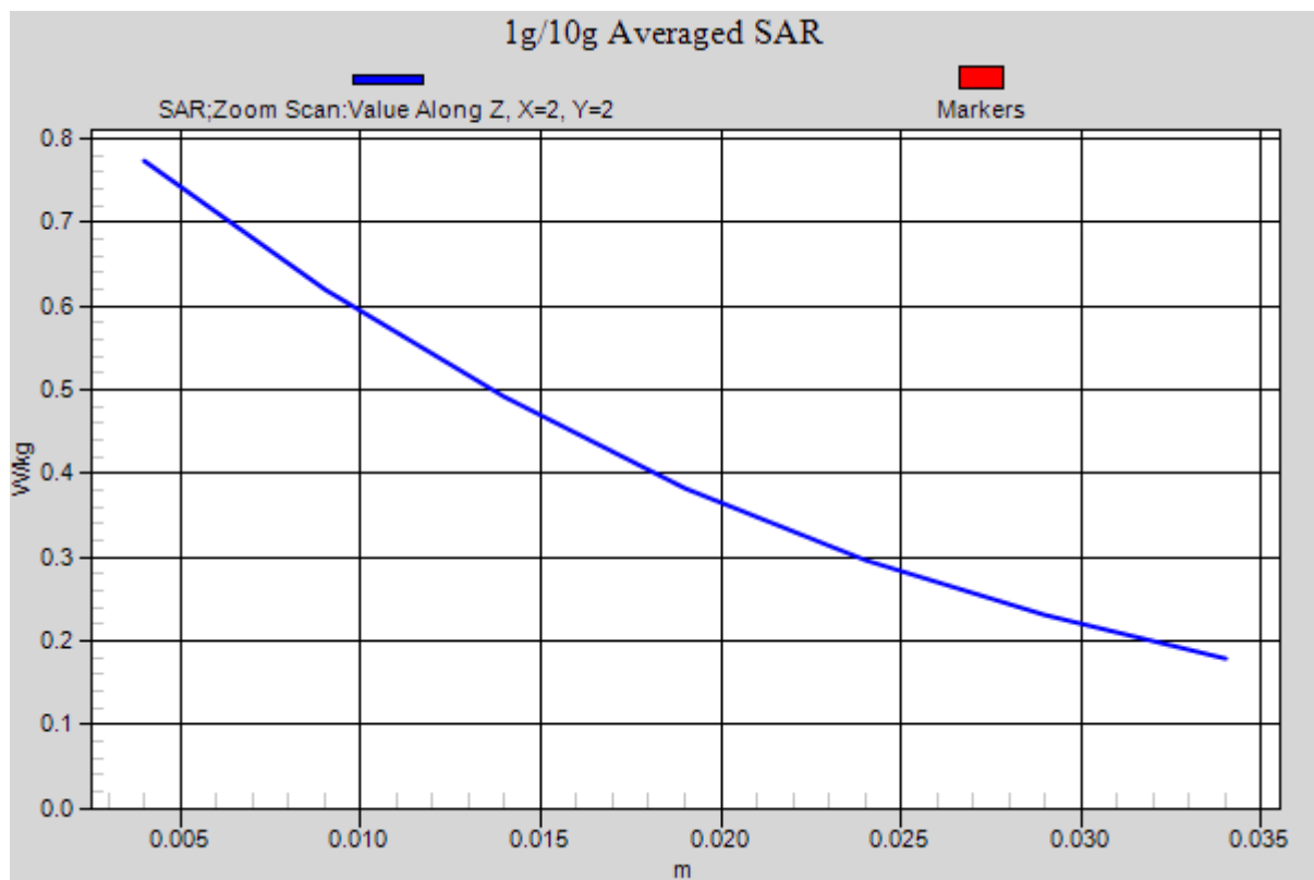
Figure 23 Body, Back Side, GSM 850 GPRS (4Txslots) Channel 128
