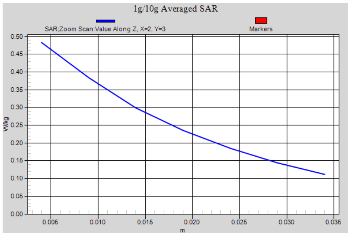
Figure 33 Body, Back Side, UMTS Band V Channel 4182
