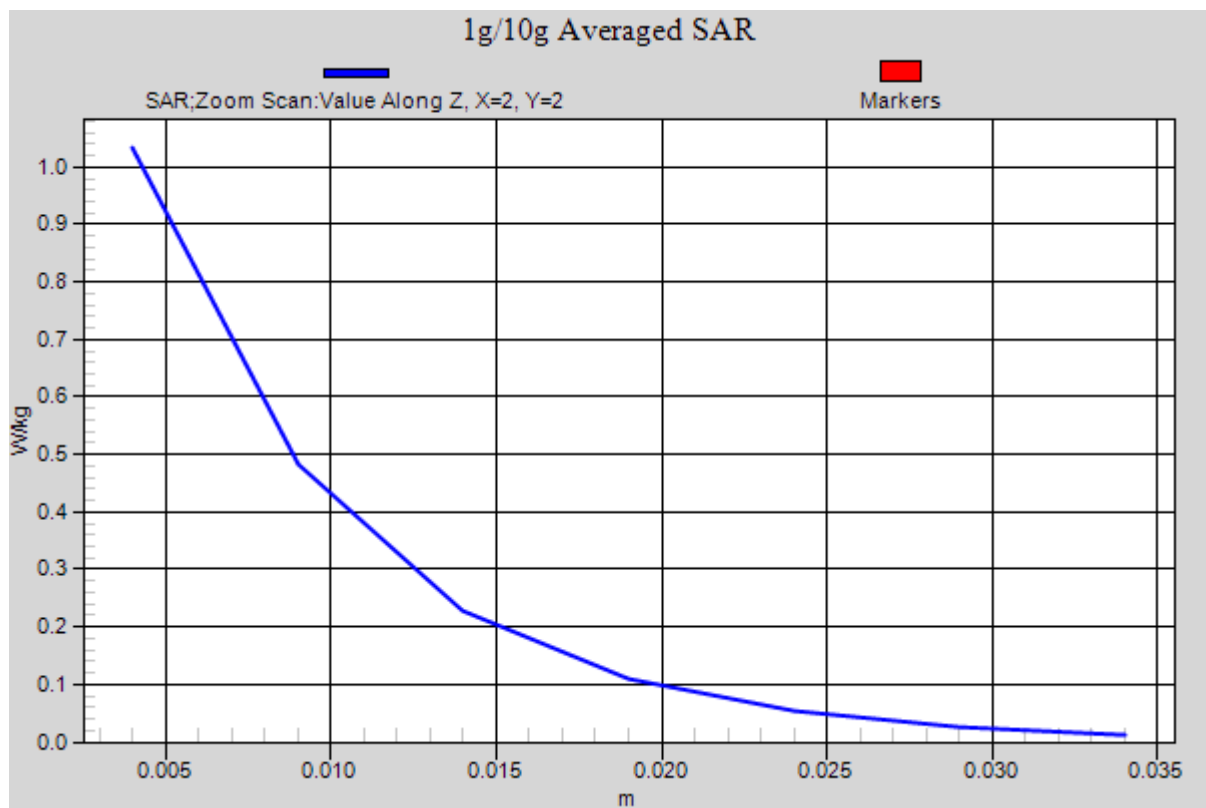
Figure 39 Body, Back Side, LTE Band 7 1RB Channel 21100
