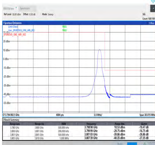
1-N78-3700-3800-30-20-H-5-CP-QPSK-Edge_1RB_Right-1@50-Ant1-1--PASS-see graph
