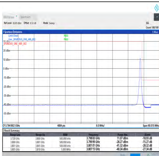
1-N78-3700-3800-30-80-H-2-DFT-PI2BPSK-Edge_1R B_Right-1@216-Ant1-1--PASS-see graph
