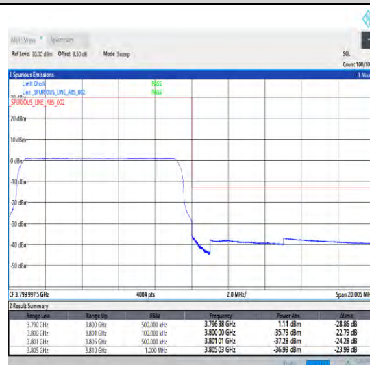
1-N78-3700-3800-30-10-H-6-CP-QPSK-Outer_Full-24@0-Ant1-1--PASS-see graph
