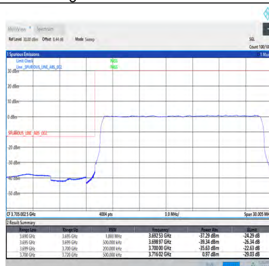
1-N78-3700-3800-30-20-L-3-DFT-PI2BPSK-Outer _Full-50@0-Ant1-1--PASS-see graph
