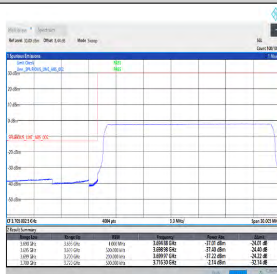
1-N78-3700-3800-30-20-L-6-CP-QPSK-Outer_Full -51@0-Ant1-1--PASS-see graph
