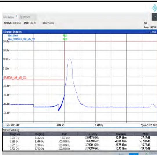
1-N78-3700-3800-30-15-L-4-CP-QPSK-Edge_1RB_Lef t-1@0-Ant1-1--PASS-see graph
