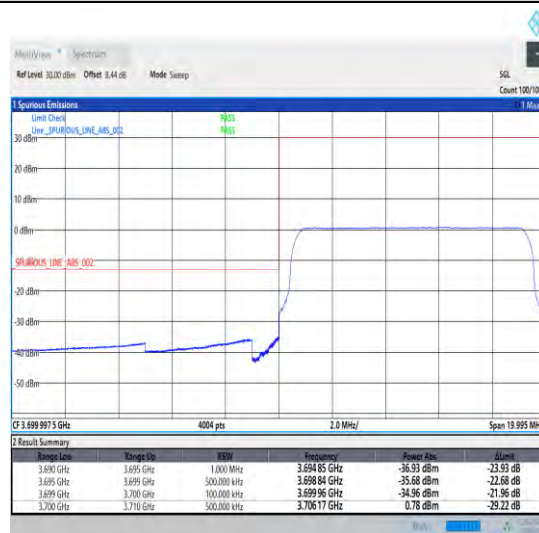
1-N78-3700-3800-30-10-L-6-CP-QPSK-Outer_Full -24@0-Ant1-1--PASS-see graph
