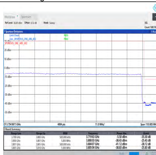
1-N78-3700-3800-30-100-H-3-DFT-PI2BPSK-Outer_Full-270@0-Ant1-1--PASS-see graph
