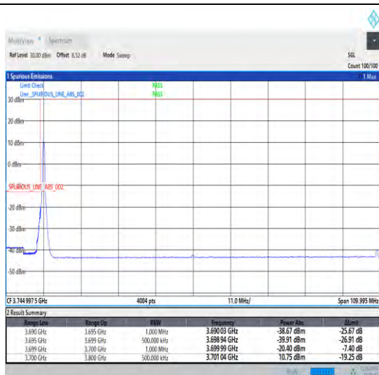
1-N78-3700-3800-30-100-L-1-DFT-PI2BPSK-Edge_1R_B_Left-1@0-Ant1-1--PASS-see graph
