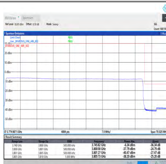
1-N78-3700-3800-30-60-H-6-CP-QPSK-Outer_Full -162@0-Ant1-1--PASS-see graph
