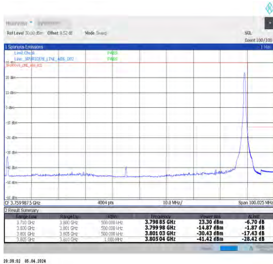
1-N78-3700-3800-N78-3700-380030-90-H-5-CP-QPS K-Edge_1RB_Right-1@244-Ant1-1--PASS-see graph
