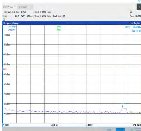
1-N78-3700-3800-30-100-M-1-DFT-QPSK-Edge_1R B_Left-1@0-0.009-0.15-Ant1-0.13--83.59--43-PASS
