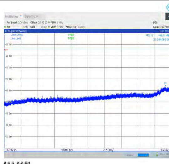
1-N78-3700-3800-N78-3700-380030-100-M-1-DFT-PI2BPSK-Inner_1RB_Left-1@1-18000-40000-Ant1-18 506.49--46.81--13-PASS
