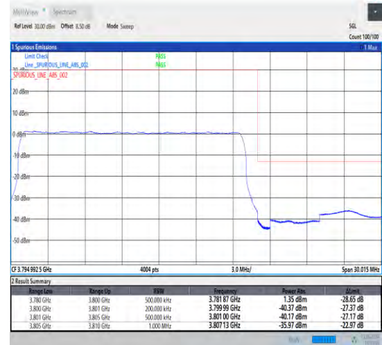
1-N78-3700-3800-30-20-H-3-DFT-PI2BPSK-Outer_Full-50@0-Ant1-1--PASS-see graph
