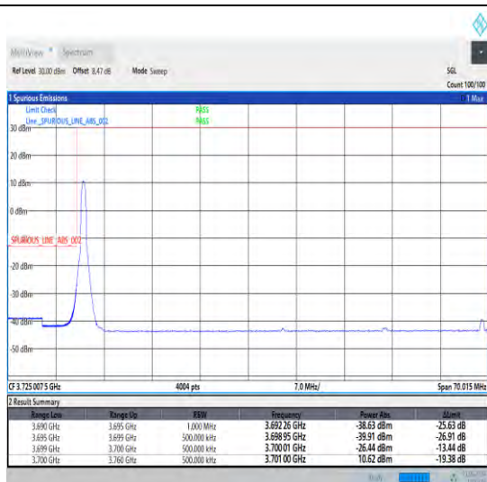
1-N78-3700-3800-30-60-L-1-DFT-PI2BPSK-Edge_1RB _Left-1@0-Ant1-1--PASS-see graph
