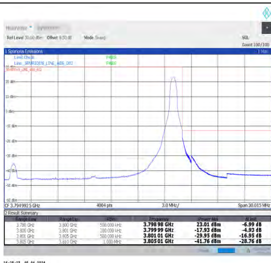
1-N78-3700-3800-N78-3700-380030-20-H-2-DFT-PI2 BPSK-Edge_1RB_Right-1@50-Ant1-1--PASS-see graph
