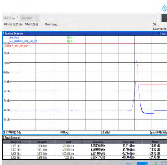
1-N78-3700-3800-30-50-H-2-DFT-PI2BPSK-Edge_1R B_Right-1@132-Ant1-1--PASS-see graph
