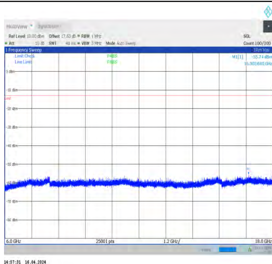
1-N78-3700-3800-N78-3700-380030-100-M-1-DFT-PI2BPSK-Inner_1RB_Left-1@1-6000-18000-Ant1-11 104.32--55.74--13-PASS
