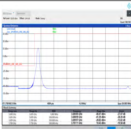
1-N78-3700-3800-30-30-L-4-CP-QPSK-Edge_1RB_Lef t-1@0-Ant1-1--PASS-see graph
