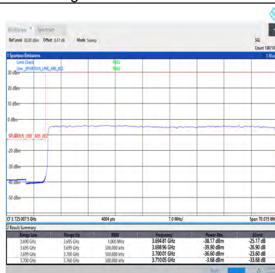
1-N78-3700-3800-30-60-L-3-DFT-PI2BPSK-Outer _Full-162@0-Ant1-1--PASS-see graph
