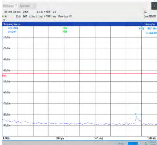
1-N78-3700-3800-30-100-H-1-DFT-QPSK-Edge_1R B_Left-1@0-0.009-0.15-Ant1-0.13--83.37--43-PASS
