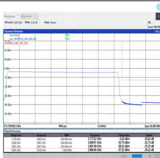
1-N78-3700-3800-30-30-H-6-CP-QPSK-Outer_Full-78@0-Ant1-1--PASS-see graph
