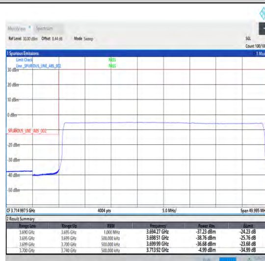
1-N78-3700-3800-30-40-L-6-CP-QPSK-Outer_Full -106@0-Ant1-1--PASS-see graph
