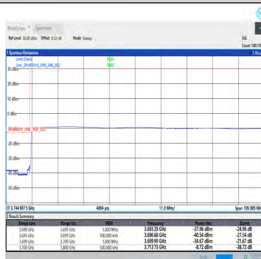
1-N78-3700-3800-30-100-L-6-CP-QPSK-Outer_Full-273@0-Ant1-1--PASS-see graph
