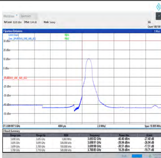
1-N78-3700-3800-30-10-L-4-CP-QPSK-Edge_1RB_Lef t-1@0-Ant1-1--PASS-see graph
