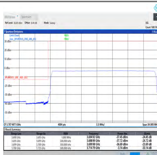
1-N78-3700-3800-30-25-L-6-CP-QPSK-Outer_Full -65@0-Ant1-1--PASS-see graph
