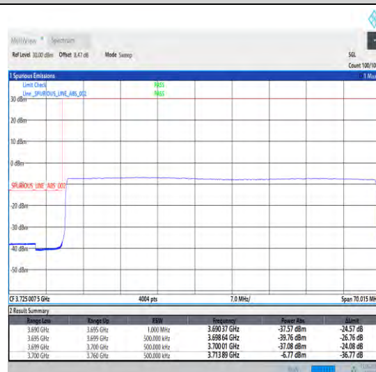
1-N78-3700-3800-30-60-L-6-CP-QPSK-Outer_Full -162@0-Ant1-1--PASS-see graph
