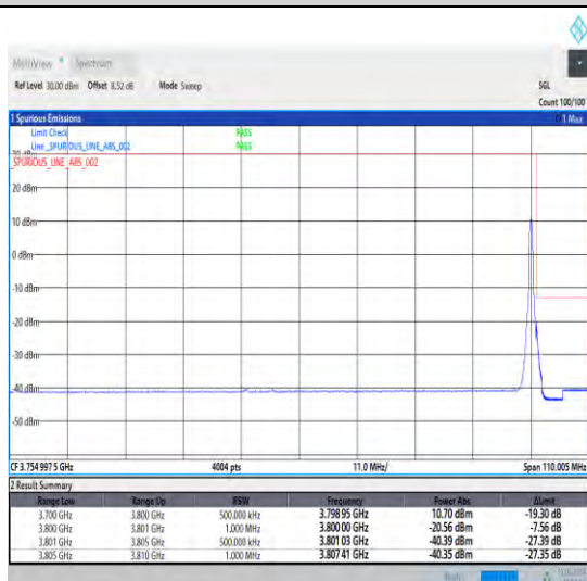
1-N78-3700-3800-30-100-H-5-CP-QPSK-Edge_1RB_Right-1@272-Ant1-1--PASS-see graph
