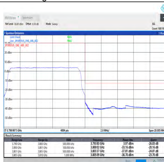
1-N78-3700-3800-30-10-H-3-DFT-PI2BPSK-Outer_Full-24@0-Ant1-1--PASS-see graph
