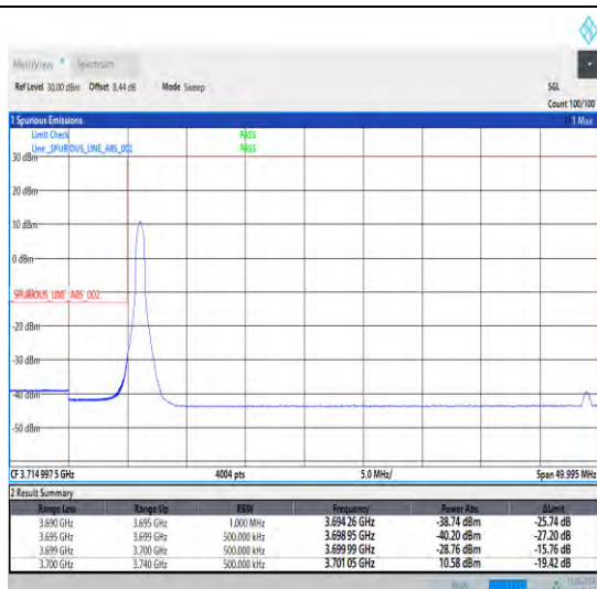
1-N78-3700-3800-30-40-L-1-DFT-PI2BPSK-Edge_1RB _Left-1@0-Ant1-1--PASS-see graph
