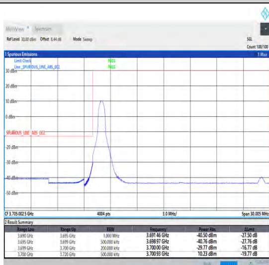
1-N78-3700-3800-30-20-L-4-CP-QPSK-Edge_1RB_Lef t-1@0-Ant1-1--PASS-see graph
