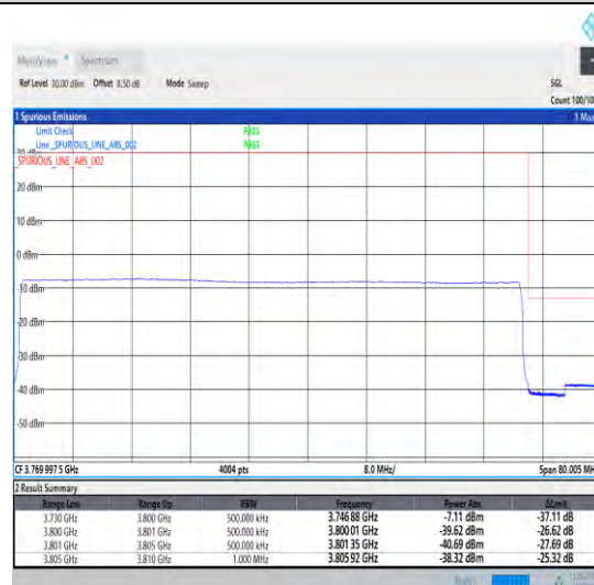
1-N78-3700-3800-30-70-H-6-CP-QPSK-Outer_Full -189@0-Ant1-1--PASS-see graph
