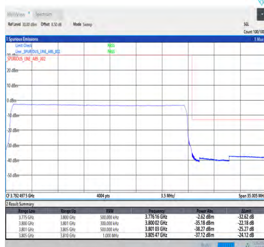
1-N78-3700-3800-30-25-H-6-CP-QPSK-Outer_Full-65@0-Ant1-1--PASS-see graph
