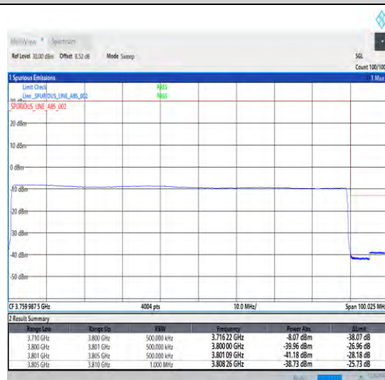
1-N78-3700-3800-30-90-H-6-CP-QPSK-Outer_Full -245@0-Ant1-1--PASS-see graph
