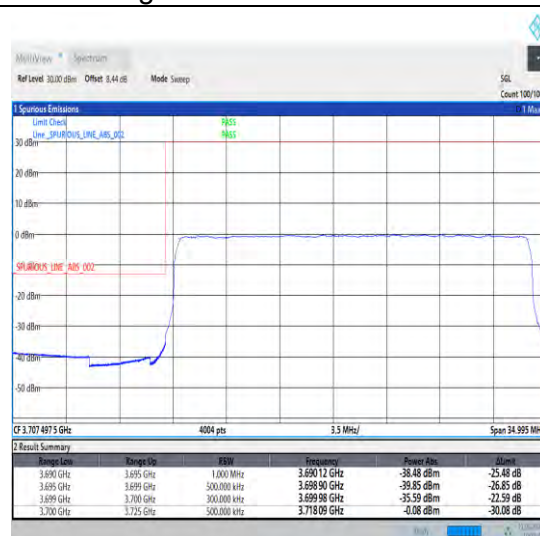
1-N78-3700-3800-30-25-L-3-DFT-PI2BPSK-Outer _Full-64@0-Ant1-1--PASS-see graph
