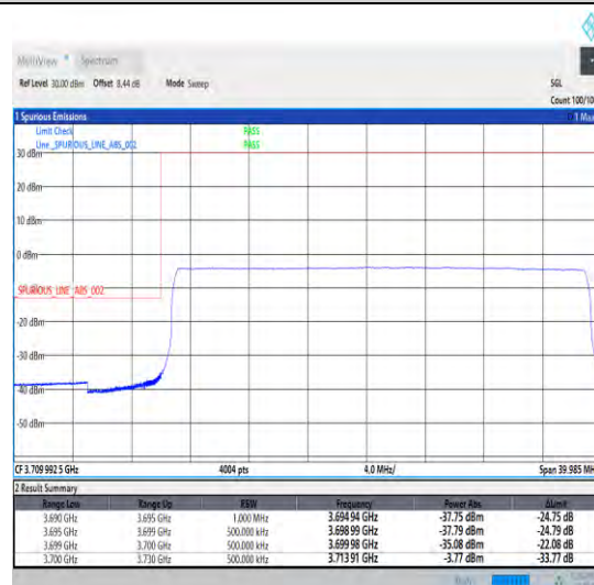
1-N78-3700-3800-30-30-L-6-CP-QPSK-Outer_Full -78@0-Ant1-1--PASS-see graph
