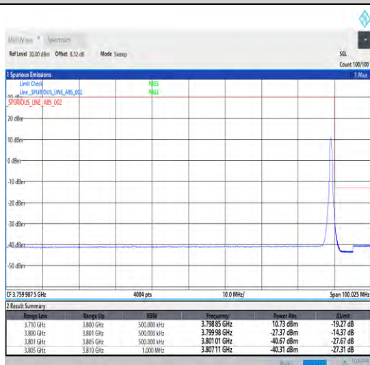
1-N78-3700-3800-30-90-H-5-CP-QPSK-Edge_1RB_Ri ght-1@244-Ant1-1--PASS-see graph
