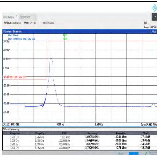
1-N78-3700-3800-30-25-L-1-DFT-PI2BPSK-Edge_1RB _Left-1@0-Ant1-1--PASS-see graph
