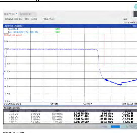
1-N78-3700-3800-N78-3700-380030-30-H-3-DFT- PI2BPSK-Outer_Full-75@0-Ant1-1--PASS-see graph
