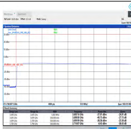
1-N78-3700-3800-30-90-L-6-CP-QPSK-Outer_Full -245@0-Ant1-1--PASS-see graph
