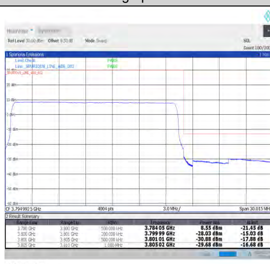
1-N78-3700-3800-N78-3700-380030-20-H-3-DFT-PI2BPSK-Outer_Full-50@0-Ant1-1--PASS-see graph
