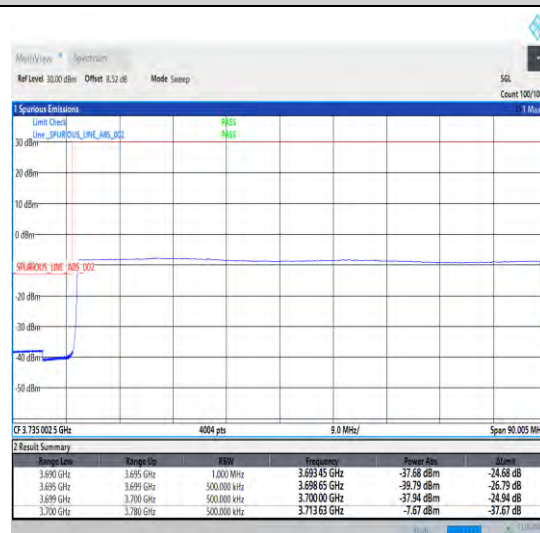
1-N78-3700-3800-30-80-L-6-CP-QPSK-Outer_Full -217@0-Ant1-1--PASS-see graph
