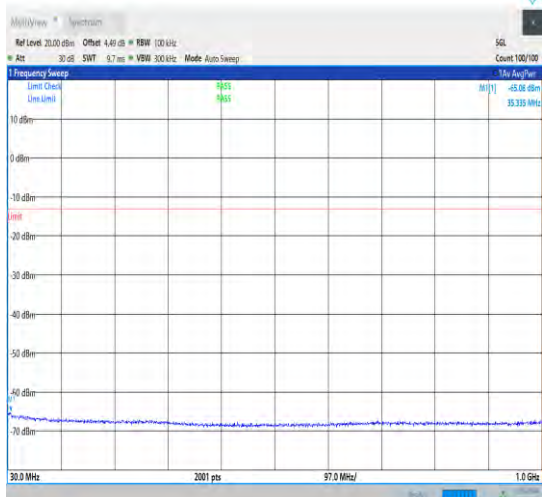
1-N78-3700-3800-30-100-H-1-DFT-QPSK-Edge_1R B_Left-1@0-30-1000-Ant1-35.34--65.08--13-PASS
