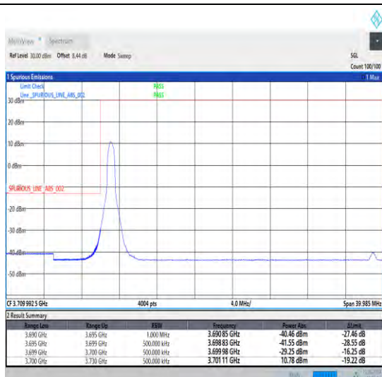
1-N78-3700-3800-30-30-L-1-DFT-PI2BPSK-Edge_1RB_Left-1@0-Ant1-1--PASS-see graph
