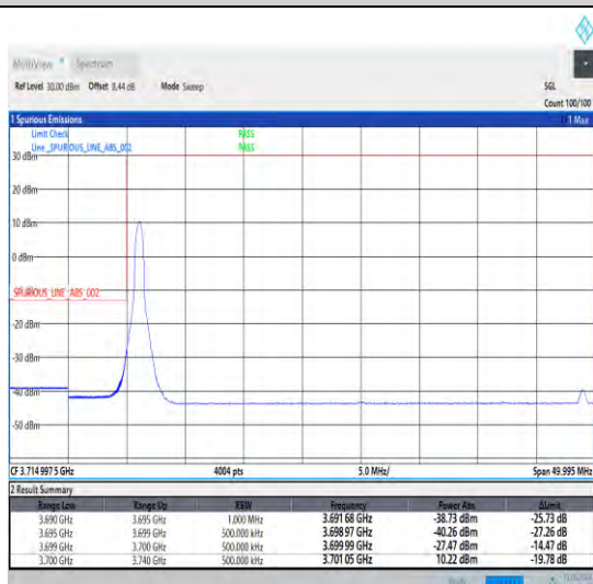
1-N78-3700-3800-30-40-L-4-CP-QPSK-Edge_1RB_Lef t-1@0-Ant1-1--PASS-see graph
