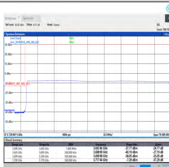
1-N78-3700-3800-30-70-L-6-CP-QPSK-Outer_Full -189@0-Ant1-1--PASS-see graph
