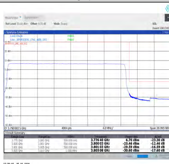
1-N78-3700-3800-N78-3700-380030-30-H-6-CP-Q PSK-Outer_Full-78@0-Ant1-1--PASS-see graph
