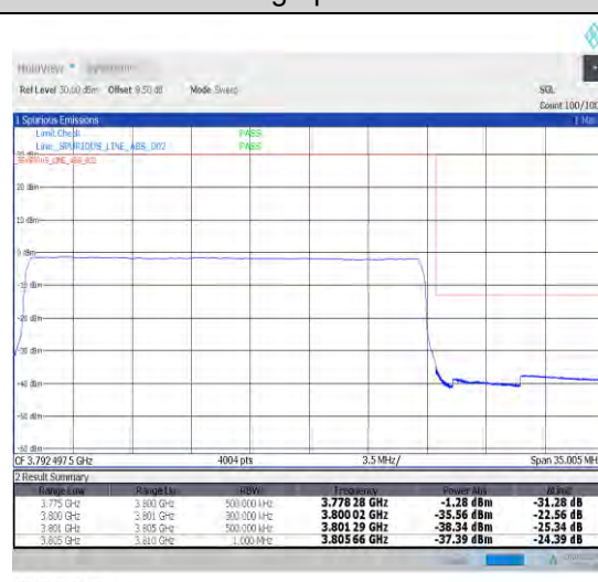
1-N78-3700-3800-N78-3700-380030-25-H-3-DFT-PI2 BPSK-Outer_Full-64@0-Ant1-1--PASS-see graph
