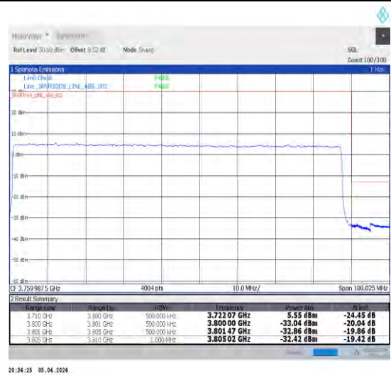
1-N78-3700-3800-N78-3700-380030-90-H-3-DFT- PI2BPSK-Outer_Full-240@0-Ant1-1--PASS-see graph
