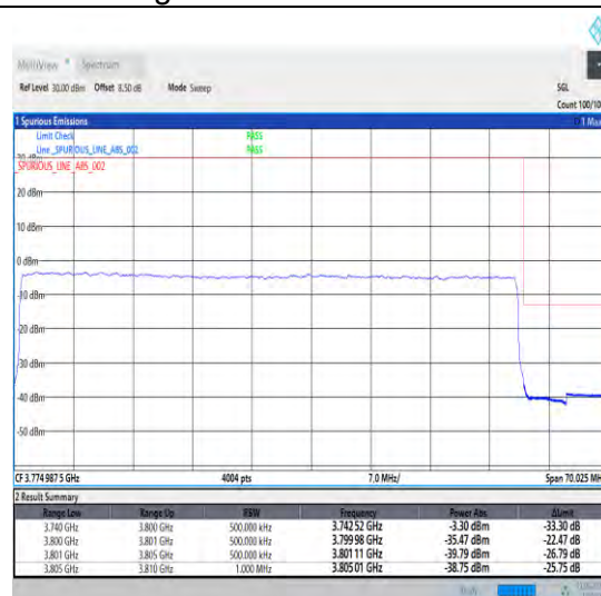
1-N78-3700-3800-30-60-H-3-DFT-PI2BPSK-Outer _Full-162@0-Ant1-1--PASS-see graph
