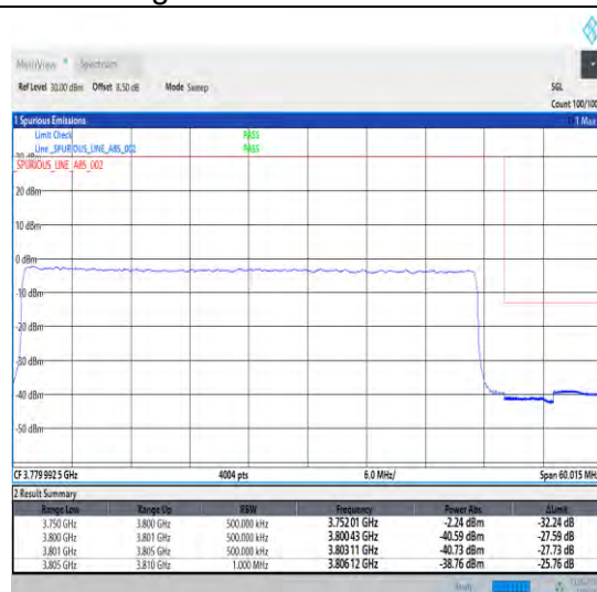
1-N78-3700-3800-30-50-H-3-DFT-PI2BPSK-Outer _Full-128@0-Ant1-1--PASS-see graph
