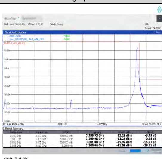
1-N78-3700-3800-N78-3700-380030-60-H-5-CP-QPS K-Edge_1RB_Right-1@161-Ant1-1--PASS-see graph
