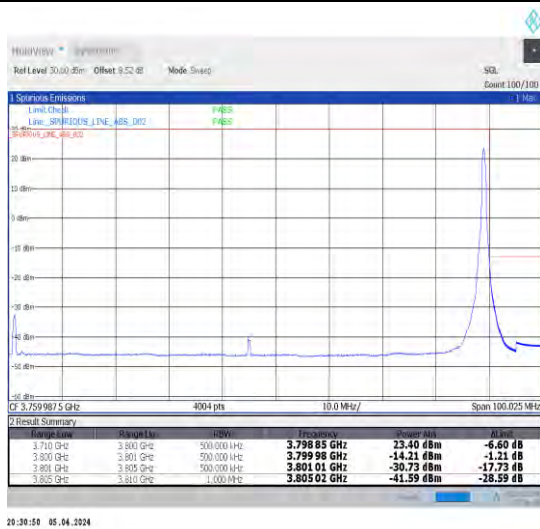
1-N78-3700-3800-N78-3700-380030-90-H-2-DFT-PI2 BPSK-Edge_1RB_Right-1@244-Ant1-1--PASS-see graph
