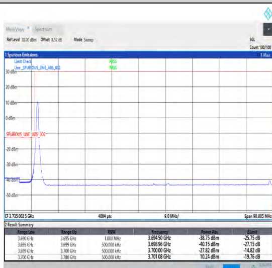
1-N78-3700-3800-30-80-L-4-CP-QPSK-Edge_1RB_Lef t-1@0-Ant1-1--PASS-see graph
