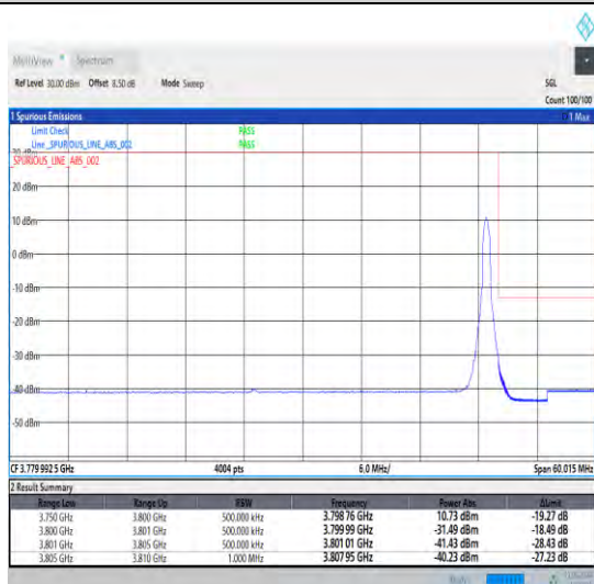
1-N78-3700-3800-30-50-H-5-CP-QPSK-Edge_1RB_Ri ght-1@132-Ant1-1--PASS-see graph
