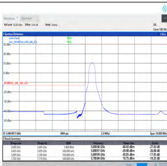
1-N78-3700-3800-30-10-L-1-DFT-PI2BPSK-Edge_1RB _Left-1@0-Ant1-1--PASS-see graph
