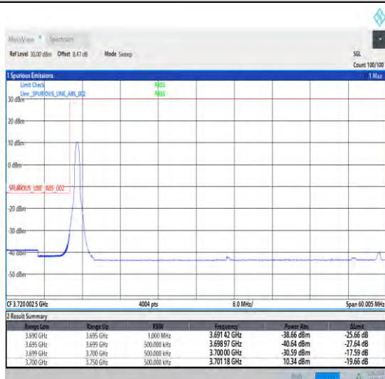
1-N78-3700-3800-30-50-L-4-CP-QPSK-Edge_1RB_Lef t-1@0-Ant1-1--PASS-see graph
