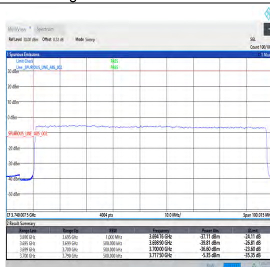
1-N78-3700-3800-30-90-L-3-DFT-PI2BPSK-Outer _Full-240@0-Ant1-1--PASS-see graph
