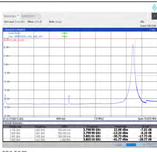
1-N78-3700-3800-N78-3700-380030-60-H-2-DFT-PI2 BPSK-Edge_1RB_Right-1@161-Ant1-1--PASS-see graph
