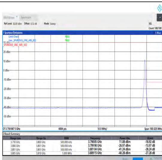
1-N78-3700-3800-30-90-H-2-DFT-PI2BPSK-Edge_1R B_Right-1@244-Ant1-1--PASS-see graph
