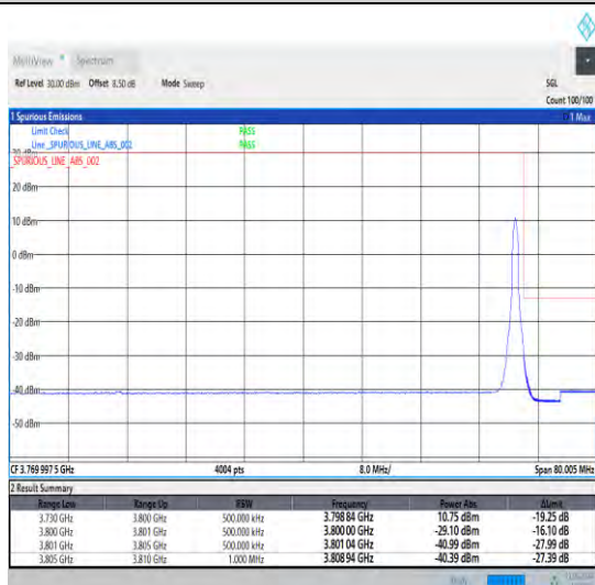
1-N78-3700-3800-30-70-H-5-CP-QPSK-Edge_1RB_Ri ght-1@188-Ant1-1--PASS-see graph
