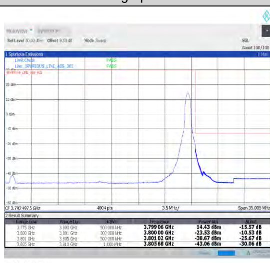
1-N78-3700-3800-N78-3700-380030-25-H-2-DFT-PI2 BPSK-Edge_1RB_Right-1@64-Ant1-1--PASS-see graph
