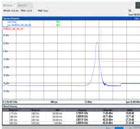
1-N78-3700-3800-30-25-H-2-DFT-PI2BPSK-Edge_1R_B_Right-1@64-Ant1-1--PASS-see graph
