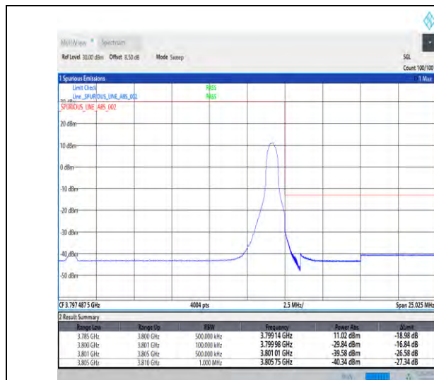
1-N78-3700-3800-30-15-H-2-DFT-PI2BPSK-Edge_1R_B_Right-1@37-Ant1-1--PASS-see graph
