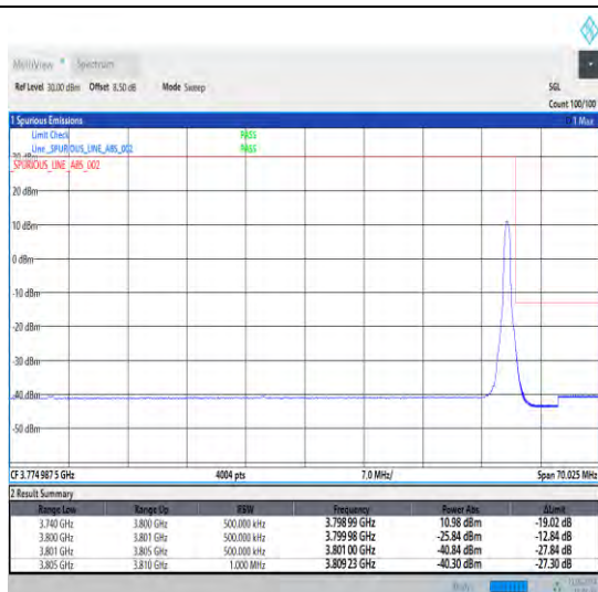
1-N78-3700-3800-30-60-H-2-DFT-PI2BPSK-Edge_1R B_Right-1@161-Ant1-1--PASS-see graph
