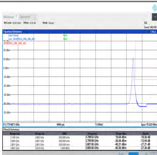
1-N78-3700-3800-30-60-H-5-CP-QPSK-Edge_1RB_Ri ght-1@161-Ant1-1--PASS-see graph
