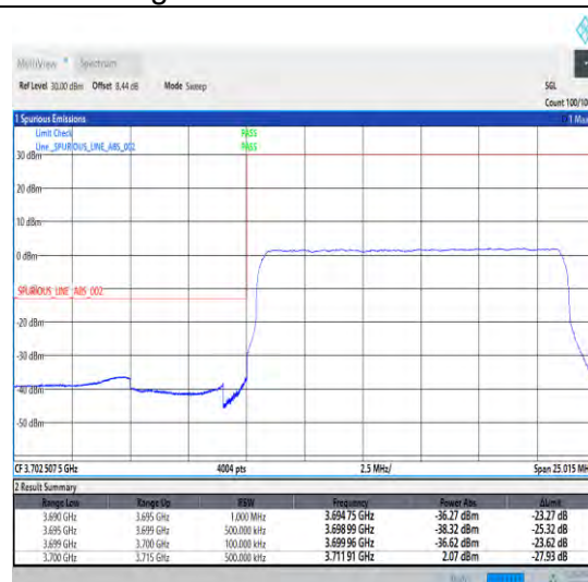
1-N78-3700-3800-30-15-L-3-DFT-PI2BPSK-Outer _Full-36@0-Ant1-1--PASS-see graph
