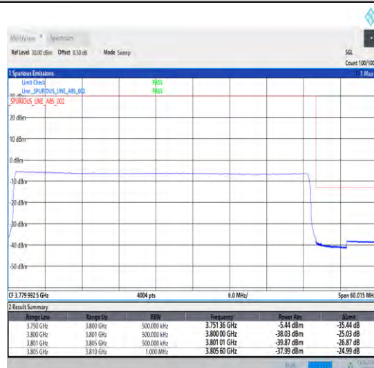
1-N78-3700-3800-30-50-H-6-CP-QPSK-Outer_Full -133@0-Ant1-1--PASS-see graph
