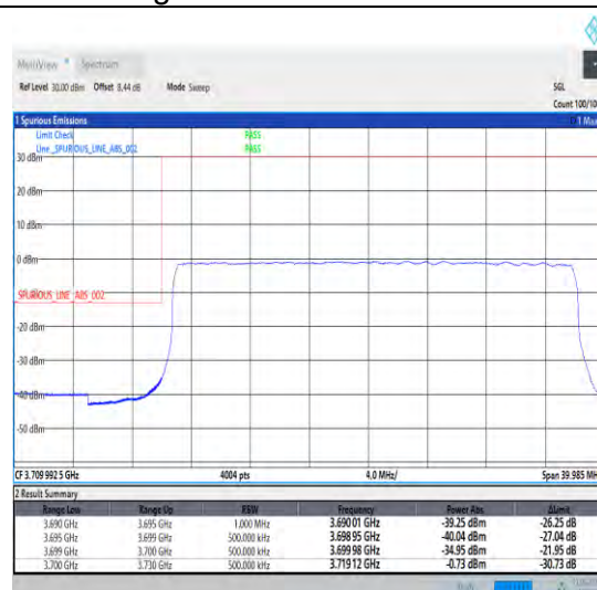
1-N78-3700-3800-30-30-L-3-DFT-PI2BPSK-Outer_Full-75@0-Ant1-1--PASS-see graph
