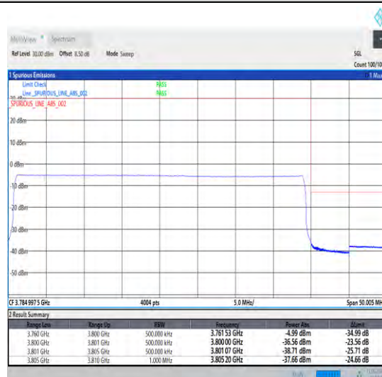
1-N78-3700-3800-30-40-H-6-CP-QPSK-Outer_Full -106@0-Ant1-1--PASS-see graph
