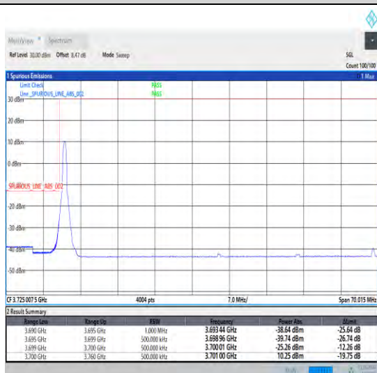
1-N78-3700-3800-30-60-L-4-CP-QPSK-Edge_1RB_Lef t-1@0-Ant1-1--PASS-see graph
