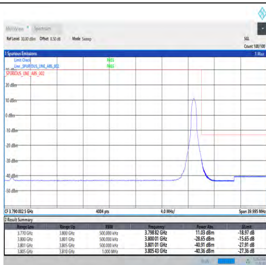
1-N78-3700-3800-30-30-H-2-DFT-PI2BPSK-Edge_1R_B_Right-1@77-Ant1-1--PASS-see graph
