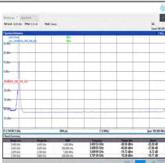
1-N78-3700-3800-30-100-L-4-CP-QPSK-Edge_1RB_Left-1@0-Ant1-1--PASS-see graph
