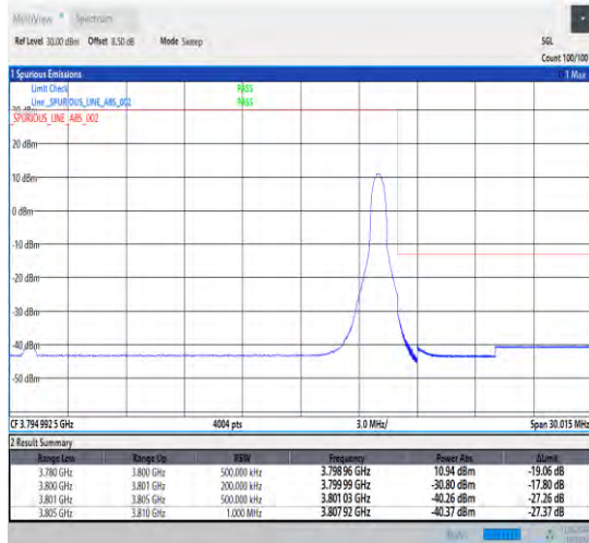
1-N78-3700-3800-30-20-H-2-DFT-PI2BPSK-Edge_1R_B_Right-1@50-Ant1-1--PASS-see graph
