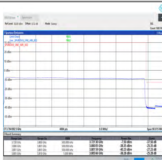
1-N78-3700-3800-30-80-H-6-CP-QPSK-Outer_Full _-217@0-Ant1-1--PASS-see graph
