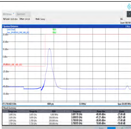
1-N78-3700-3800-30-20-L-1-DFT-PI2BPSK-Edge_1RB _Left-1@0-Ant1-1--PASS-see graph
