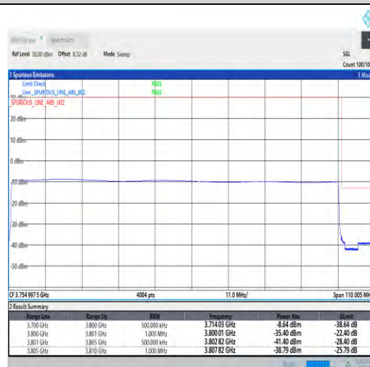
1-N78-3700-3800-30-100-H-6-CP-QPSK-Outer_Full-273@0-Ant1-1--PASS-see graph
