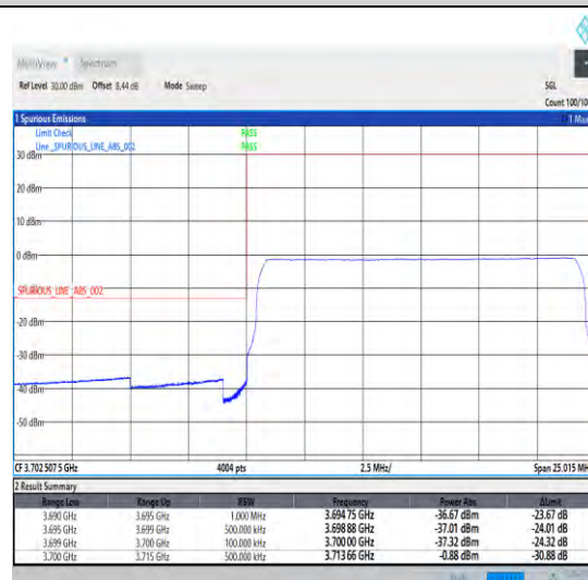
1-N78-3700-3800-30-15-L-6-CP-QPSK-Outer_Full -38@0-Ant1-1--PASS-see graph
