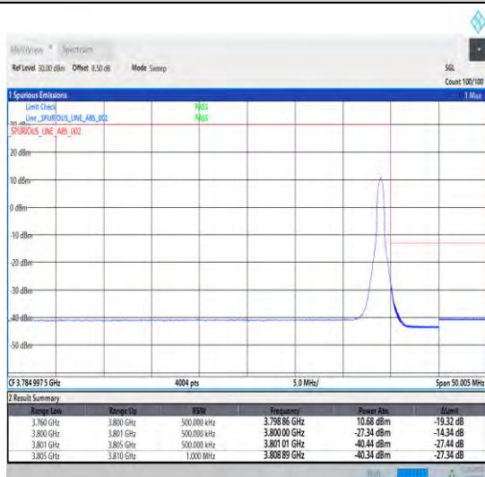
1-N78-3700-3800-30-40-H-5-CP-QPSK-Edge_1RB_Ri ght-1@105-Ant1-1--PASS-see graph
