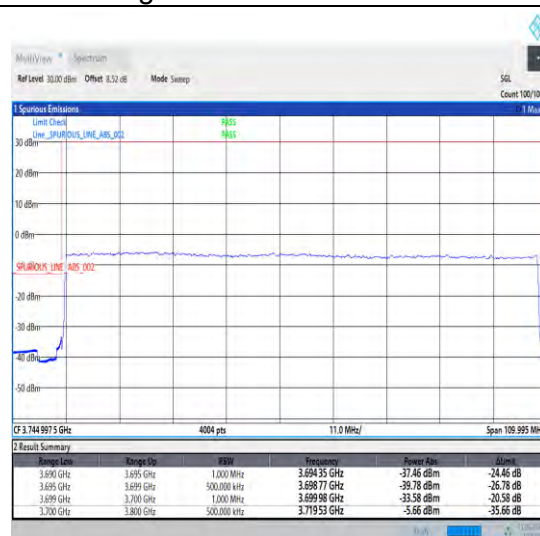
1-N78-3700-3800-30-100-L-3-DFT-PI2BPSK-Outer_Full-270@0-Ant1-1--PASS-see graph
