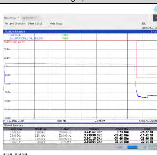
1-N78-3700-3800-N78-3700-380030-60-H-6-CP-Q PSK-Outer_Full-162@0-Ant1-1--PASS-see graph
