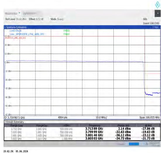
1-N78-3700-3800-N78-3700-380030-90-H-6-CP-Q PSK-Outer_Full-245@0-Ant1-1--PASS-see graph
