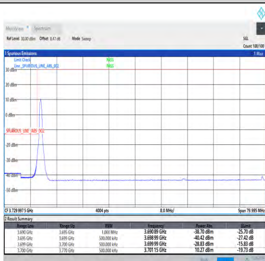
1-N78-3700-3800-30-70-L-4-CP-QPSK-Edge_1RB_Lef t-1@0-Ant1-1--PASS-see graph
