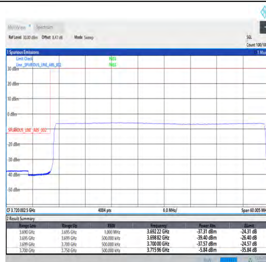
1-N78-3700-3800-30-50-L-6-CP-QPSK-Outer_Full -133@0-Ant1-1--PASS-see graph
