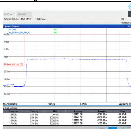
1-N78-3700-3800-30-50-L-3-DFT-PI2BPSK-Outer _Full-128@0-Ant1-1--PASS-see graph
