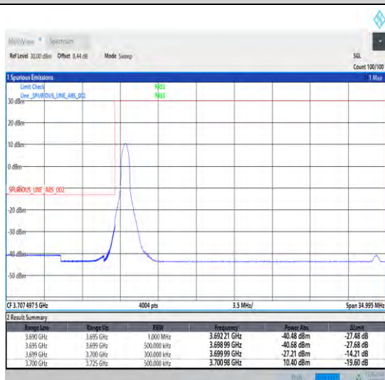
1-N78-3700-3800-30-25-L-4-CP-QPSK-Edge_1RB_Lef t-1@0-Ant1-1--PASS-see graph
