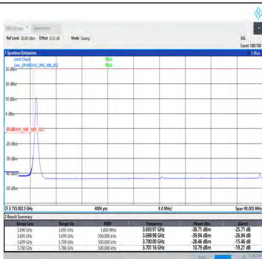
1-N78-3700-3800-30-80-L-1-DFT-PI2BPSK-Edge_1RB _Left-1@0-Ant1-1--PASS-see graph
