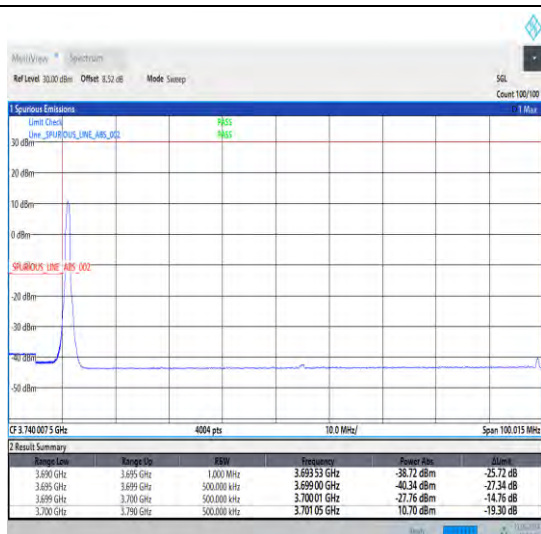
1-N78-3700-3800-30-90-L-1-DFT-PI2BPSK-Edge_1RB _Left-1@0-Ant1-1--PASS-see graph
