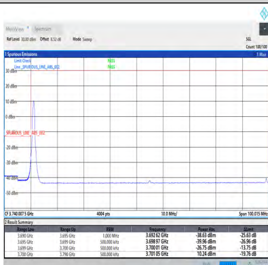
1-N78-3700-3800-30-90-L-4-CP-QPSK-Edge_1RB_Lef t-1@0-Ant1-1--PASS-see graph
