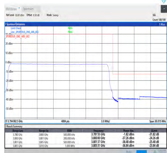
1-N78-3700-3800-30-20-H-6-CP-QPSK-Outer_Full-51@0-Ant1-1--PASS-see graph
