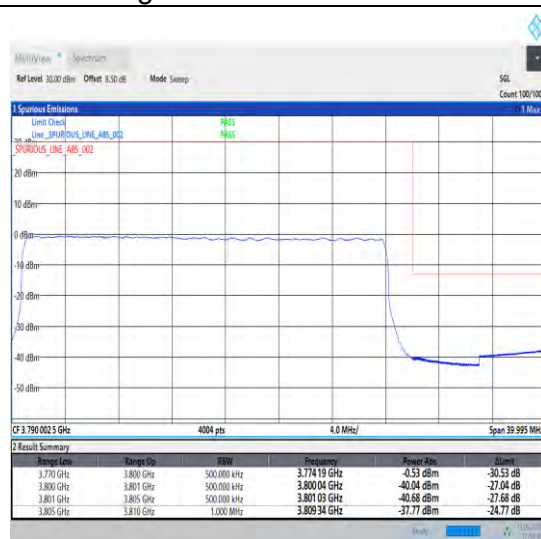
1-N78-3700-3800-30-30-H-3-DFT-PI2BPSK-Outer_Full-75@0-Ant1-1--PASS-see graph
