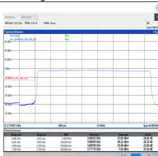
1-N78-3700-3800-30-40-L-3-DFT-PI2BPSK-Outer _Full-100@0-Ant1-1--PASS-see graph
