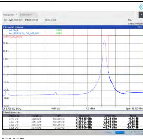
1-N78-3700-3800-N78-3700-380030-30-H-2-DFT-PI2 BPSK-Edge_1RB_Right-1@77-Ant1-1--PASS-see graph
