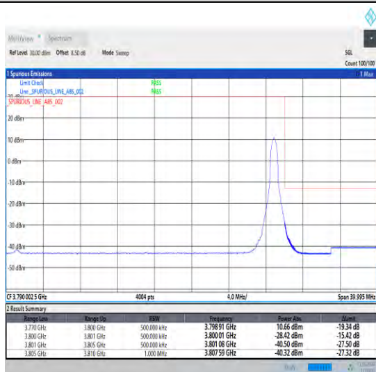
1-N78-3700-3800-30-30-H-5-CP-QPSK-Edge_1RB_Right-1@77-Ant1-1--PASS-see graph
