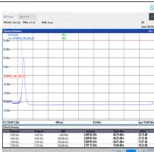
1-N78-3700-3800-30-70-L-1-DFT-PI2BPSK-Edge_1RB _Left-1@0-Ant1-1--PASS-see graph
