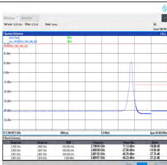
1-N78-3700-3800-30-40-H-2-DFT-PI2BPSK-Edge_1R B_Right-1@105-Ant1-1--PASS-see graph
