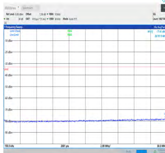
1-N78-3700-3800-30-100-M-1-DFT-QPSK-Edge_1R B_Left-1@0-0.15-30-Ant1-29.70--77.41--33-PASS
