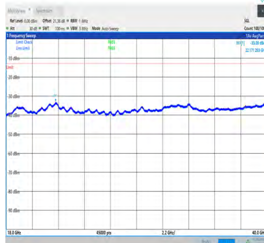
1-N78-3700-3800-30-100-L-1-DFT-QPSK-Edge_1RB _Left-1@0-18000-40000-Ant1-22171.29--33.09--13-P ASS
