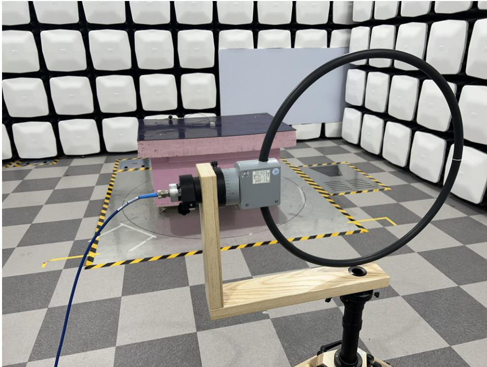
Radiated Test_9 kHz to 30 MHz_Rear
