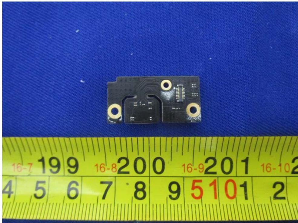
EUT – Link Board2 Bottom View
