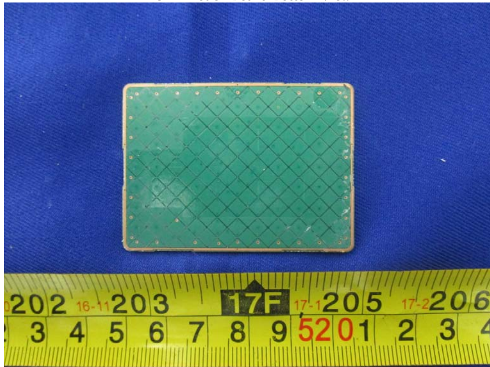
EUT – Touch Board Bottom View
