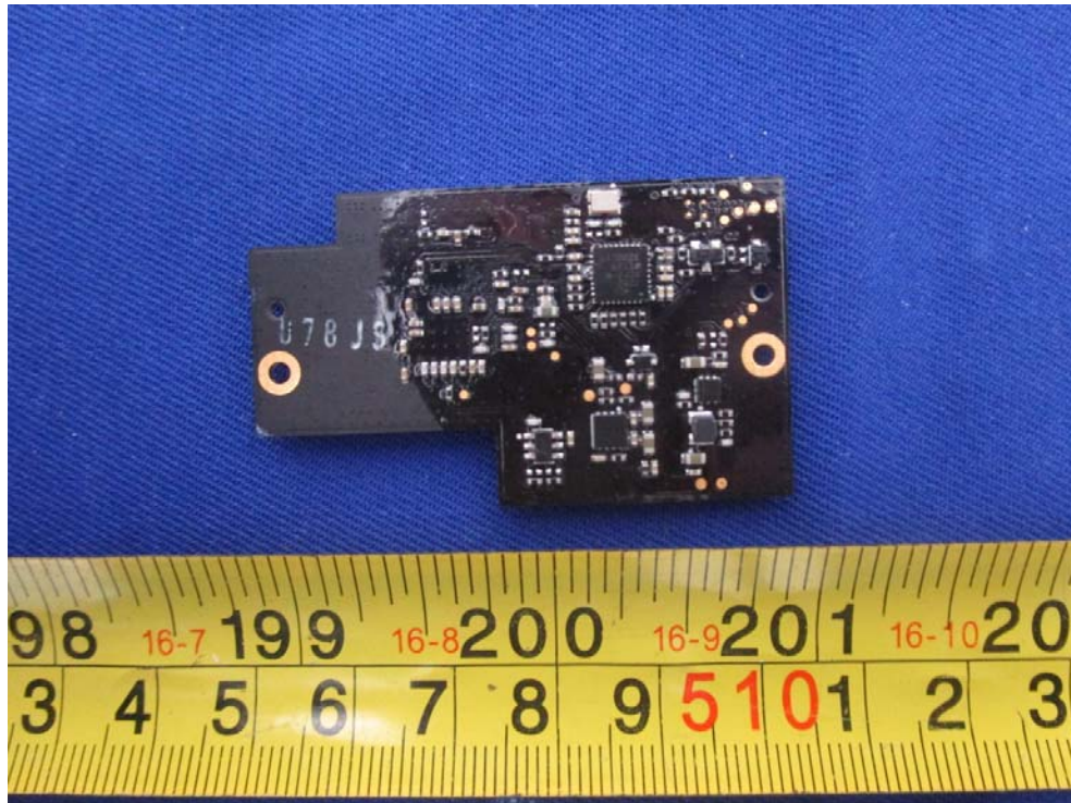
EUT – 5G RF Board Bottom View
