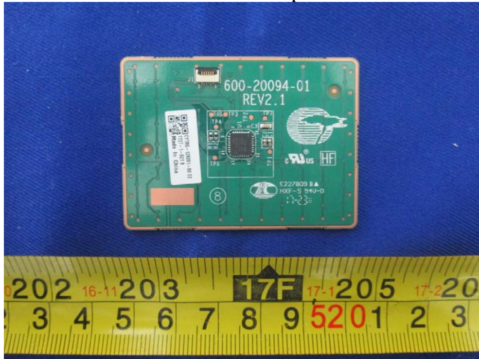
EUT – Touch Board Top View
