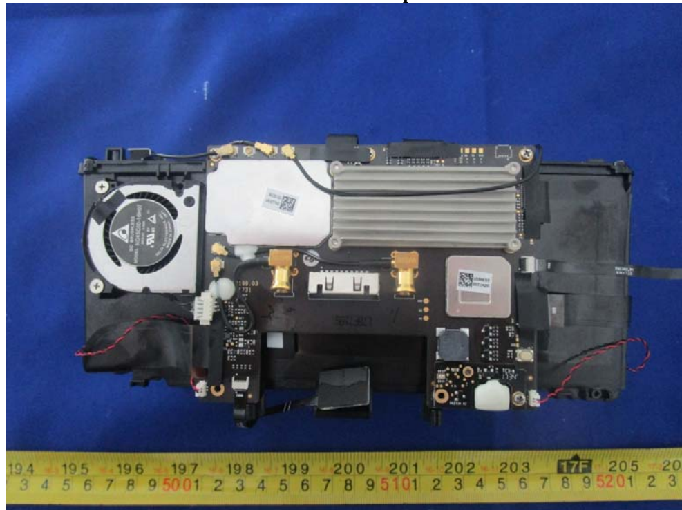
EUT – Main Part Top View
