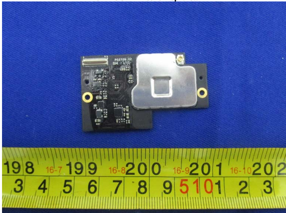
EUT – 5G RF Board Top View
