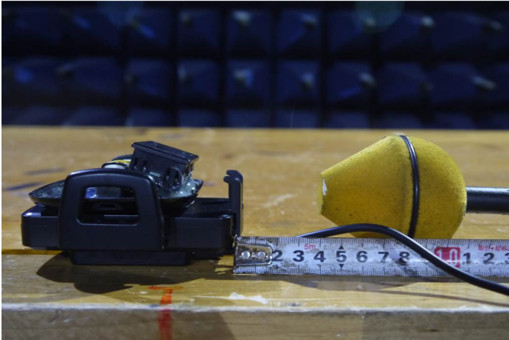
Electric Field and Magnetic Field_4cm
