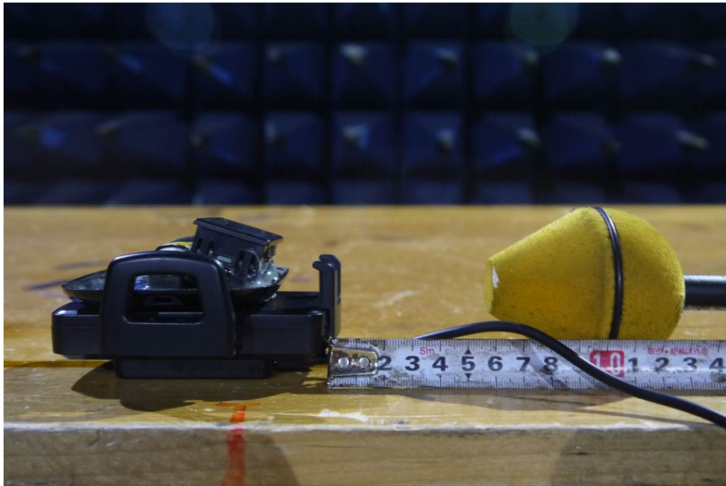
Electric Field and Magnetic Field_6cm
