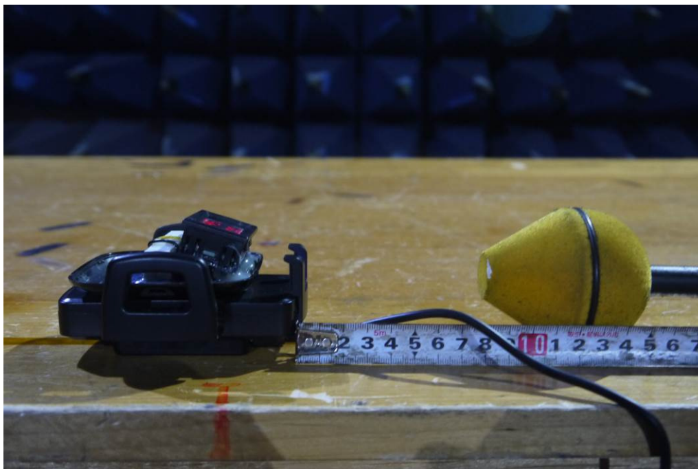
Electric Field and Magnetic Field_8cm
