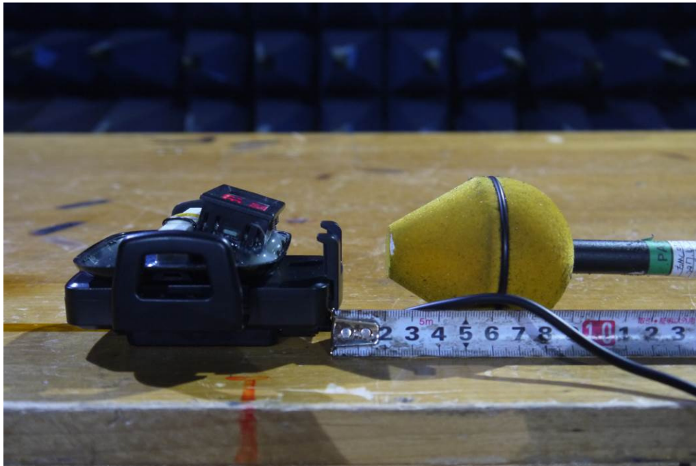
Electric Field and Magnetic Field_2cm
