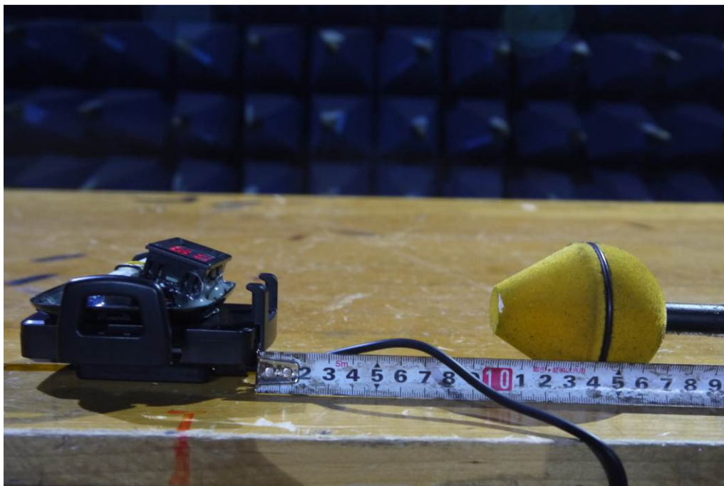
Electric Field and Magnetic Field_10cm
