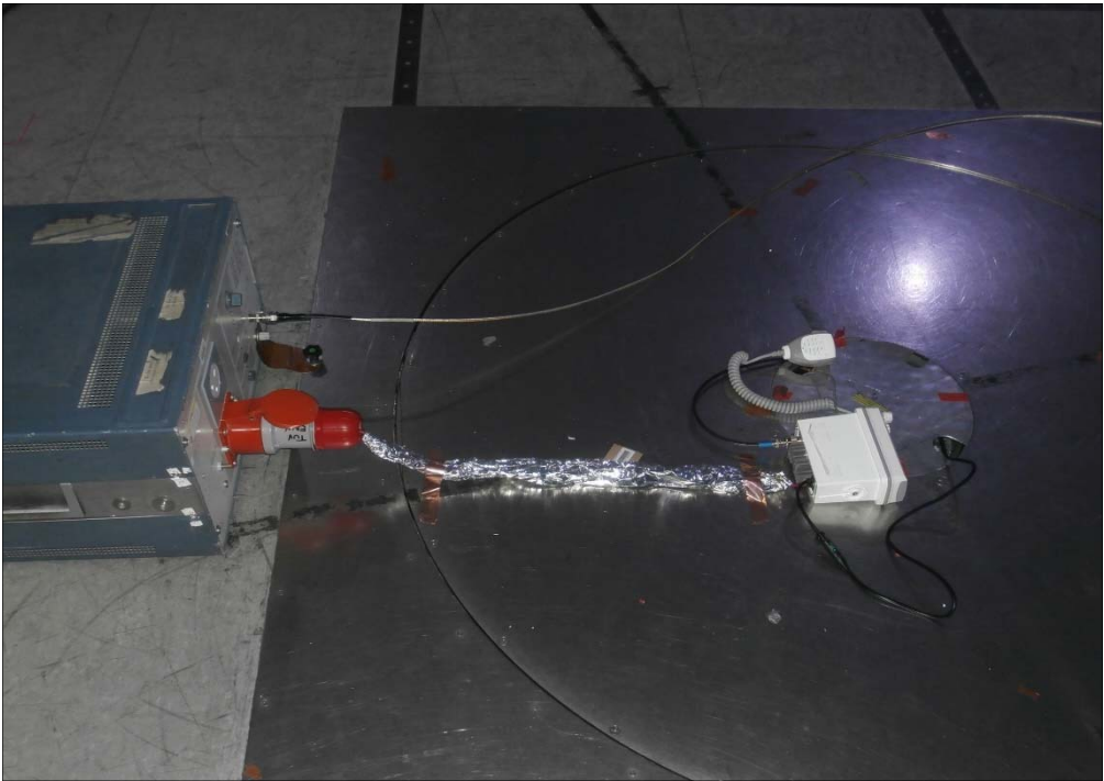
Figure 5 - Test Setup
