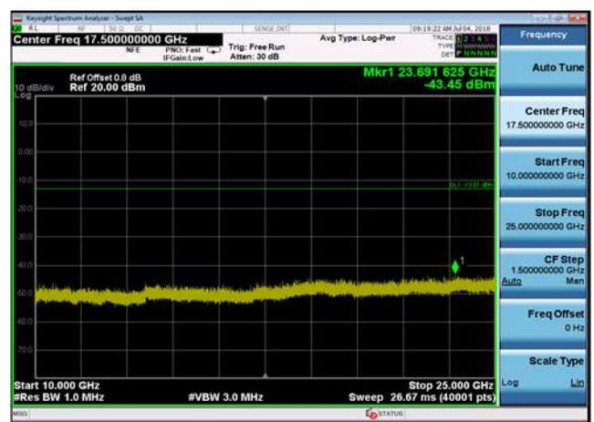
GFSK,2480MHz,DH5,Plot 4,10000MHz~2500 OMHz
