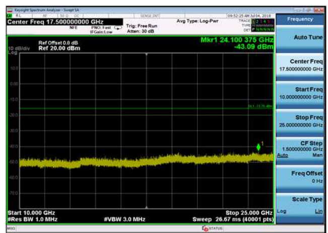
8DPSK,2480MHz,3DH5,Plot 4,10000MHz~25 000MHz
