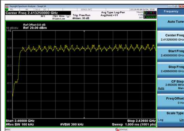
DQPSK,Hopping,2DH5,2400~2426.5MHz
