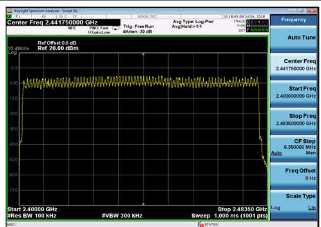
DQPSK,Hopping,2DH5,2400~2483.5MHz
