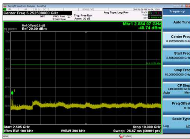
8DPSK,2480MHz,3DH5,Plot 3,2505MHz~100 00MHz
