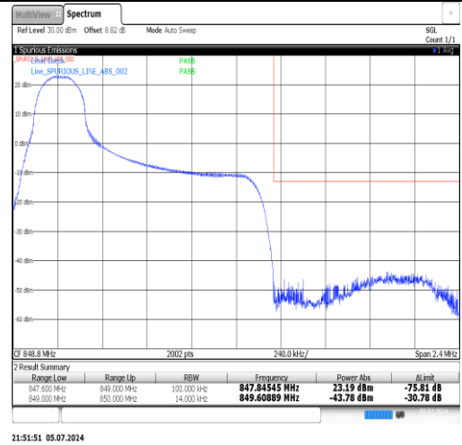
Band5-1.4MHz-16QAM-20643-1RB#5-PASS
