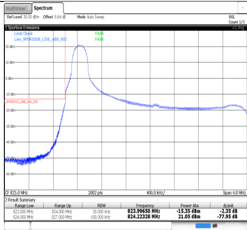
Band5-3MHz-16QAM-20415-1RB#14-PASS
