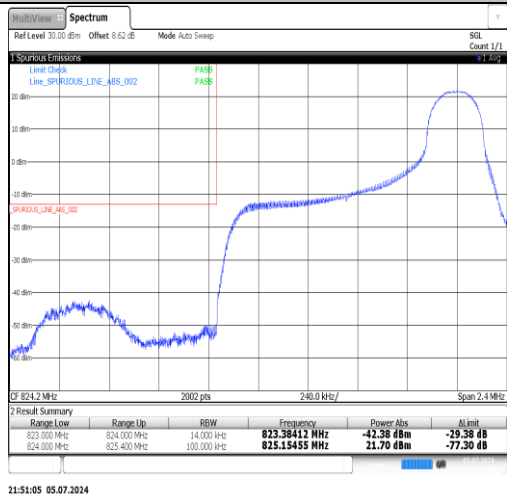
Band5-1.4MHz-QPSK-20643-6RB#0-PASS
