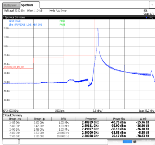
Band7-10MHz-16QAM-20800-1RB#49-PASS
