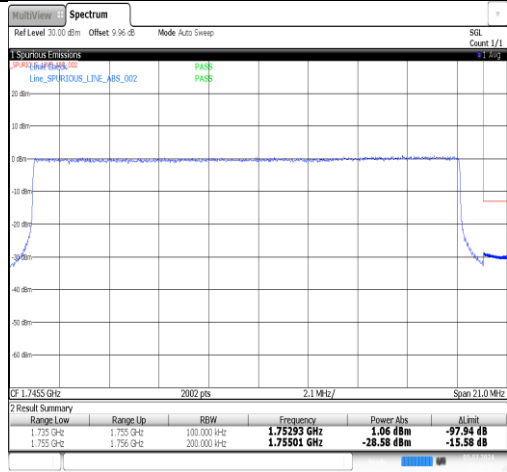
Band4-20MHz-QPSK-20300-100RB#0-PASS
