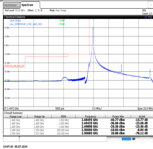
Band7-15MHz-16QAM-20825-1RB#74-PASS
