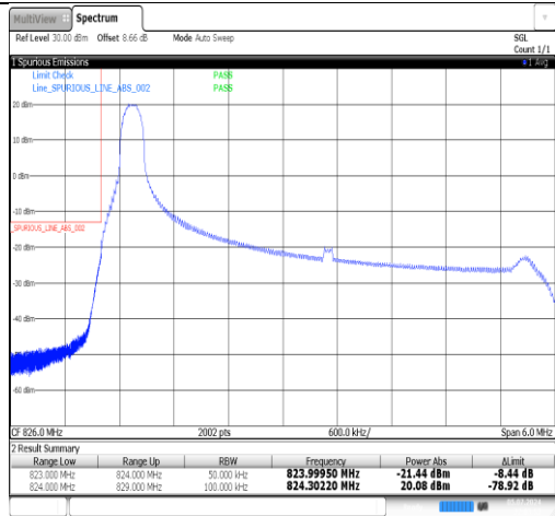
Band5-5MHz-16QAM-20425-1RB#24-PASS
