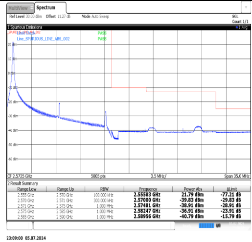
Band7-15MHz-16QAM-21375-1RB#74-PASS
