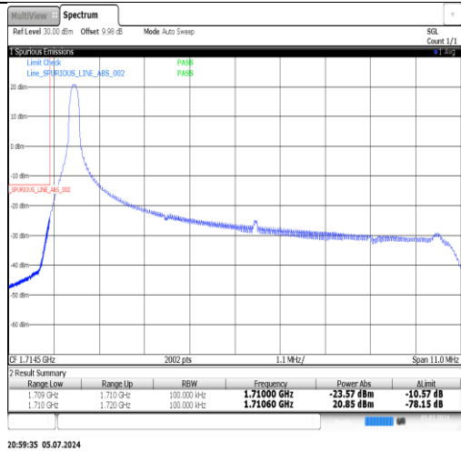
Band4-10MHz-16QAM-20000-1RB#49-PASS
