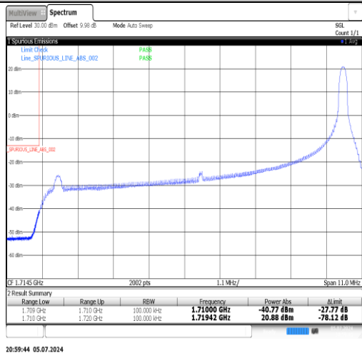
Band4-10MHz-QPSK-20350-50RB#0-PASS
