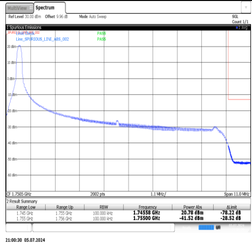
Band4-10MHz-16QAM-20350-1RB#49-PASS
