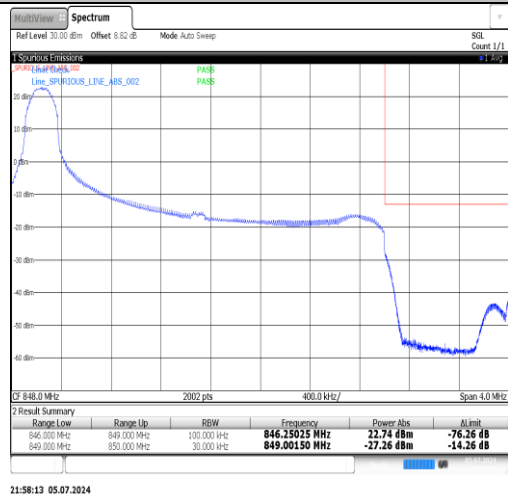
Band5-3MHz-16QAM-20635-1RB#14-PASS
