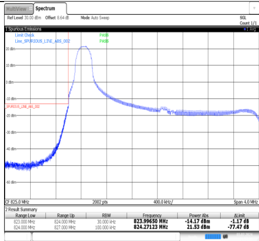
Band5-3MHz-QPSK-20415-1RB#14-PASS
