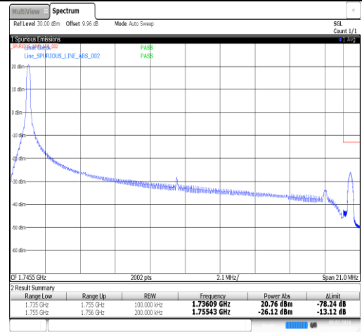
Band4-20MHz-QPSK-20300-1RB#0-PASS
