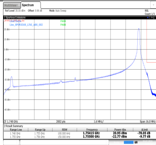
Band4-15MHz-16QAM-20325-1RB#74-PASS
