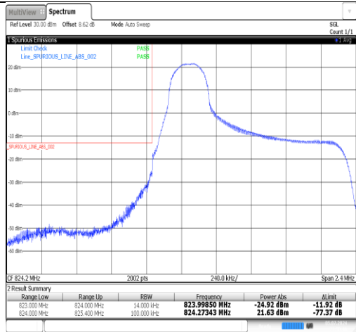
Band5-1.4MHz-QPSK-20407-1RB#5-PASS
