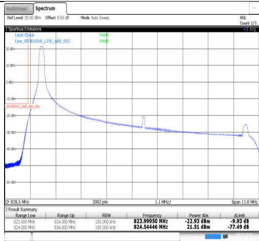
Band5-10MHz-QPSK-20450-1RB#49-PASS
