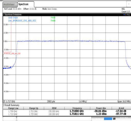
Band4-15MHz-16QAM-20325-1RB#0-PASS
