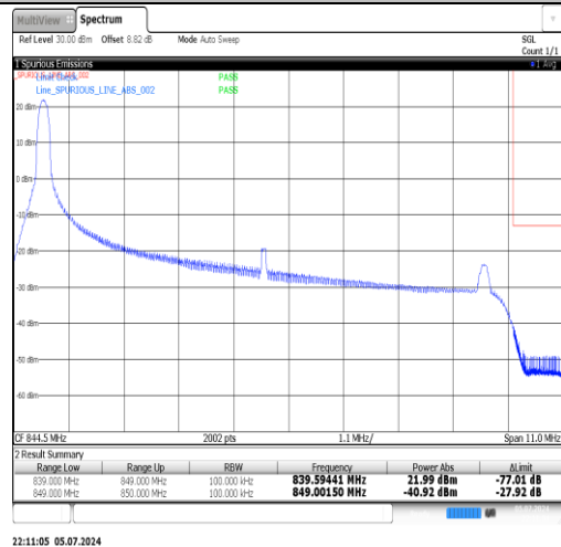
Band5-10MHz-16QAM-20600-1RB#49-PASS
