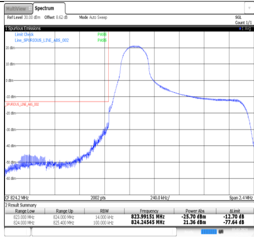
Band5-1.4MHz-16QAM-20407-1RB#5-PASS
