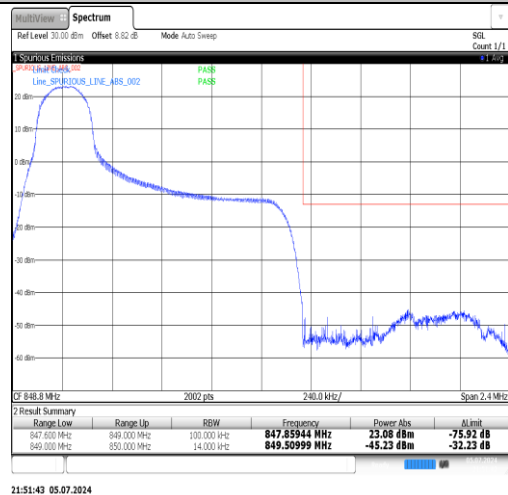
Band5-1.4MHz-QPSK-20643-1RB#5-PASS
