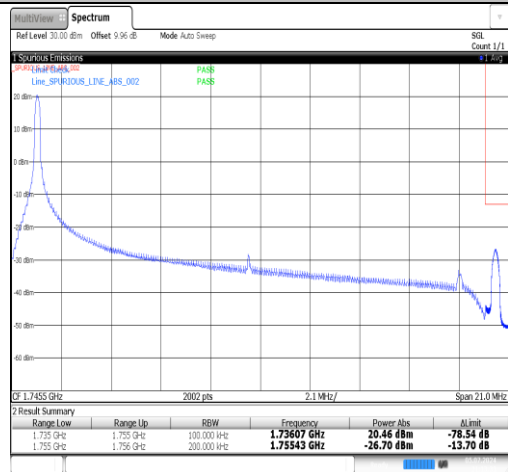
Band4-20MHz-16QAM-20300-1RB#99-PASS
