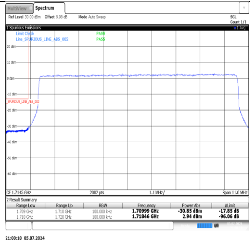
Band4-10MHz-16QAM-20350-1RB#0-PASS
