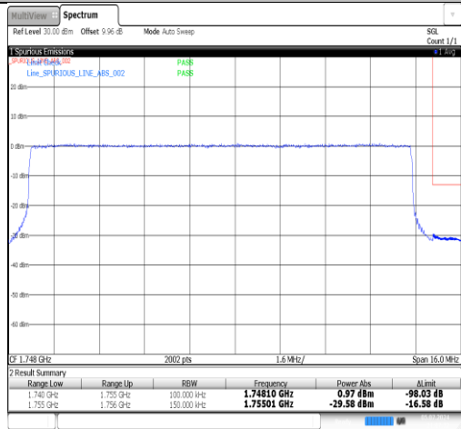
Band4-15MHz-16QAM-20325-75RB#0-PASS
