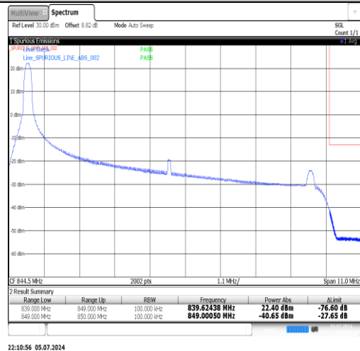
Band5-10MHz-QPSK-20600-1RB#49-PASS
