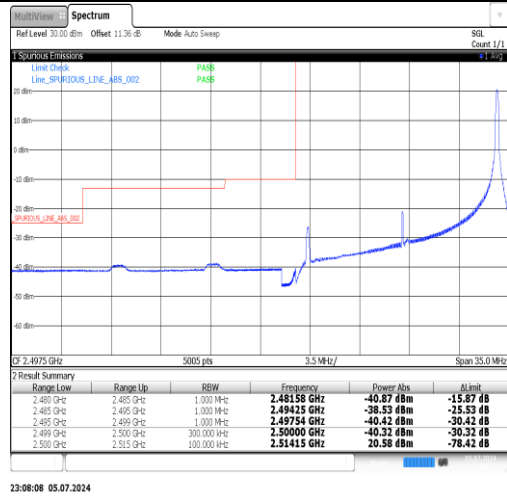
Band7-15MHz-16QAM-21375-75RB#0-PASS
