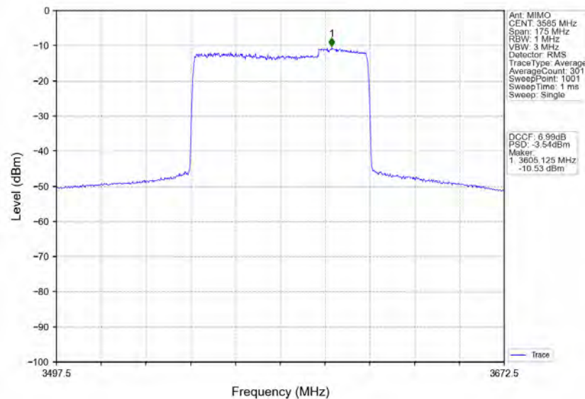
n78d_30kHz_MIMO_NTNV_70MHz_CP-OFDM_QPSK_3585MHz_Inner_Full
