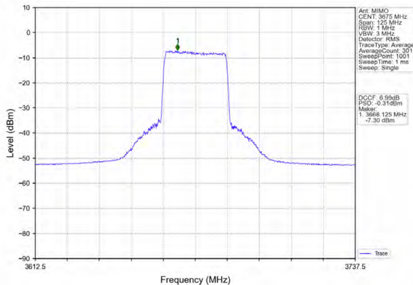
n78d_30kHz_MIMO_NTNV_50MHz_CP-OFDM_QPSK_3675MHz_Inner_Full
