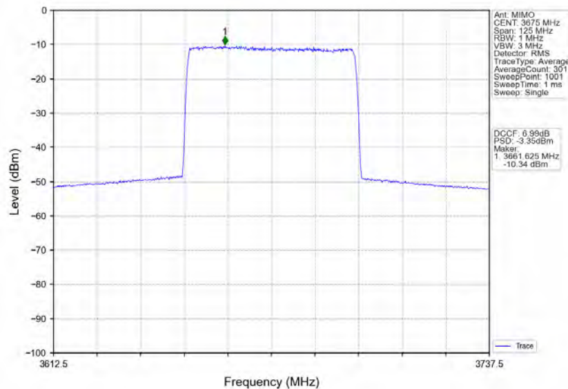
n78d_30kHz_MIMO_NTNV_50MHz_CP-OFDM_256_QAM_3675MHz_Inner_Full
