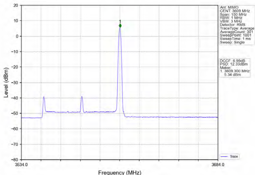
n78d_30kHz_MIMO_NTNV_60MHz_CP-OFDM 64 QAM_3580.02MHz_Edge_1RB_Right
