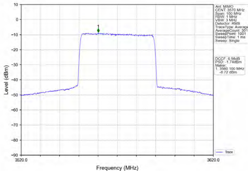
n78d_30kHz_MIMO_NTNV_40MHz_CP-OFDM_QPSK_3570MHz_Inner_Full
