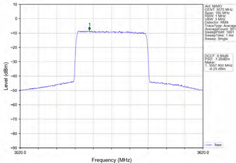
n78d_30kHz_MIMO_NTNV_40MHz_CP-OFDM_256_QAM_3570MHz_Inner_Full
