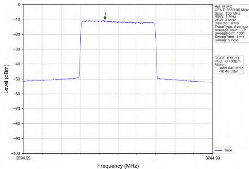
n78d_30kHz_MIMO_NTNV_60MHz_CP-OFDM_16_QAM_3669.99MHz_Inner_Full
