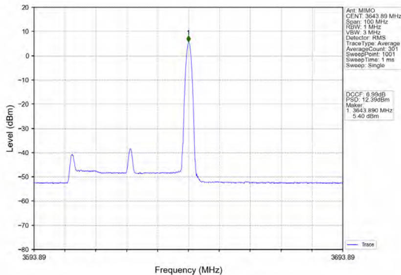
n78d_30kHz_MIMO_NTNV_40MHz_CP-OFDM_QPSK_3624.99MHz_Edge_1RB_Right
