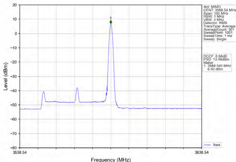
n78d_30kHz_MIMO_NTNV_40MHz_CP-OFDM QPSK_3570MHz_Inner_1RB_Right
