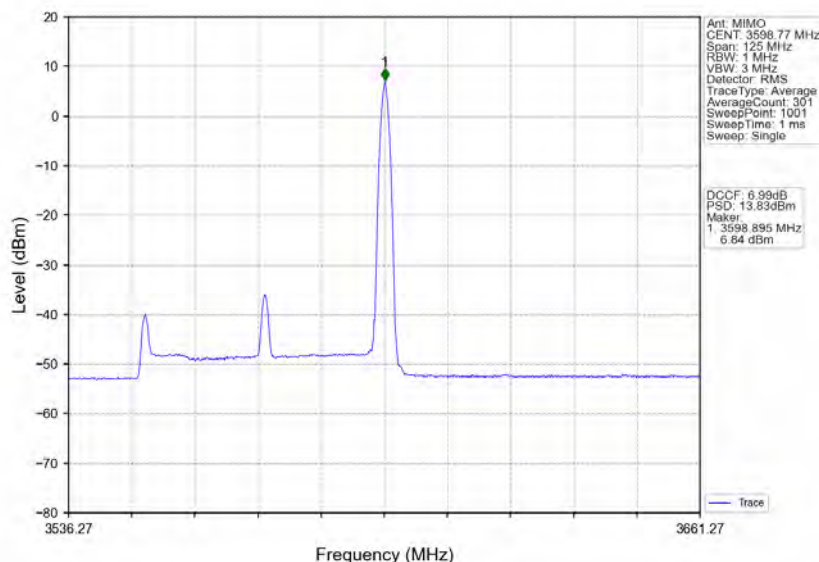
n78d_30kHz_MIMO_NTNV_50MHz_CP-OFDM_256_QAM_3575.01MHz_Edge_1RB_Right
