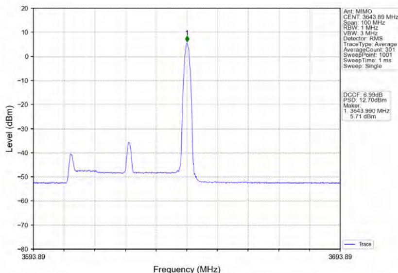
n78d_30kHz_MIMO_NTNV_40MHz_CP-OFDM_256_QAM_3624.99MHz_Edge_1RB_Right
