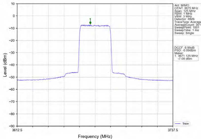
n78d_30kHz_MIMO_NTNV_50MHz_CP-OFDM_256_QAM_3675MHz_Inner_Full
