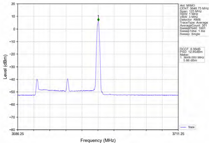
n78d_30kHz_MIMO_NTNV_50MHz_CP-OFDM_QPSK_3624.99MHz_Edge_1RB_Right
