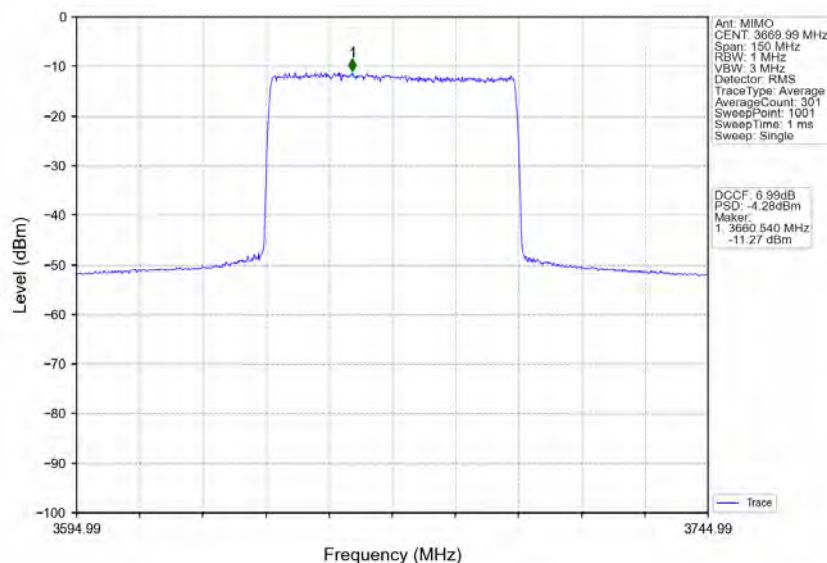
n78d_30kHz_MIMO_NTNV_60MHz_CP-OFDM_64_QAM_3669.99MHz_Inner_Full
