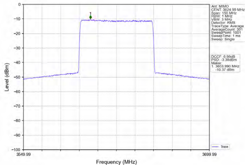
n78d_30kHz_MIMO_NTNV_60MHz_CP-OFDM_256_QAM_3624.99MHz_Inner_Full
