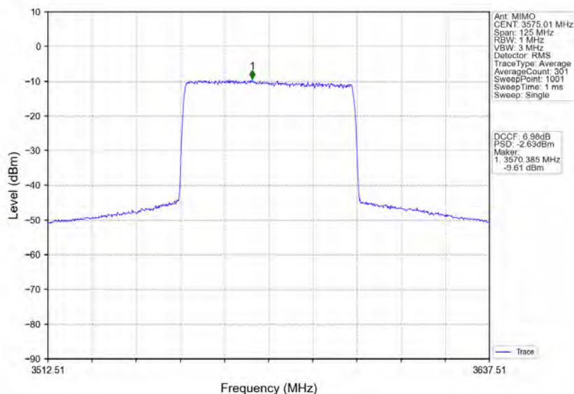
n78d_30kHz_MIMO_NTNV_50MHz_CP-OFDM 64 QAM_3575.01MHz_Inner_Full
