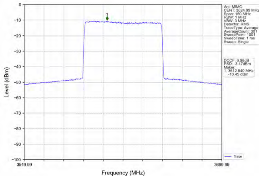
n78d_30kHz_MIMO_NTNV_60MHz_CP-OFDM QPSK_3624.99MHz_Inner_Full
