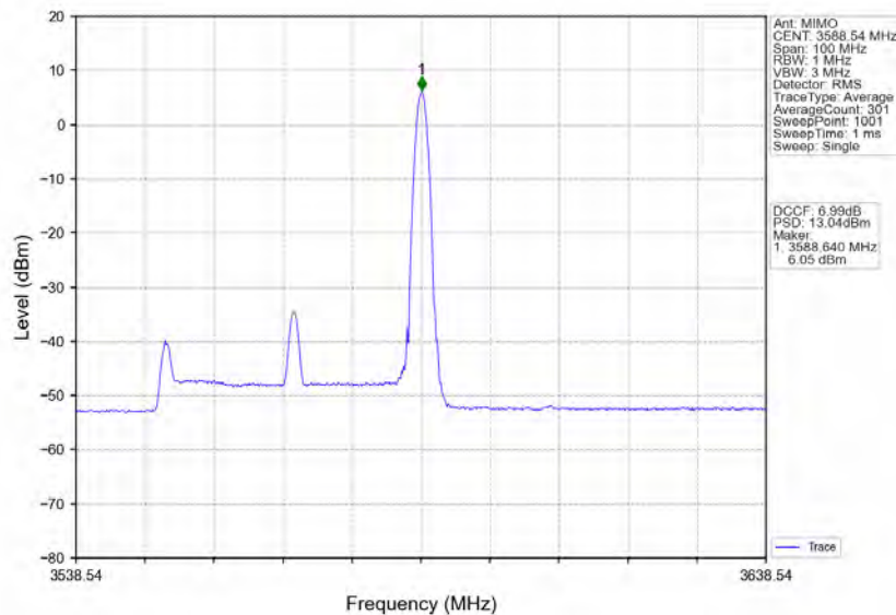
n78d_30kHz_MIMO_NTNV_40MHz_CP-OFDM_256_QAM_3570MHz_Inner_1RB_Right
