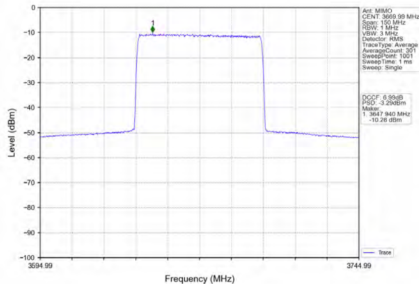
n78d_30kHz_MIMO_NTNV_60MHz_CP-OFDM QPSK_3669.99MHz_Inner_Full
