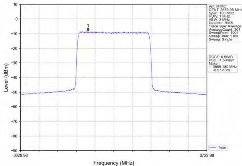
n78d_30kHz_MIMO_NTNV_40MHz_CP-OFDM_16_QAM_3679.98MHz_Inner_Full
