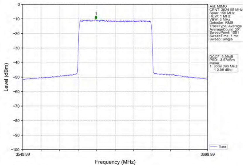
n78d_30kHz_MIMO_NTNV_60MHz_CP-OFDM_16_QAM_3624.99MHz_Inner_Full
