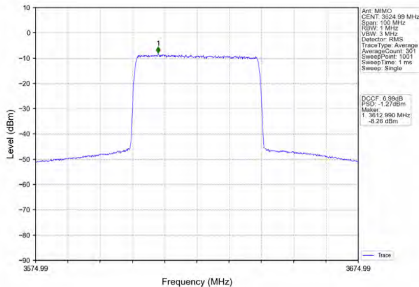
n78d_30kHz_MIMO_NTNV_40MHz_CP-OFDM_QPSK_3624.99MHz_Inner_Full
