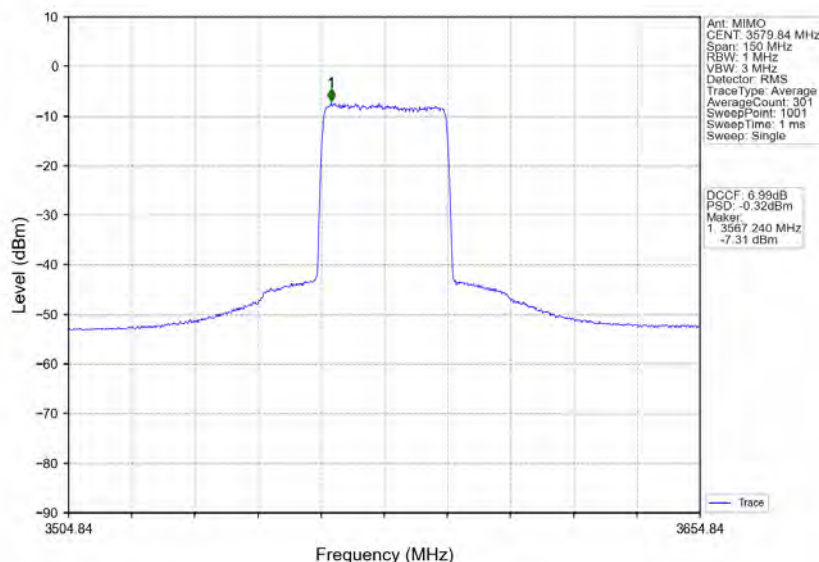
n78d_30kHz_MIMO_NTNV_60MHz_CP-OFDM_256_QAM_3580.02MHz_Inner_Full
