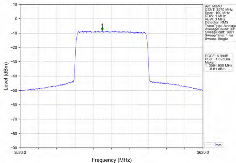
n78d_30kHz_MIMO_NTNV_40MHz_CP-OFDM_16_QAM_3570MHz_Inner_Full
