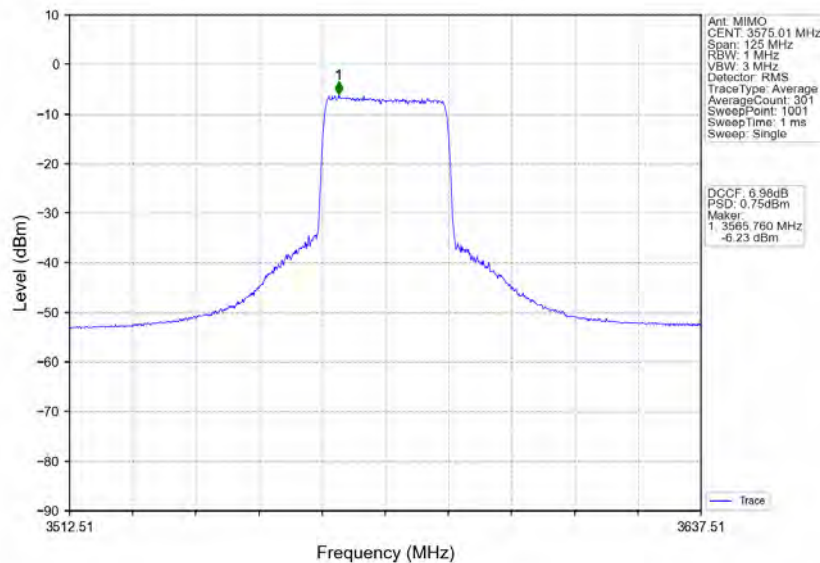
n78d_30kHz_MIMO_NTNV_50MHz_CP-OFDM_16_QAM_3575.01MHz_Inner_Full
