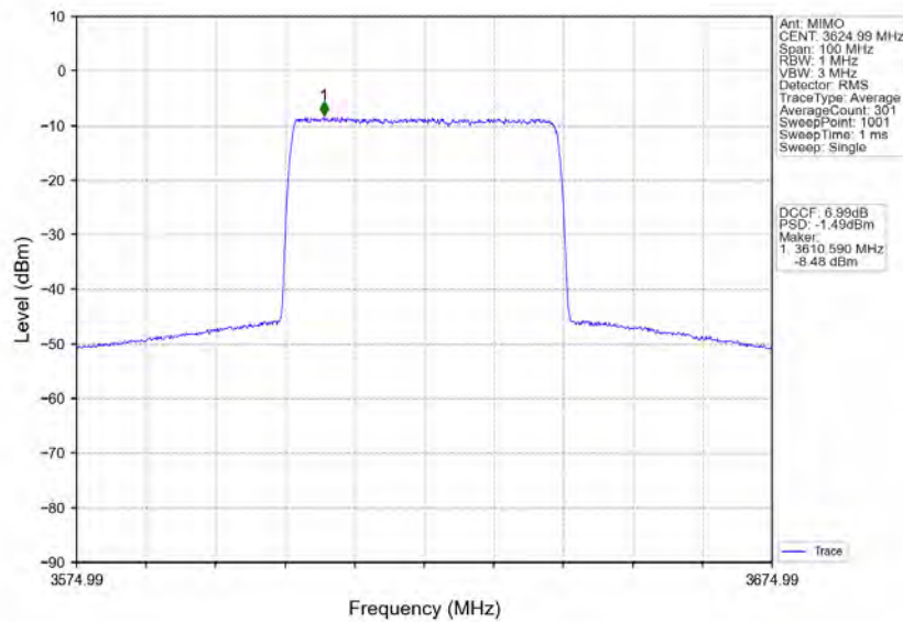
n78d_30kHz_MIMO_NTNV_40MHz_CP-OFDM_256_QAM_3624.99MHz_Inner_Full
