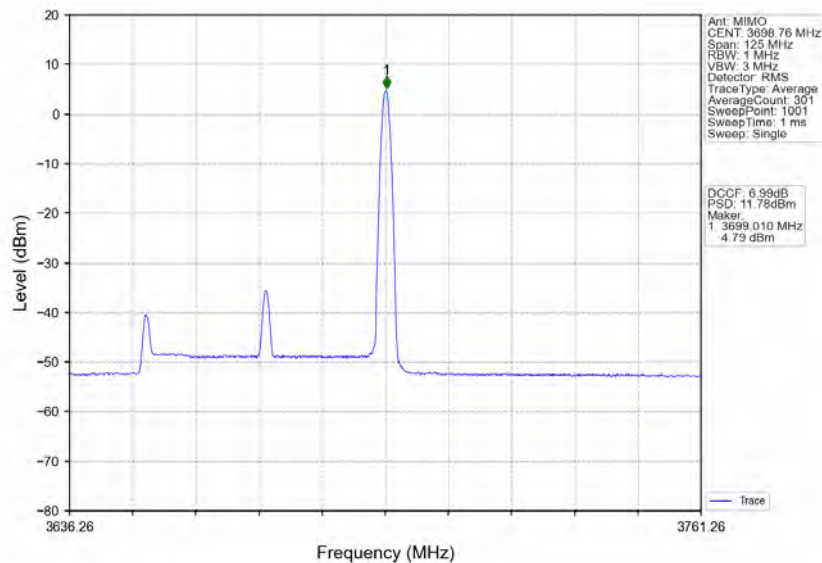
n78d_30kHz_MIMO_NTNV_50MHz_CP-OFDM_256_QAM_3675MHz_Edge_1RB_Right
