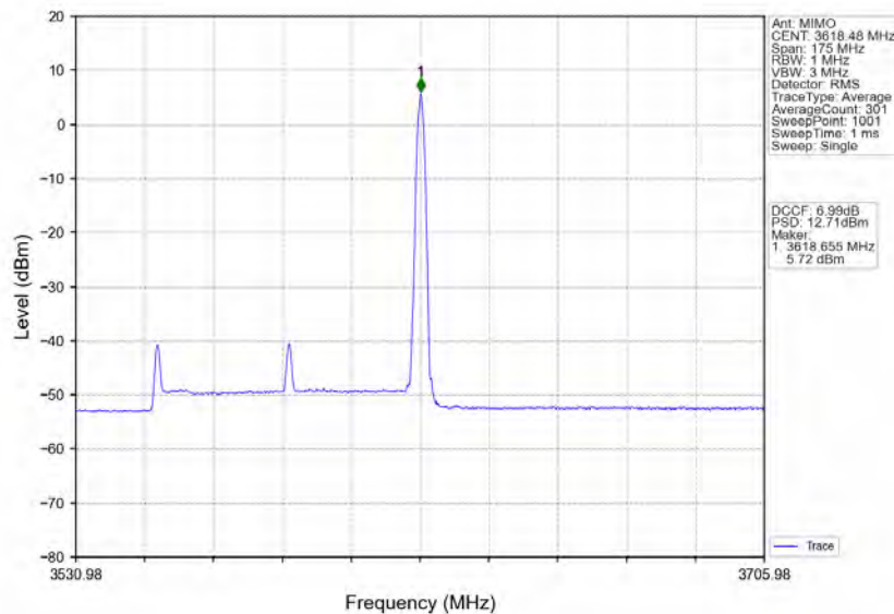
n78d_30kHz_MIMO_NTNV_70MHz_CP-OFDM QPSK_3585MHz_Inner_1RB_Right
