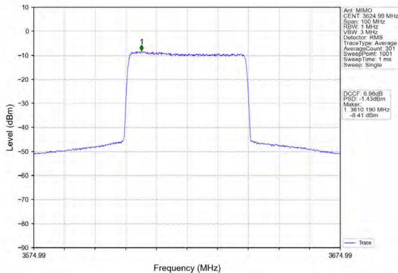
n78d_30kHz_MIMO_NTNV_40MHz_CP-OFDM_16_QAM_3624.99MHz_Inner_Full
