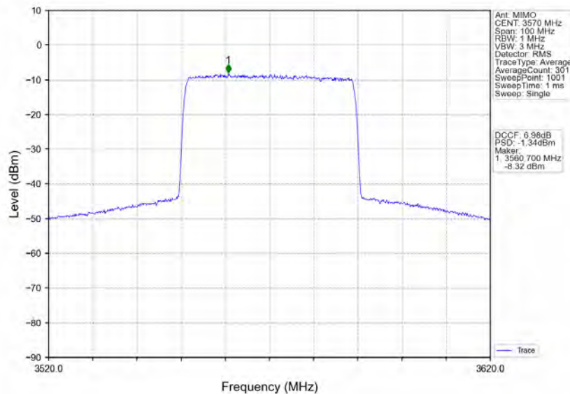
n78d_30kHz_MIMO_NTNV_40MHz_CP-OFDM_64_QAM_3570MHz_Inner_Full
