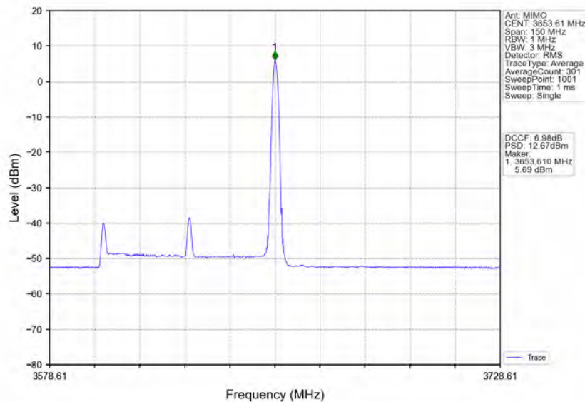
n78d_30kHz_MIMO_NTNV_60MHz_CP-OFDM 16 QAM_3624.99MHz_Inner_1RB_Right
