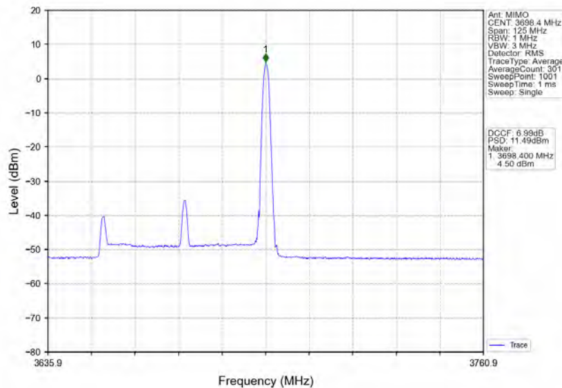
n78d_30kHz_MIMO_NTNV_50MHz_CP-OFDM_256_QAM_3675MHz_Inner_1RB_Right
