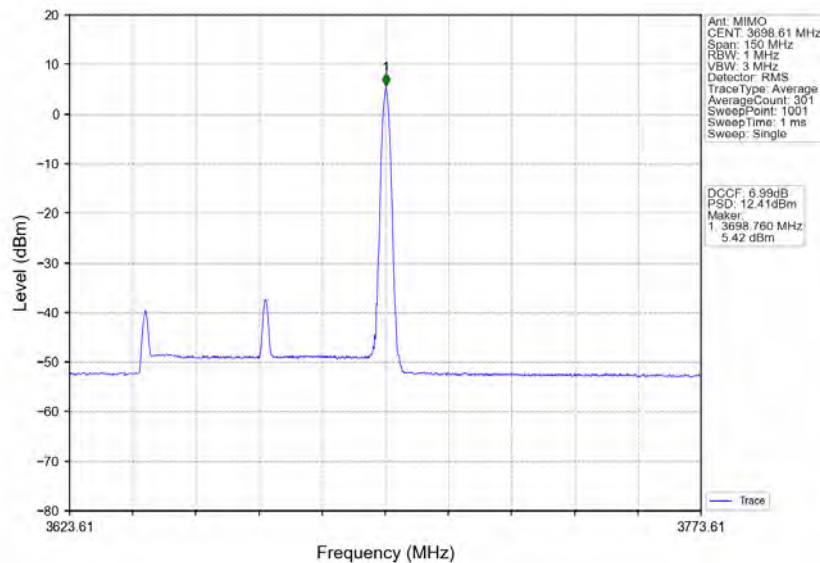
n78d_30kHz_MIMO_NTNV_60MHz_CP-OFDM 16 QAM_3669.99MHz_Inner_1RB_Right
