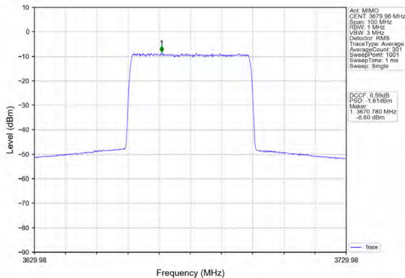
n78d_30kHz_MIMO_NTNV_40MHz_CP-OFDM_256_QAM_3679.98MHz_Inner_Full
