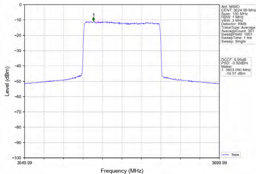
n78d_30kHz_MIMO_NTNV_60MHz_CP-OFDM_64_QAM_3624.99MHz_Inner_Full
