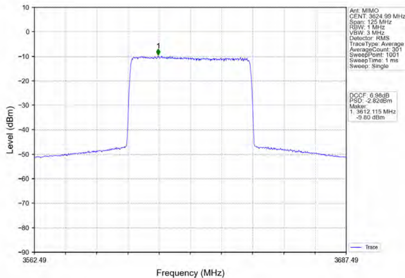
n78d_30kHz_MIMO_NTNV_50MHz_CP-OFDM_QPSK_3624.99MHz_Inner_Full
