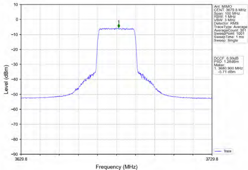
n78d_30kHz_MIMO_NTNV_40MHz_CP-OFDM_QPSK_3679.98MHz_Inner_Full
