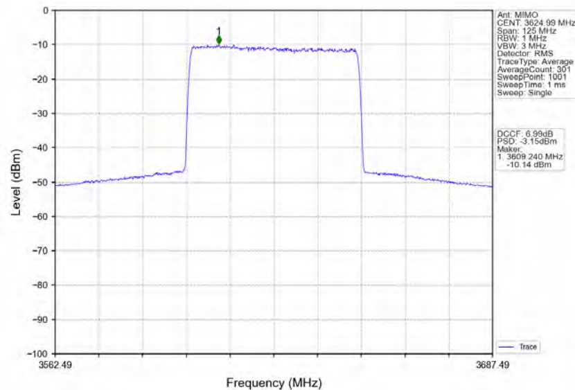
n78d_30kHz_MIMO_NTNV_50MHz_CP-OFDM_256_QAM_3624.99MHz_Inner_Full
