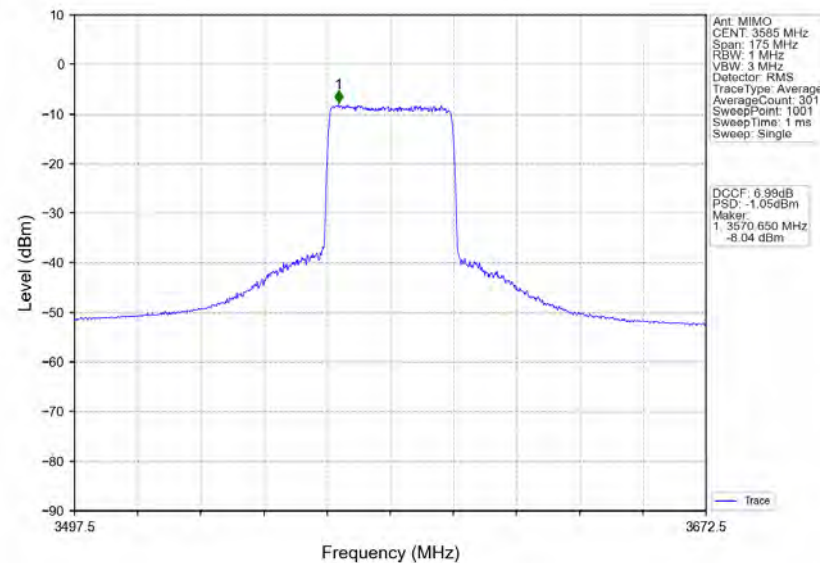
n78d_30kHz_MIMO_NTNV_70MHz_CP-OFDM_QPSK_3585MHz_Inner_Full
