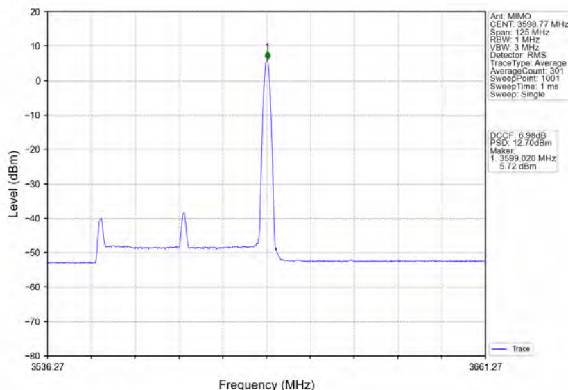
n78d_30kHz_MIMO_NTNV_50MHz_CP-OFDM 16 QAM_3575.01MHz_Edge_1RB_Right
