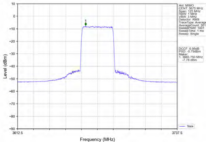
n78d_30kHz_MIMO_NTNV_50MHz_CP-OFDM_64_QAM_3675MHz_Inner_Full
