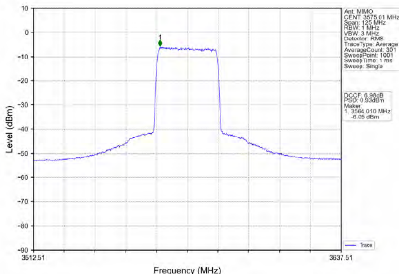
n78d_30kHz_MIMO_NTNV_50MHz_CP-OFDM_256_QAM_3575.01MHz_Inner_Full
