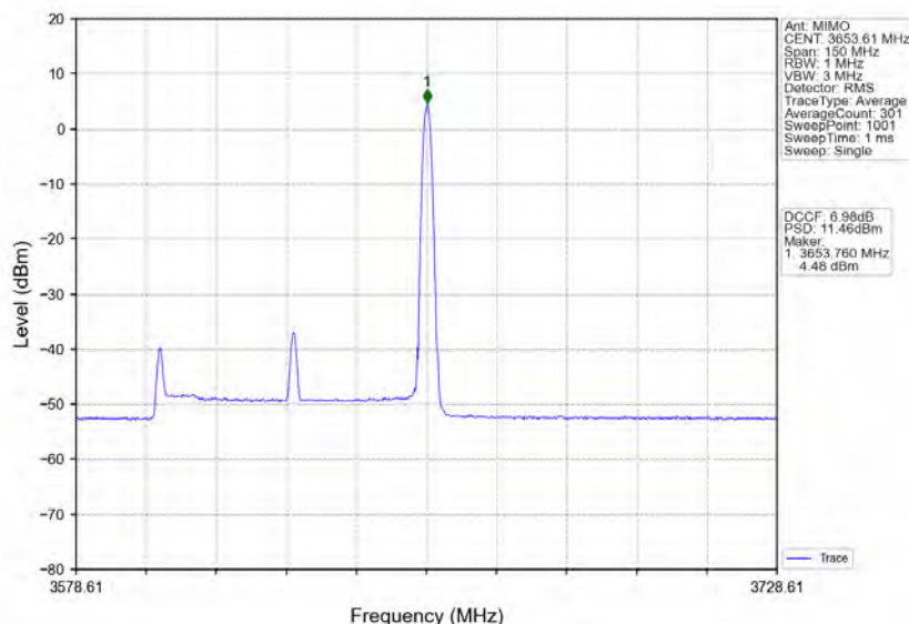
n78d_30kHz_MIMO_NTNV_60MHz_CP-OFDM_256_QAM_3624.99MHz_Inner_1RB_Right
