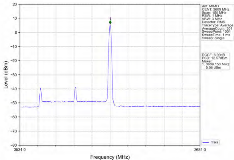
n78d_30kHz_MIMO_NTNV_60MHz_CP-OFDM 16 QAM_3580.02MHz_Edge_1RB_Right
