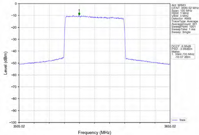
n78d_30kHz_MIMO_NTNV_60MHz_CP-OFDM 64 QAM_3580.02MHz_Inner_Full
