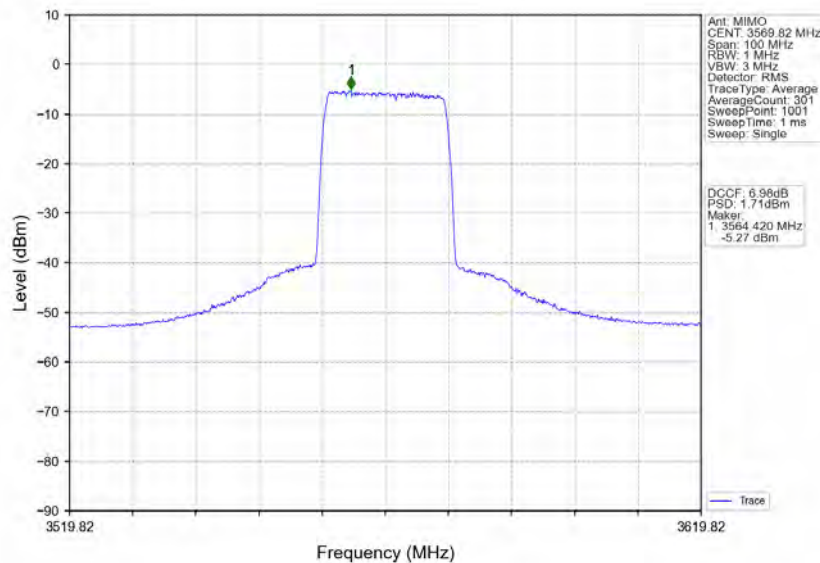
n78d_30kHz_MIMO_NTNV_40MHz_CP-OFDM_256_QAM_3570MHz_Inner_Full
