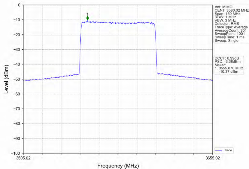
n78d_30kHz_MIMO_NTNV_60MHz_CP-OFDM_16_QAM_3580.02MHz_Inner_Full
