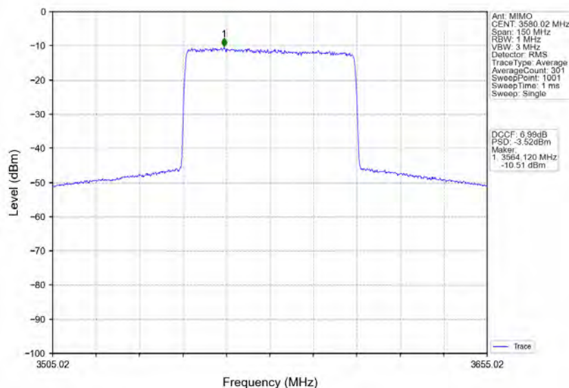
n78d_30kHz_MIMO_NTNV_60MHz_CP-OFDM_256_QAM_3580.02MHz_Inner_Full
