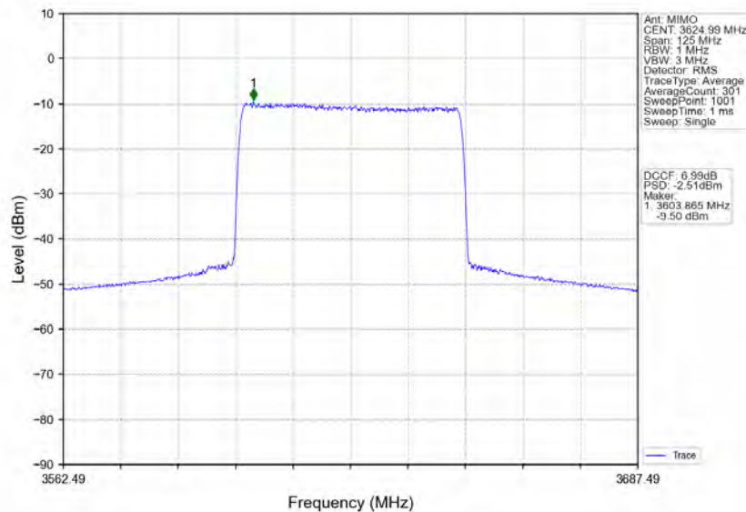
n78d_30kHz_MIMO_NTNV_50MHz_CP-OFDM 64 QAM_3624.99MHz_Inner_Full
