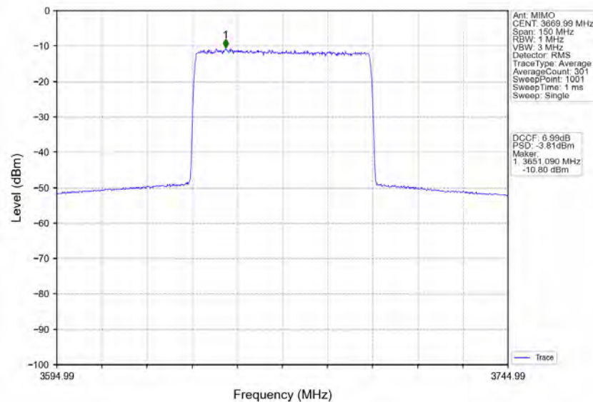
n78d_30kHz_MIMO_NTNV_60MHz_CP-OFDM_256_QAM_3669.99MHz_Inner_Full
