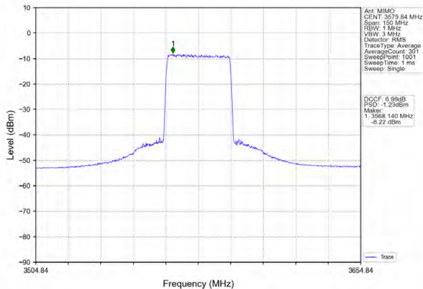
n78d_30kHz_MIMO_NTNV_60MHz_CP-OFDM 64 QAM_3580.02MHz_Inner_Full
