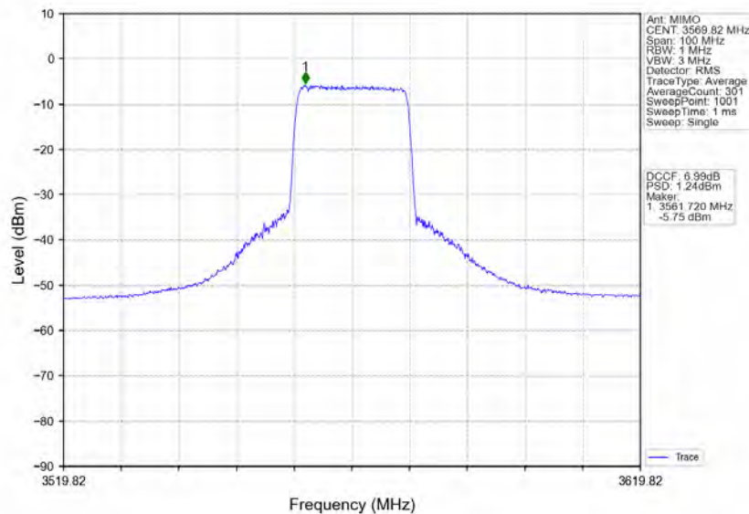
n78d_30kHz_MIMO_NTNV_40MHz_CP-OFDM_QPSK_3570MHz_Inner_Full
