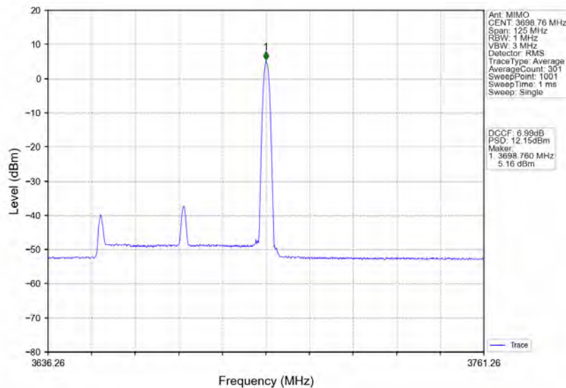
n78d_30kHz_MIMO_NTNV_50MHz_CP-OFDM QPSK_3675MHz_Edge_1RB_Right
