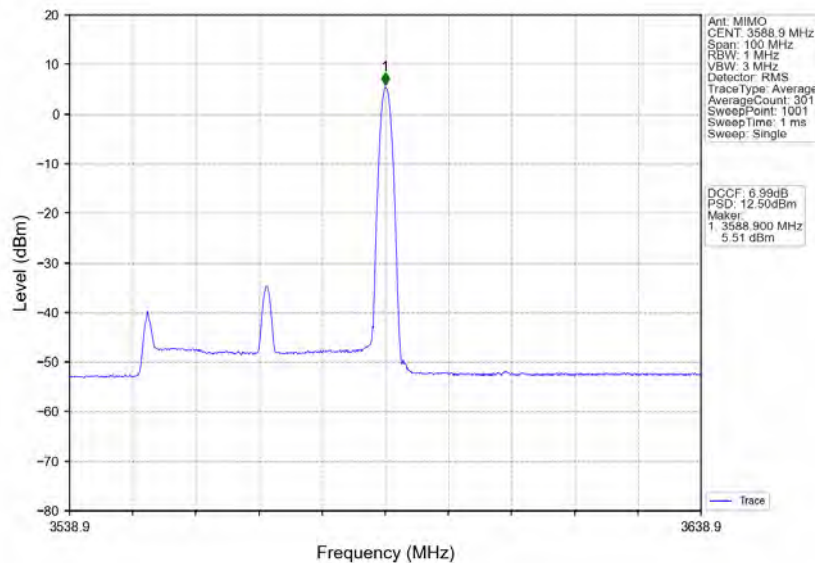
n78d_30kHz_MIMO_NTNV_40MHz_CP-OFDM_256_QAM_3570MHz_Edge_1RB_Right
