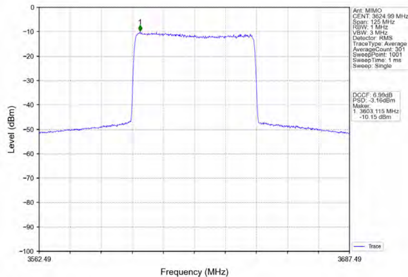
n78d_30kHz_MIMO_NTNV_50MHz_CP-OFDM_16_QAM_3624.99MHz_Inner_Full
