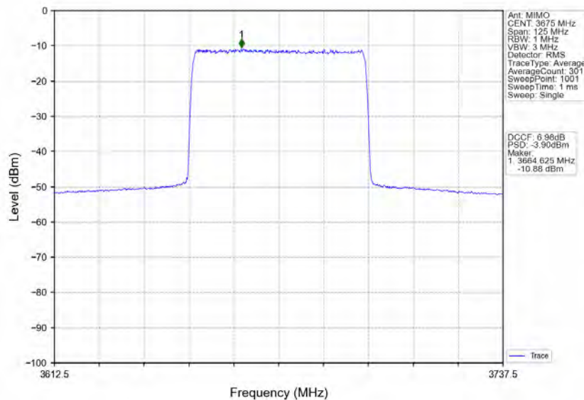
n78d_30kHz_MIMO_NTNV_50MHz_CP-OFDM_QPSK_3675MHz_Inner_Full
