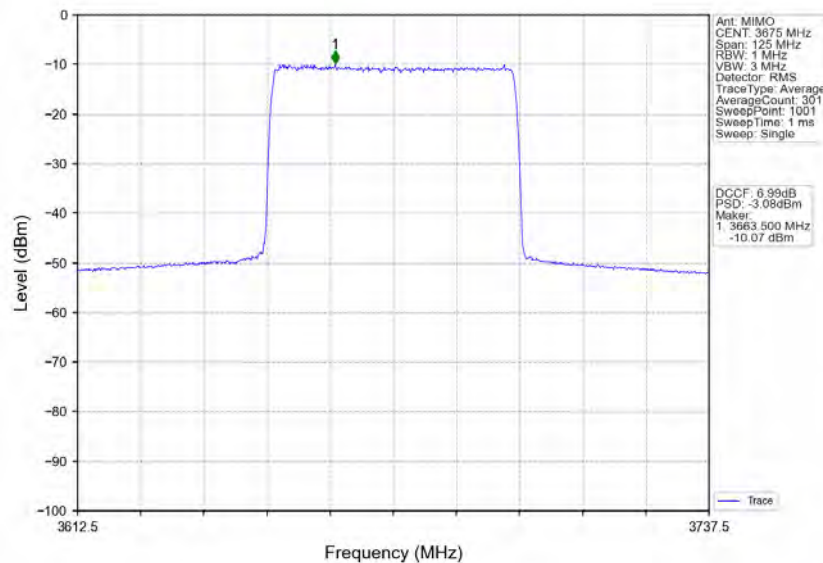
n78d_30kHz_MIMO_NTNV_50MHz_CP-OFDM_16_QAM_3675MHz_Inner_Full
