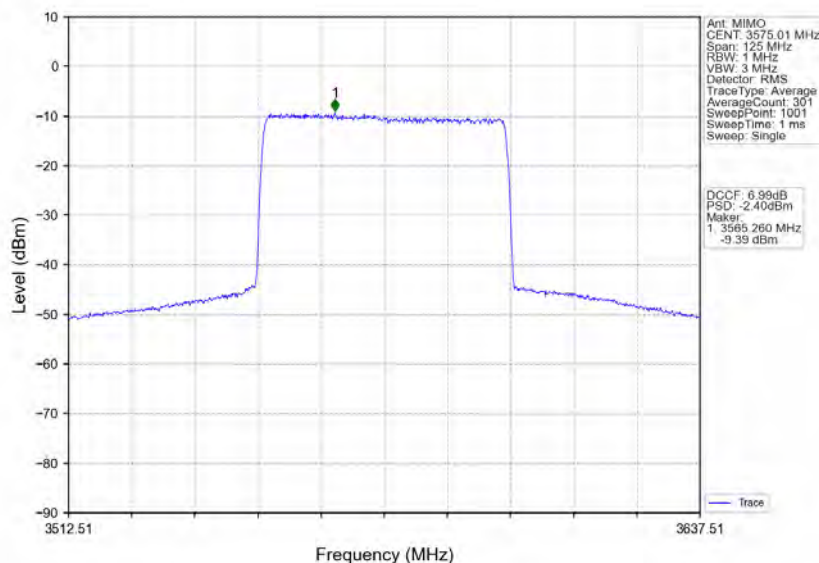
n78d_30kHz_MIMO_NTNV_50MHz_CP-OFDM_QPSK_3575.01MHz_Inner_Full
