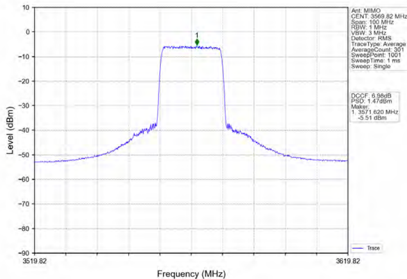
n78d_30kHz_MIMO_NTNV_40MHz_CP-OFDM_16_QAM_3570MHz_Inner_Full
