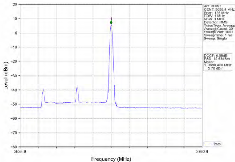
n78d_30kHz_MIMO_NTNV_50MHz_CP-OFDM 64 QAM_3675MHz_Inner_1RB_Right
