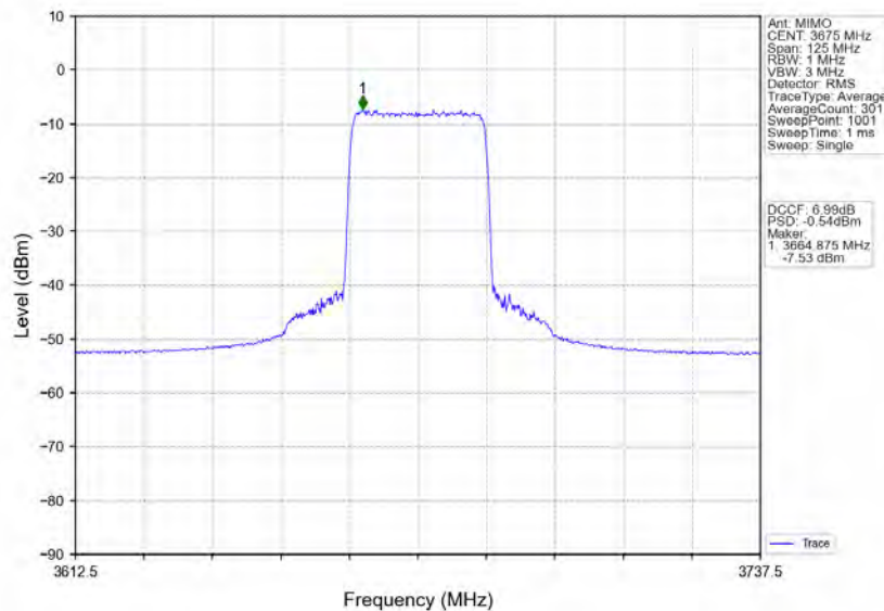
n78d_30kHz_MIMO_NTNV_50MHz_CP-OFDM_16_QAM_3675MHz_Inner_Full
