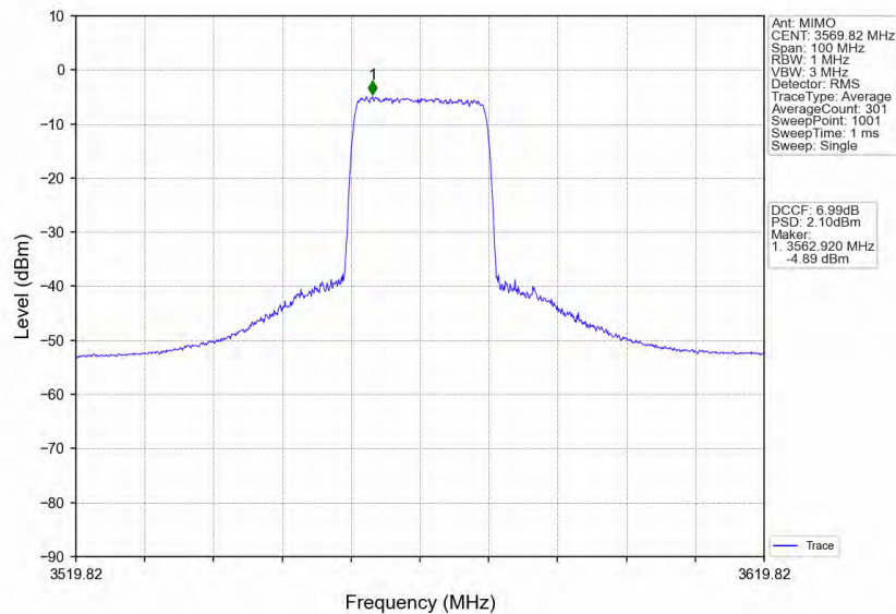
n78d_30kHz_MIMO_NTNV_40MHz_CP-OFDM_64_QAM_3570MHz_Inner_Full
