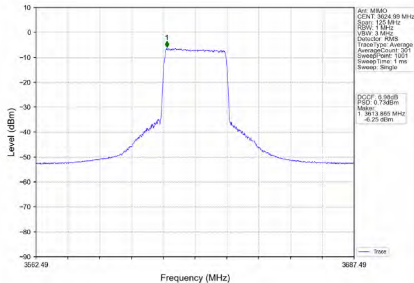
n78d_30kHz_MIMO_NTNV_50MHz_CP-OFDM_16_QAM_3624.99MHz_Inner_Full
