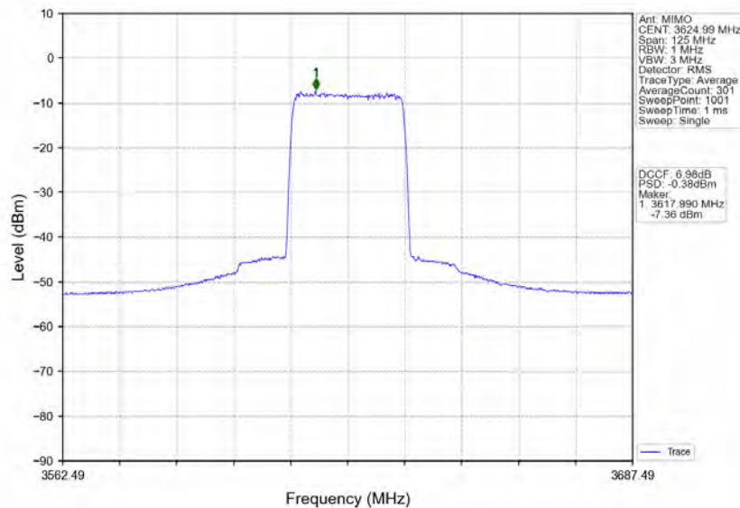
n78d_30kHz_MIMO_NTNV_50MHz_CP-OFDM_256_QAM_3624.99MHz_Inner_Full
