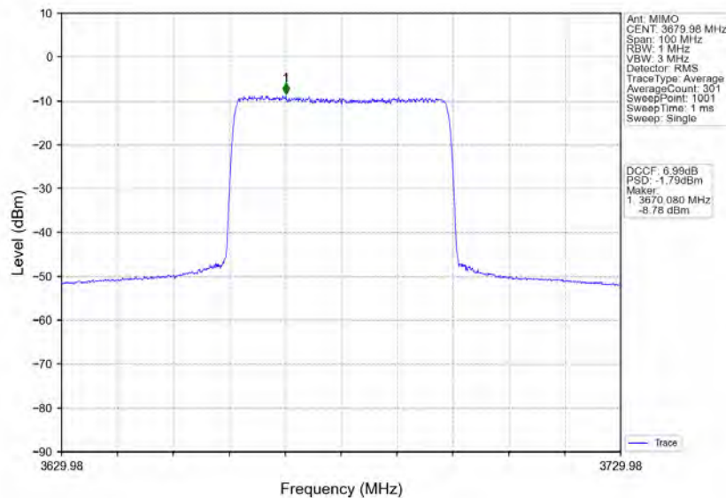
n78d_30kHz_MIMO_NTNV_40MHz_CP-OFDM 64 QAM_3679.98MHz_Inner_Full
