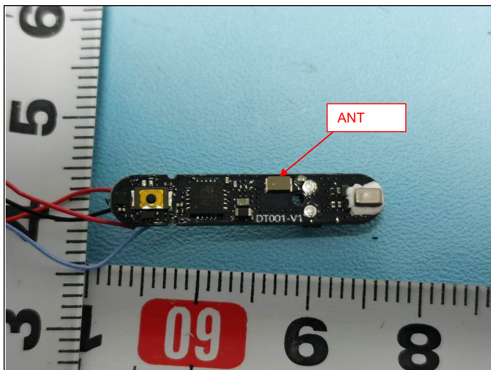
Right earphone
