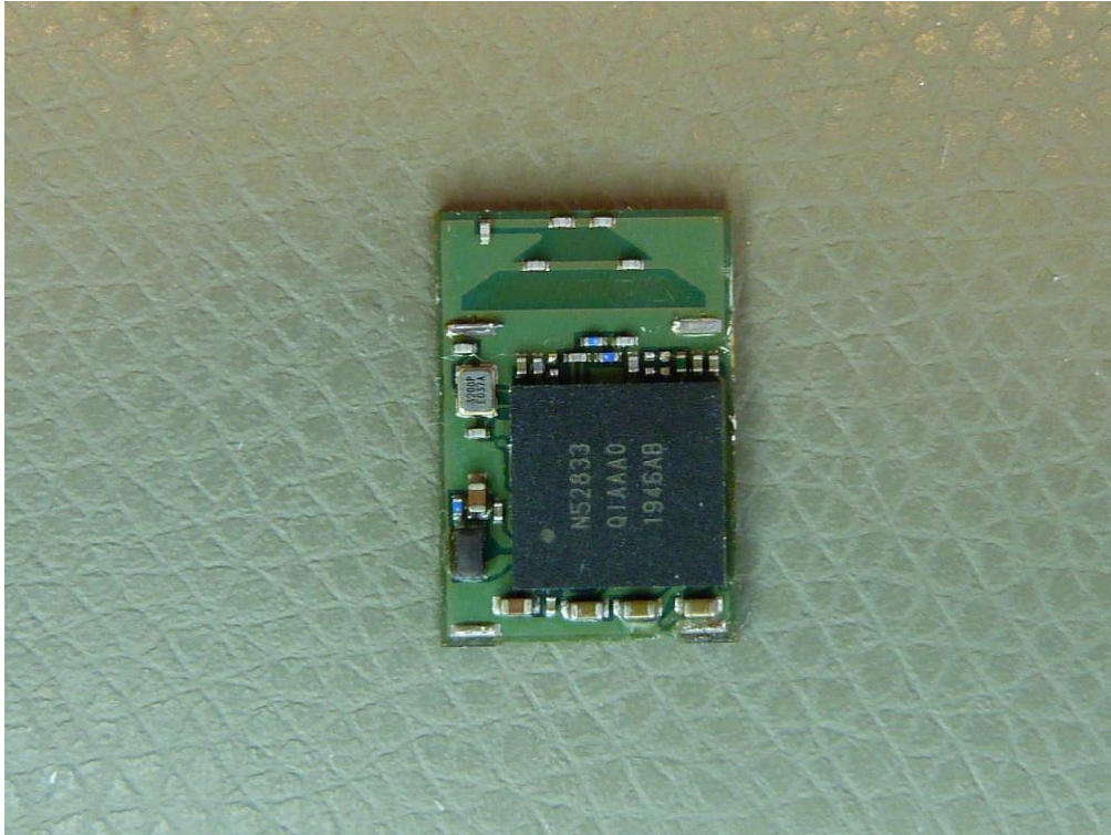
INTERNAL VIEW OF EUT (NINA-B406)
