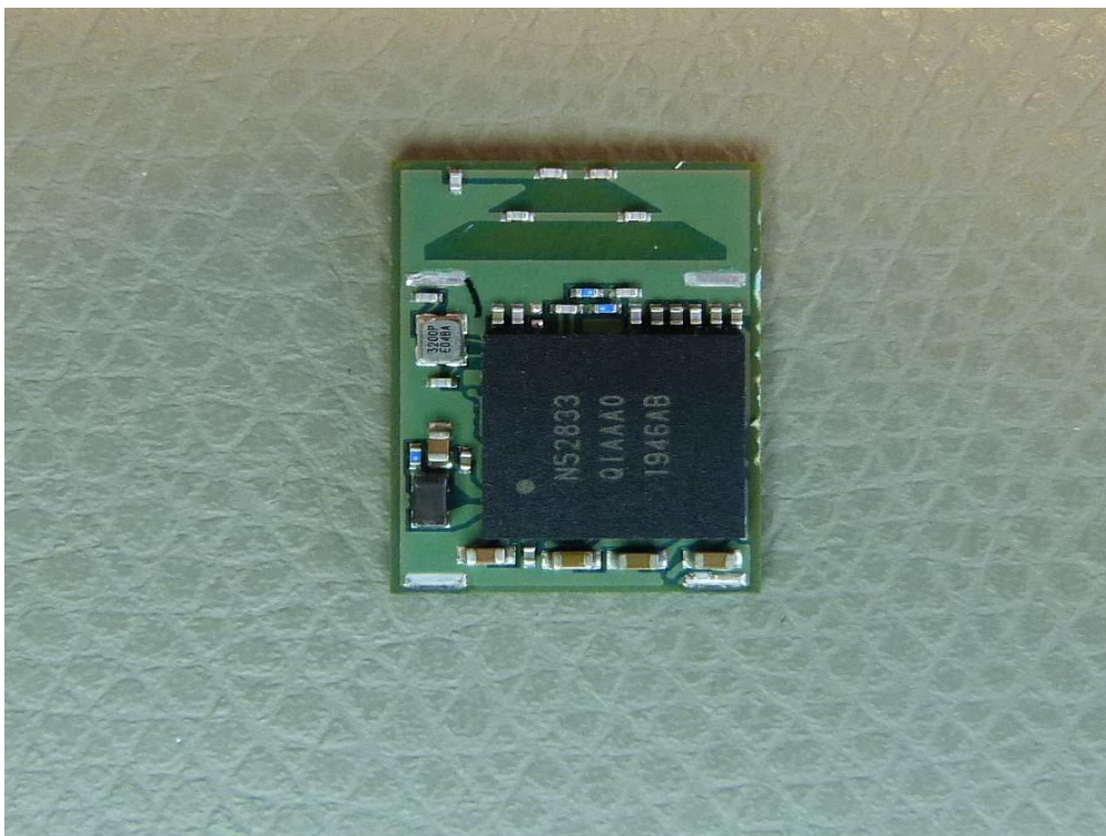
INTERNAL VIEW OF EUT (NINA-B416)
