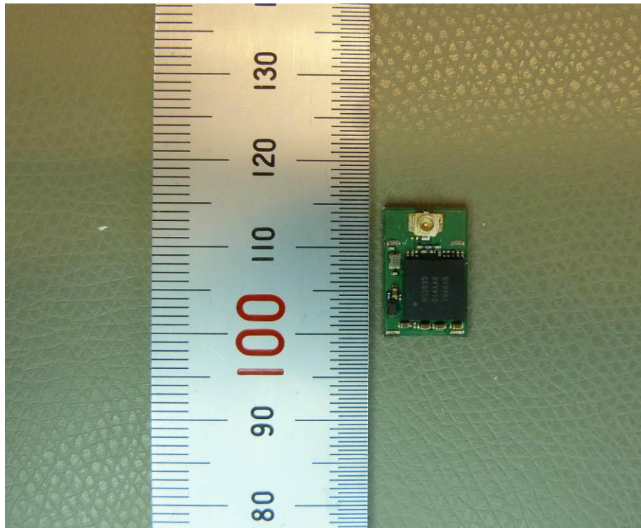
INTERNAL VIEW OF EUT (NINA-B400)
