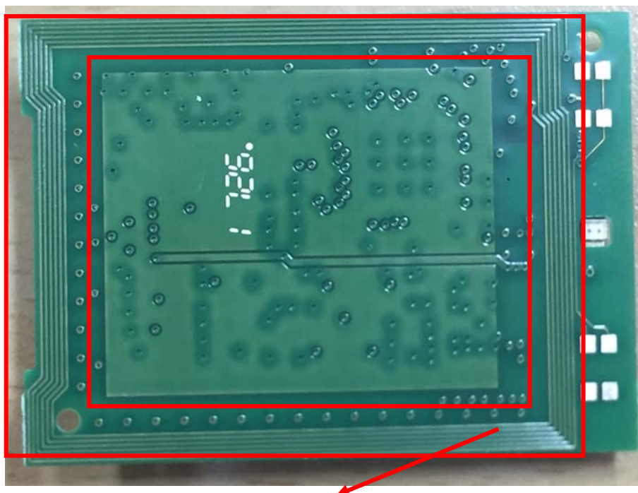
NFC receiving Antenna
