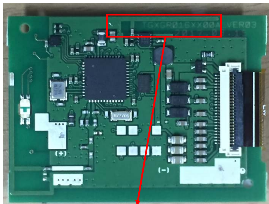
Zigbee receiving Antenna (Wake Up)
