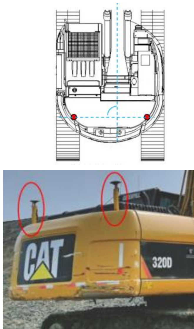
2-1 Antenna bracket installing
