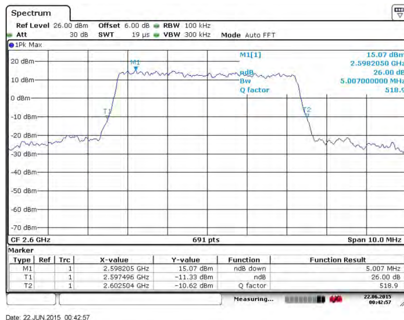
26dB Bandwidth Plot on Channel 40690
