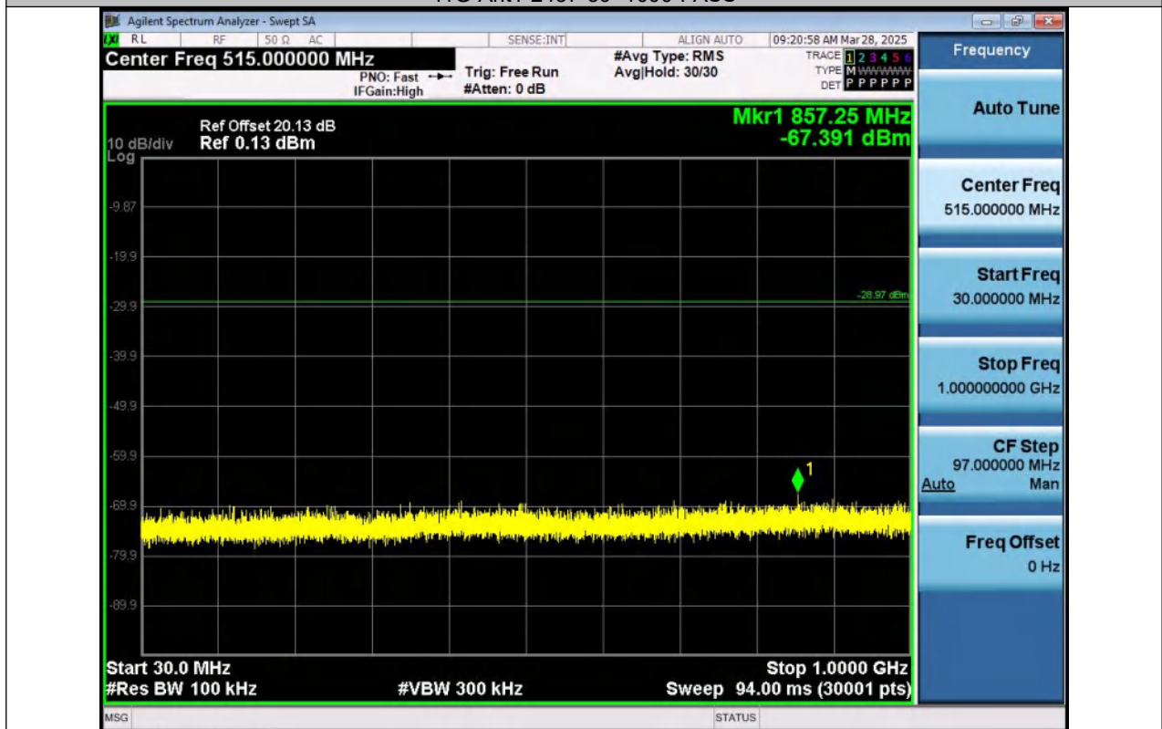
11G-Ant2-2437-30~1000-PASS
