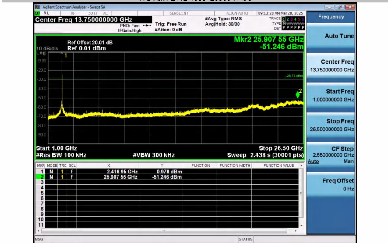
11G-Ant2-2412-1000~26500-PASS
