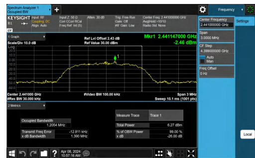
3DH5-Ant1-2441
