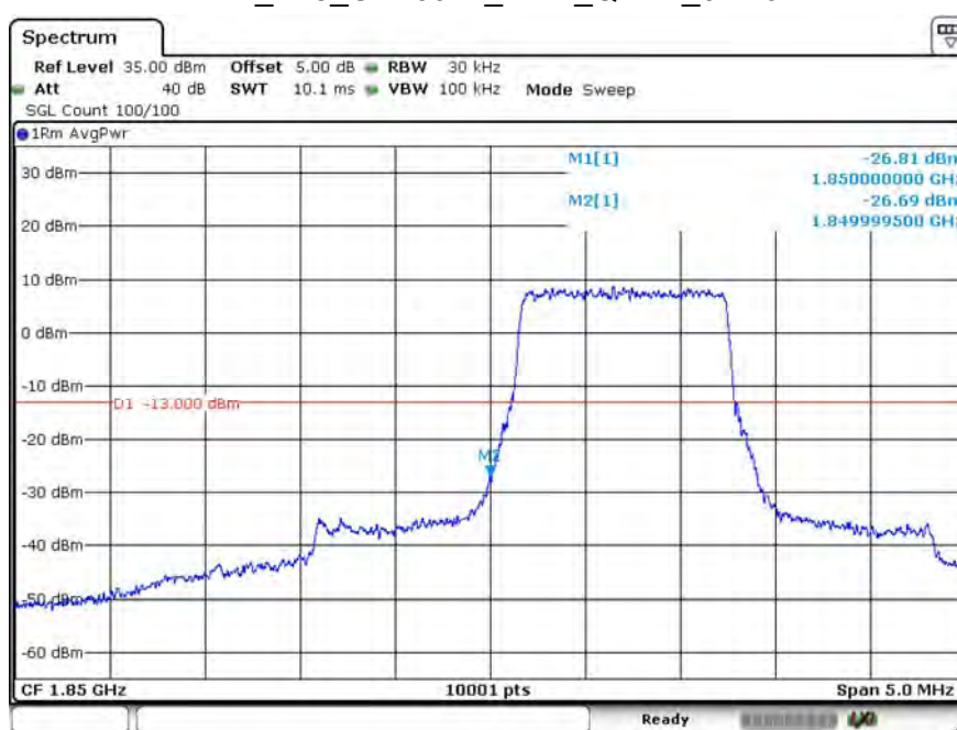
LTE_B25_CH26047_1.4M_QPSK_6RB0
