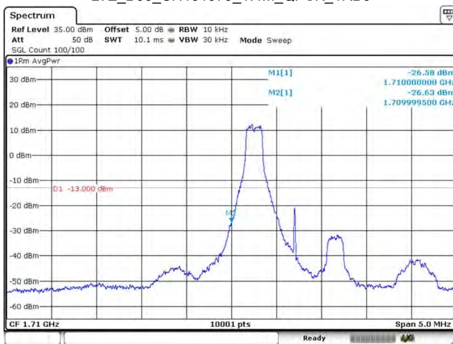
LTE_B66_CH131979_1.4M_QPSK_1RB0
