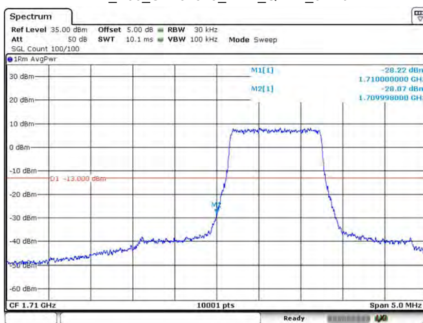
LTE_B66_CH131979_1.4M_QPSK_6RB0
