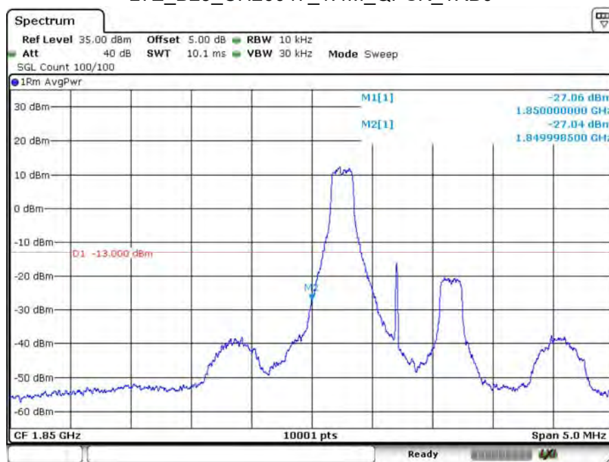
LTE_B25_CH26047_1.4M_QPSK_1RB0
