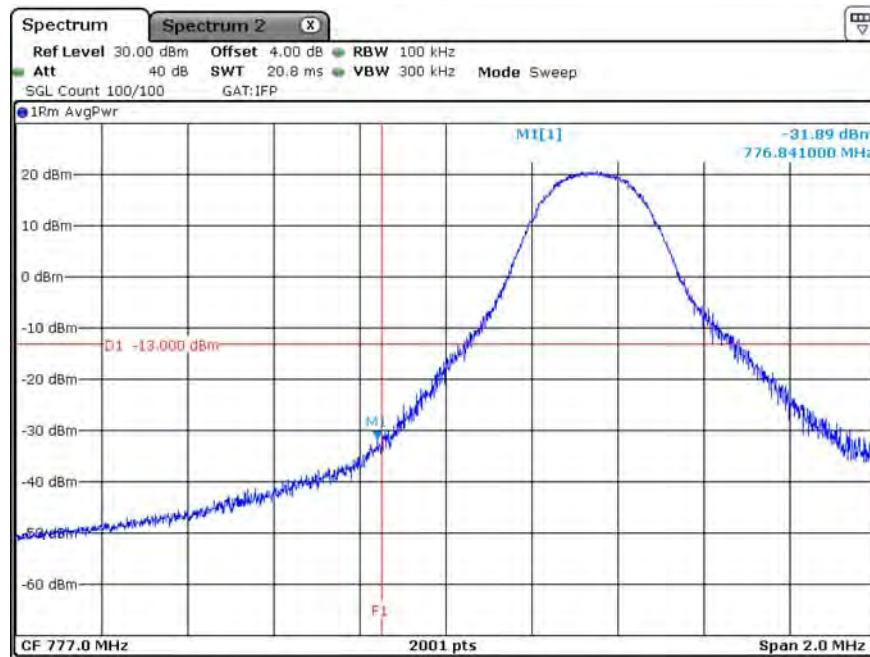
B13_CH23205_5M_QPSK_1RB0_150k
