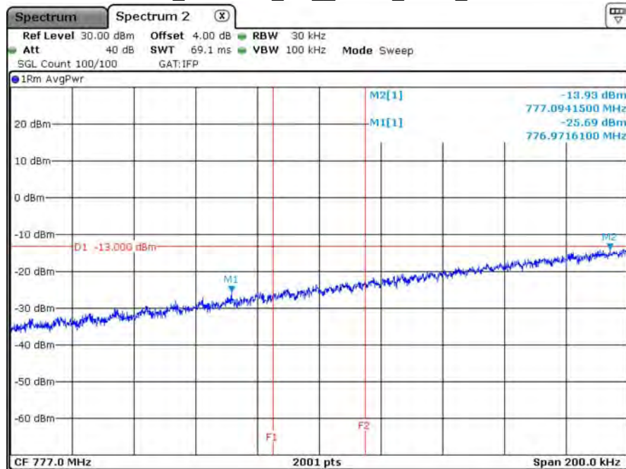
B13_CH23205_5M_QPSK_1RB0_15k
