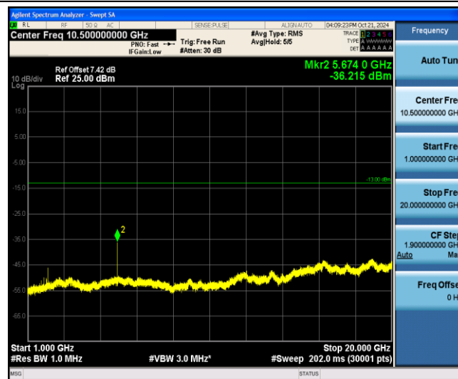
Band2-20MHz-16QAM-19100-1-0-Low-1000-20000--36.22-PASS
