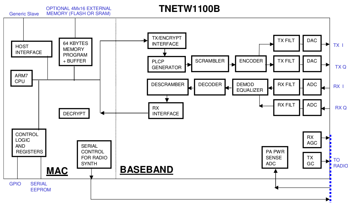
Fig. 66 Detail block diagram of TNETW1100B
