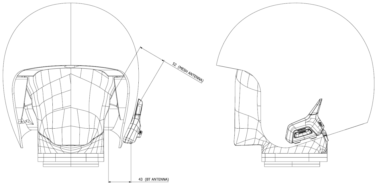
Figure E-1 Antenna Location
