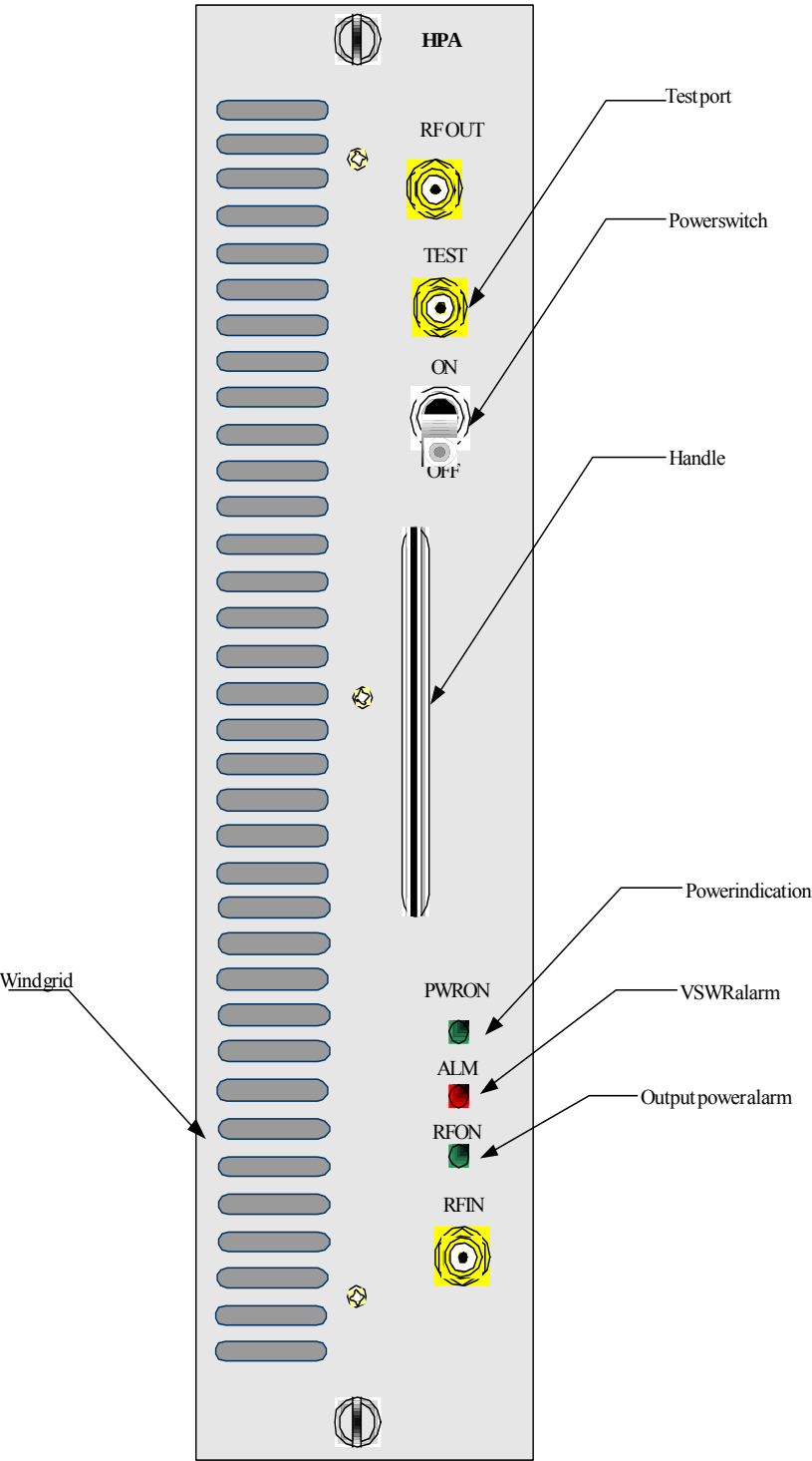
Fig. 12.2-2 Structure of the HPA Front Panel
