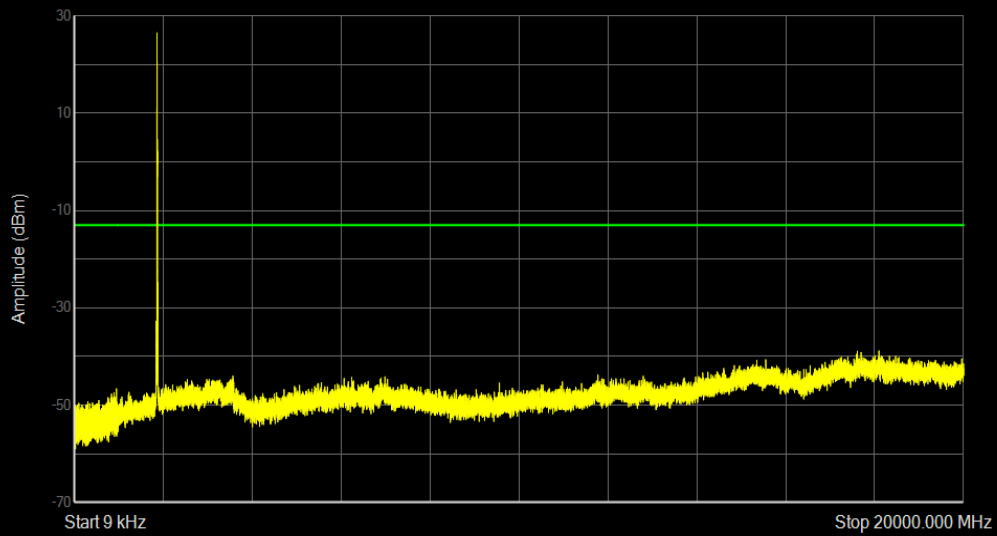
Band2 16QAM BW=10MHz Channel=18900 RB Size=1 Position=#0
