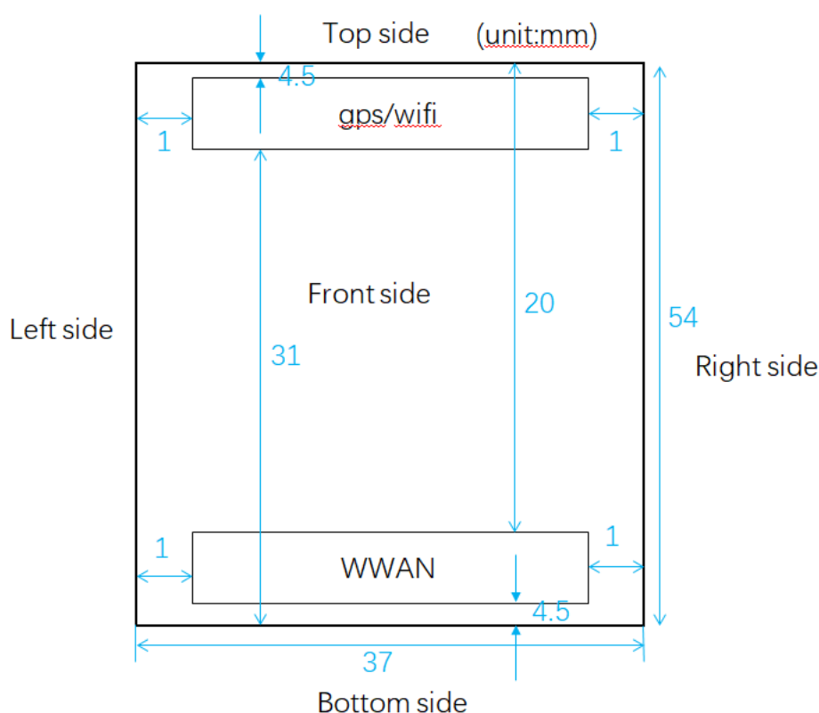
Fig.12.1 EUT Antenna Locations
