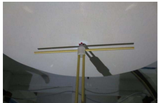
Fig.8.2 Photo of Dipole setup
