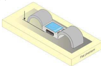
Fig.8.1 Illustration for Limb-worn Position
