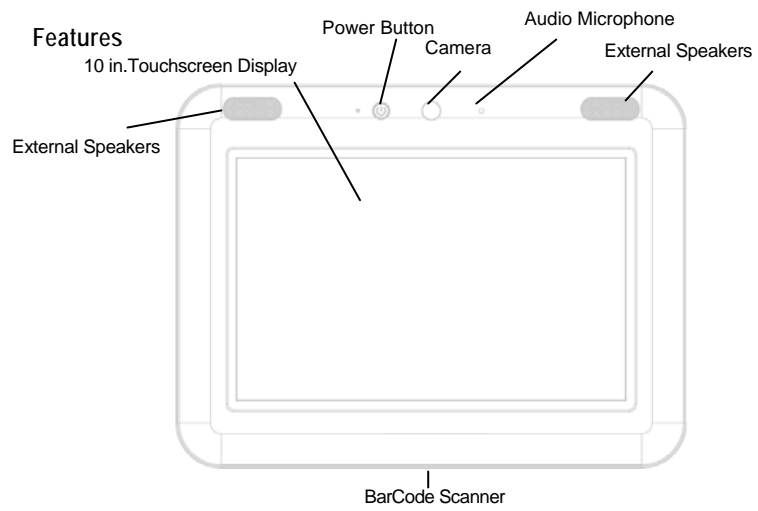
Figure 1. Front view
