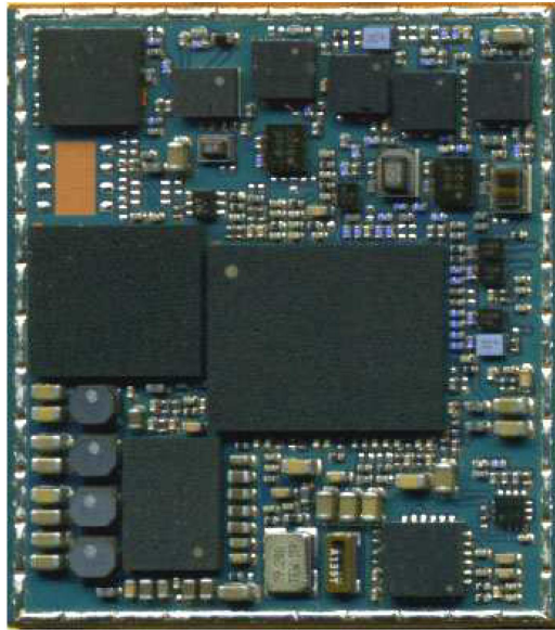
PHS8-P Top side
