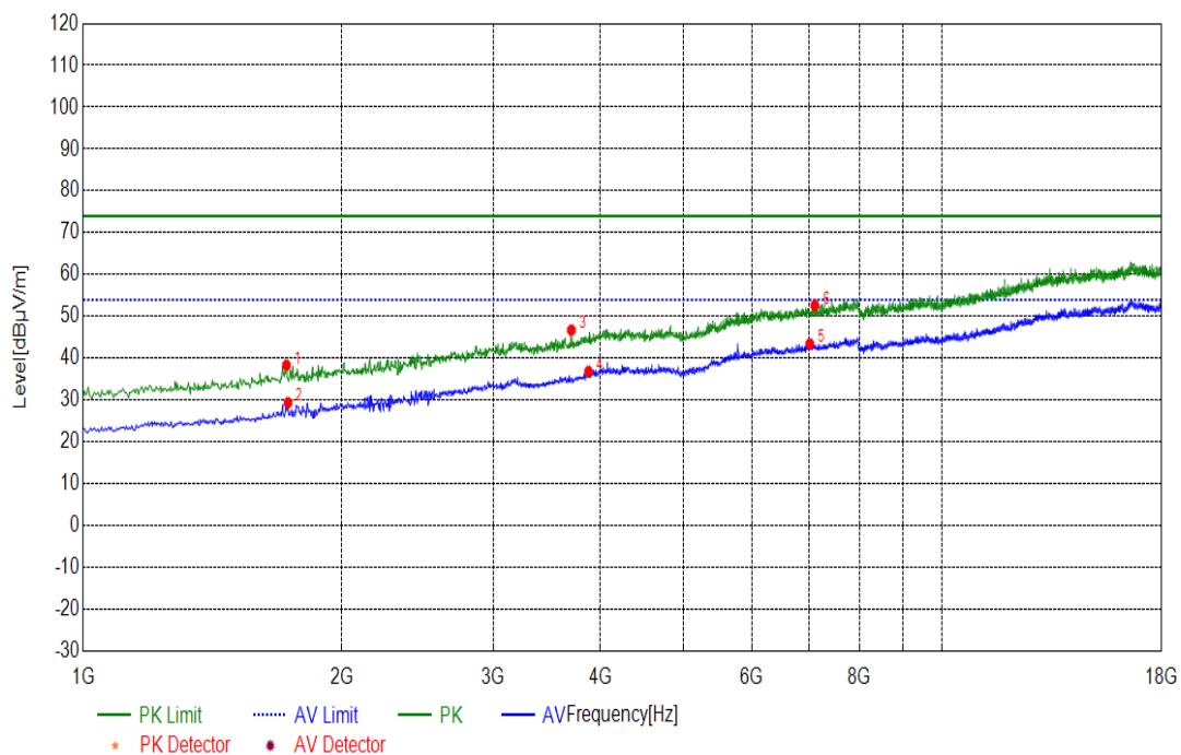
(Plot M: Test Antenna Horizontal 1G – 18G)
