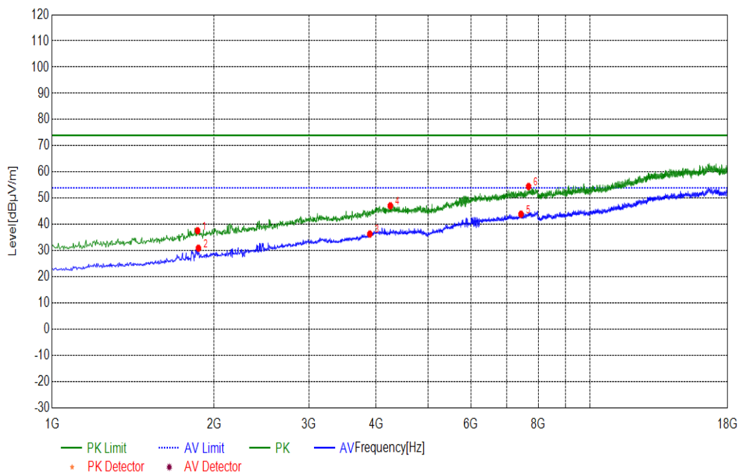
(Plot N: Test Antenna Vertical 1G – 18G)
