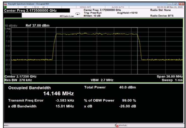
Figure 360: 64QAM 15MHz B.W.; 2172.5MHz, 15kHz - Input
