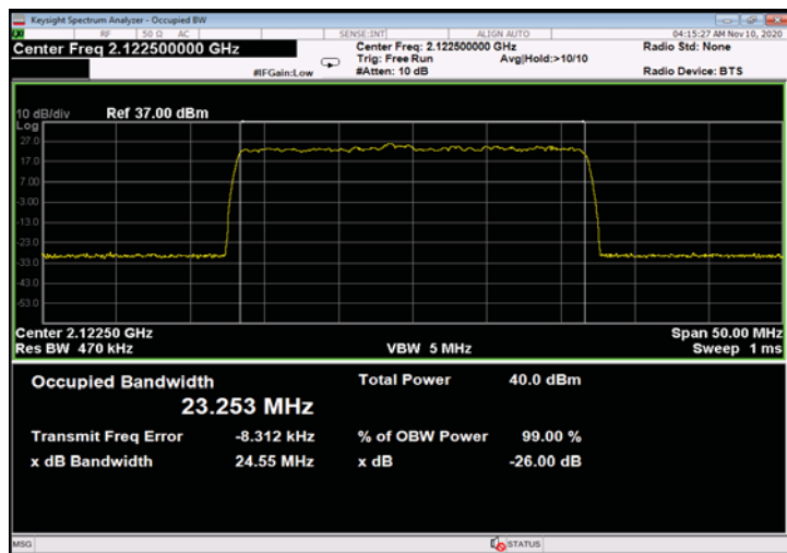
Figure 373: 64QAM 25MHz B.W.; 2122.5MHz, 30kHz - Input
