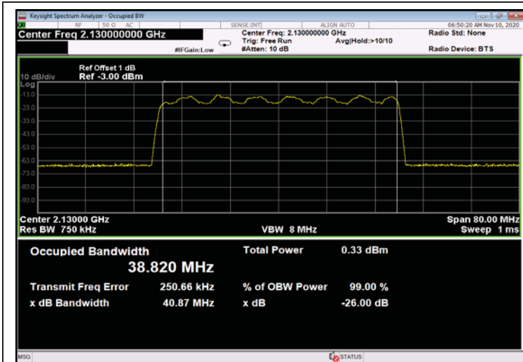
Figure 315: 16QAM 40MHz B.W.; 2130.0MHz, 15kHz - Input
