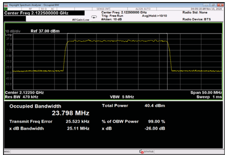
Figure 372: 64QAM 25MHz B.W.; 2122.5MHz, 15kHz - Input
