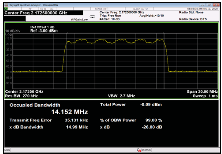
Figure 294: 16QAM 15MHz B.W.; 2172.5MHz, 15kHz - Input
