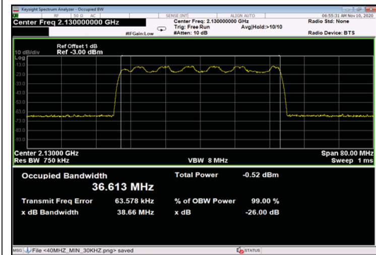
Figure 317: 16QAM 40MHz B.W.; 2130.0MHz, 60kHz - Input
