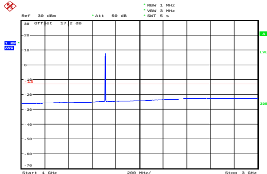
LTE Band 4 1.4MHz CH-Low 1GHz~3GHz
