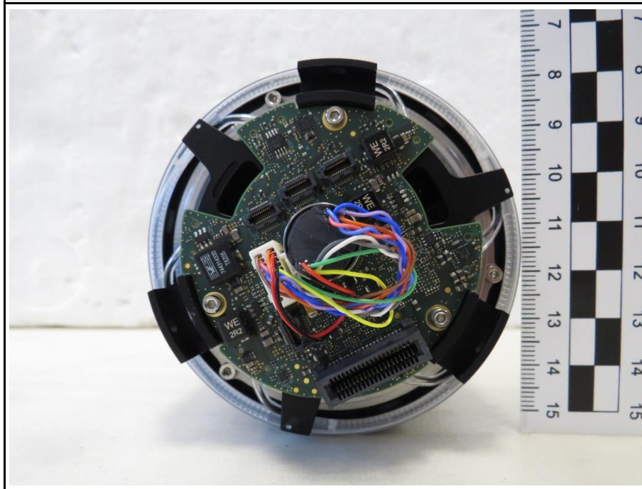
LASER SCANNER BOTTOM SIDE
