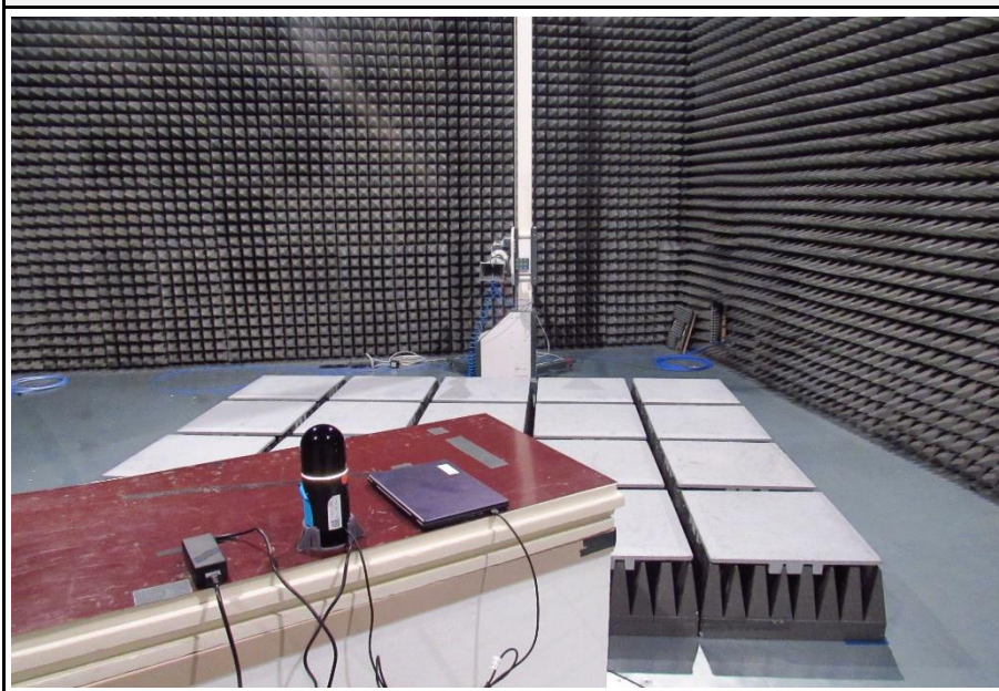
Setup 6.5-18 GHz
