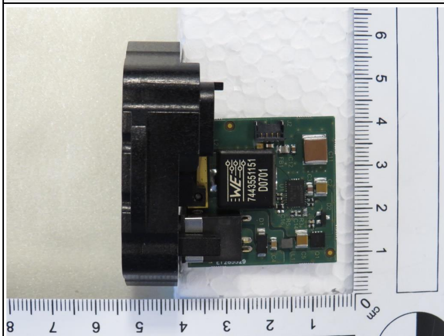
POWERBOARD TOP SIDE
