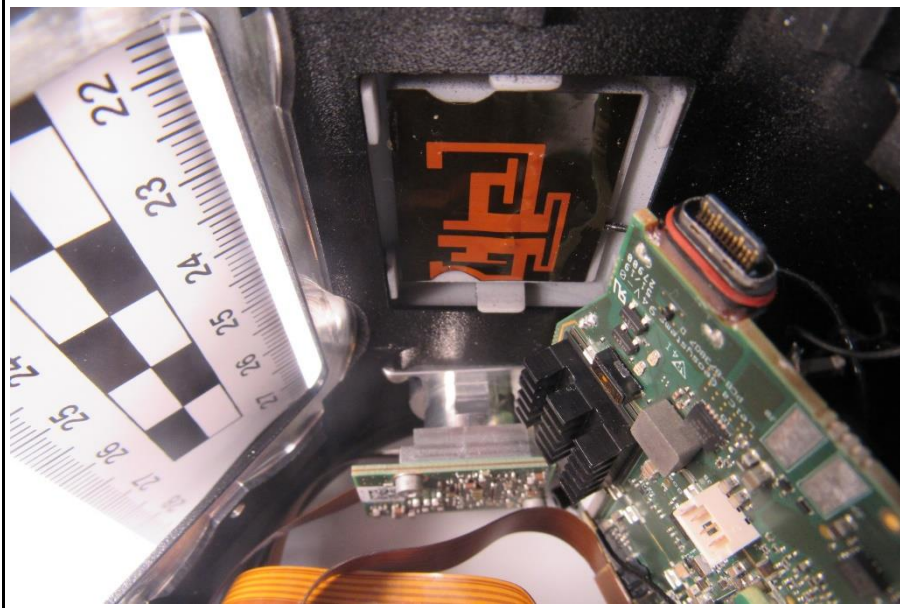
WLAN/BT Antenna 2
