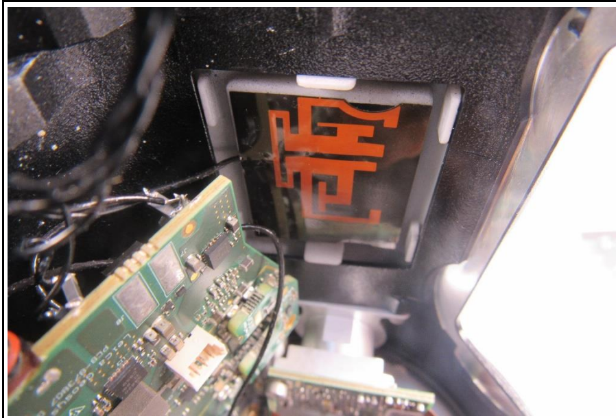
WLAN/BT Antenna 1
