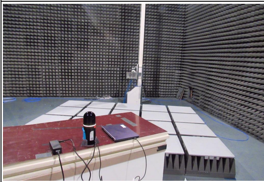
Setup 1-6.5 GHz
