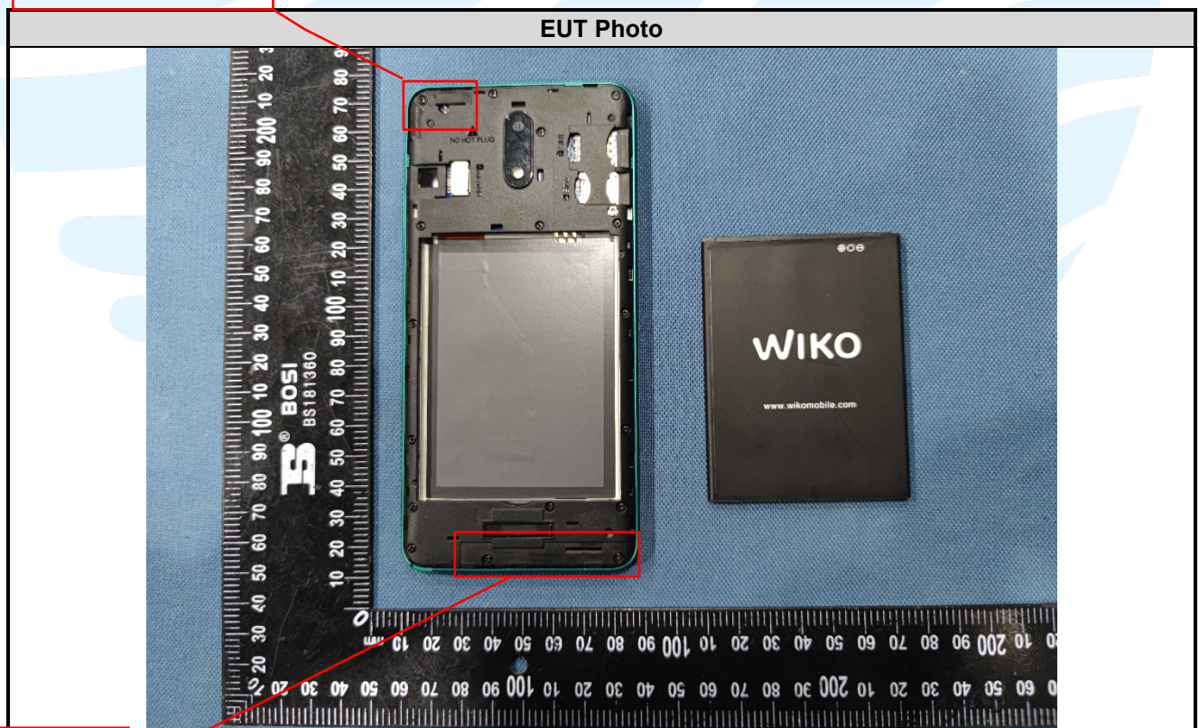
2G/3G Antenna
