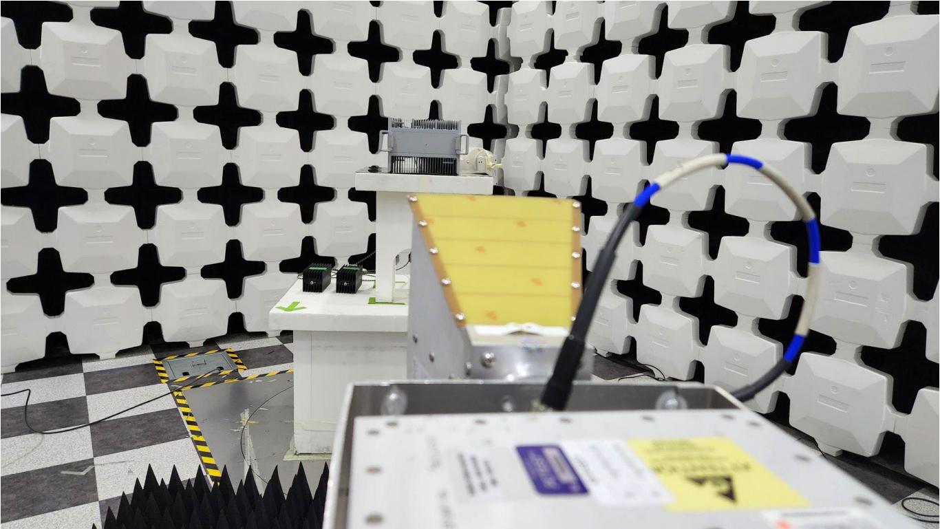
Above 1GHz Test Instrument & Measurement Setup
