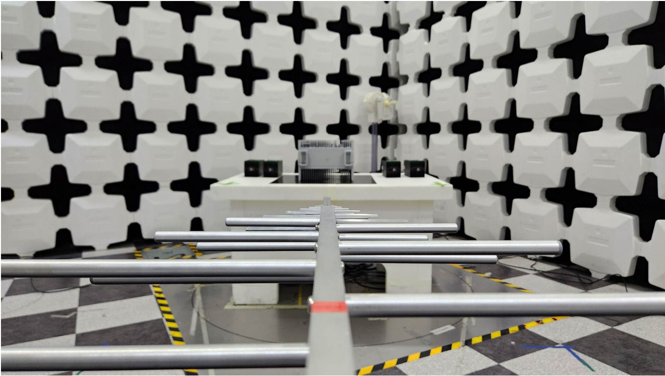
Below 1GHz Test Instrument & Measurement Setup
