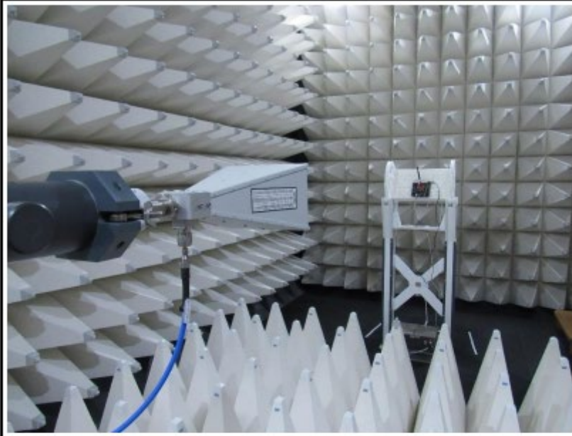
Test Setup – Radiated Measurement
