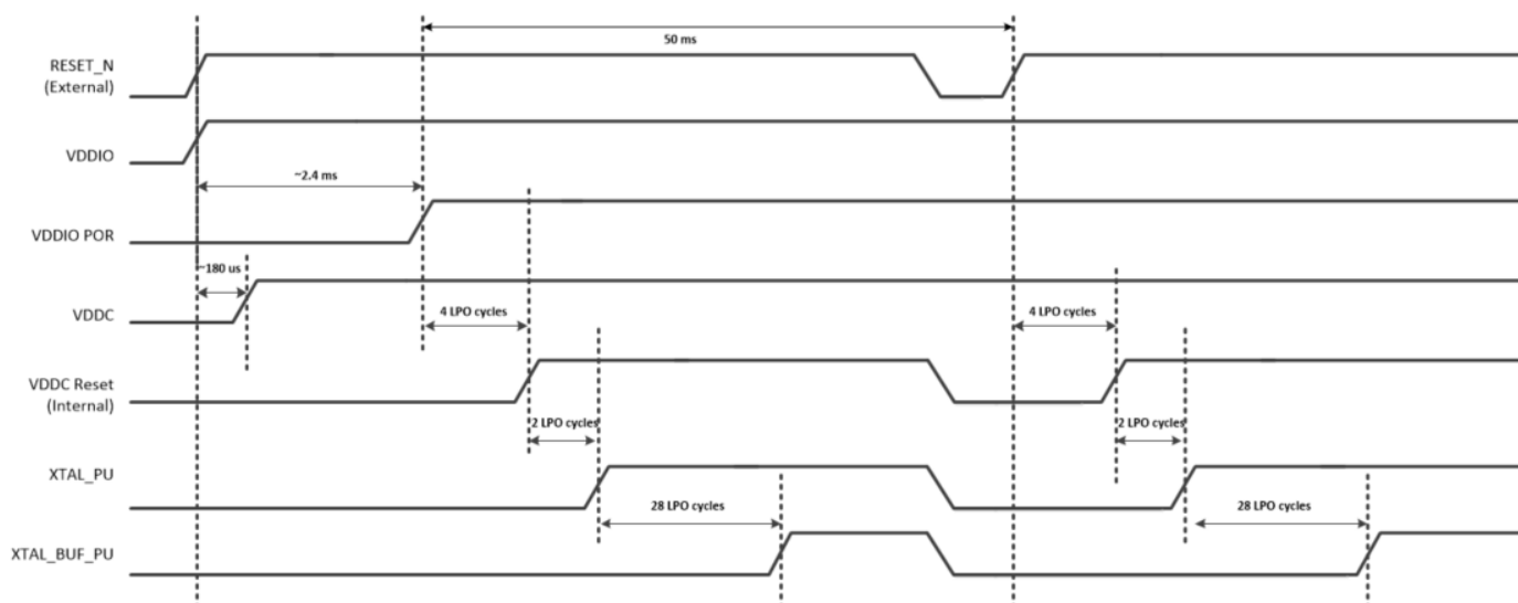
Figure 10. Reset Timing
