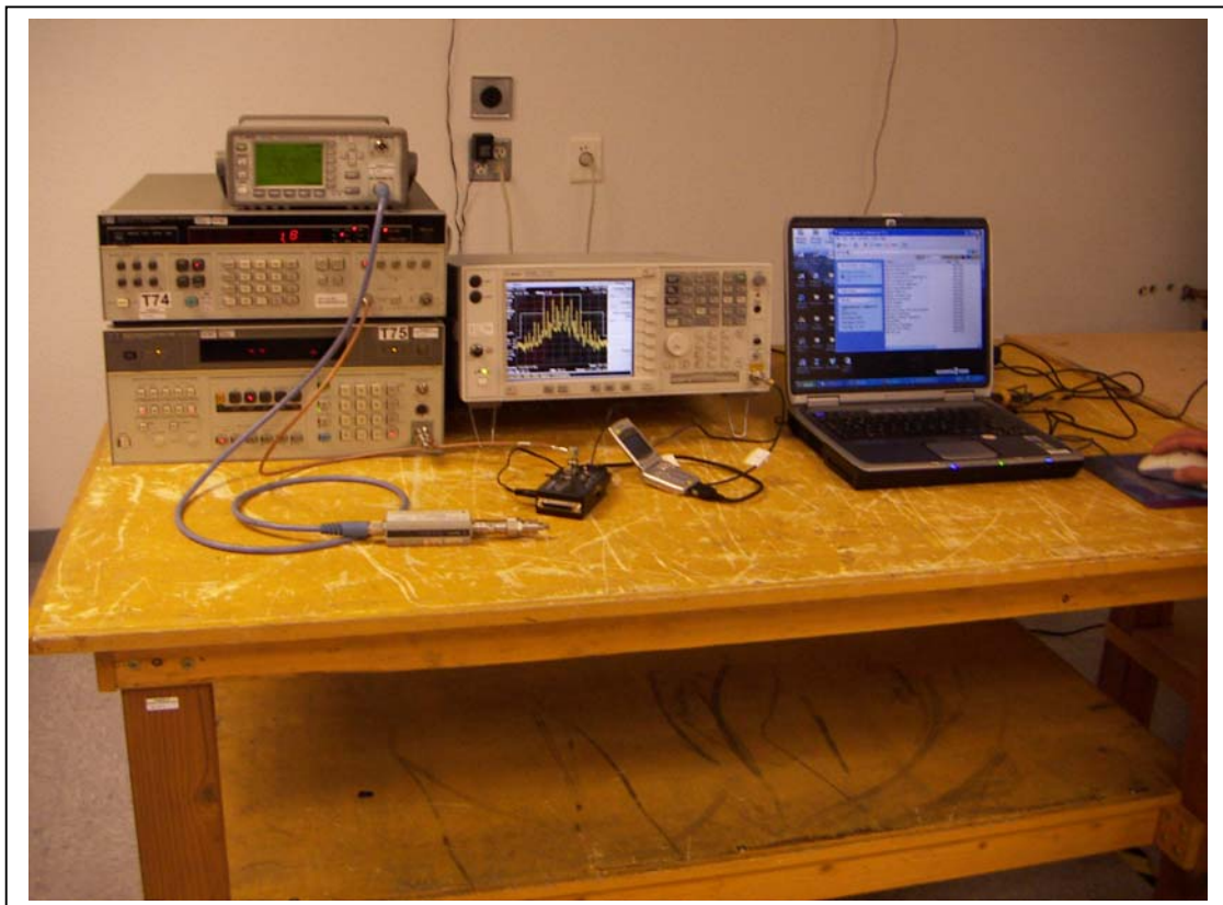
Set-up Photo
