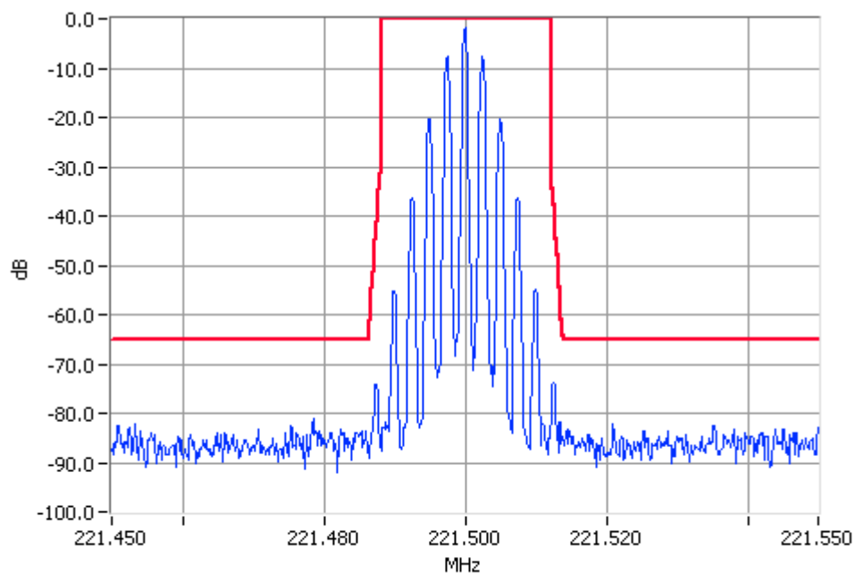
Analogue Modulation 221.5000MHz Mask Fx5 10W Pass RBW=300Hz VBW=3000Hz
