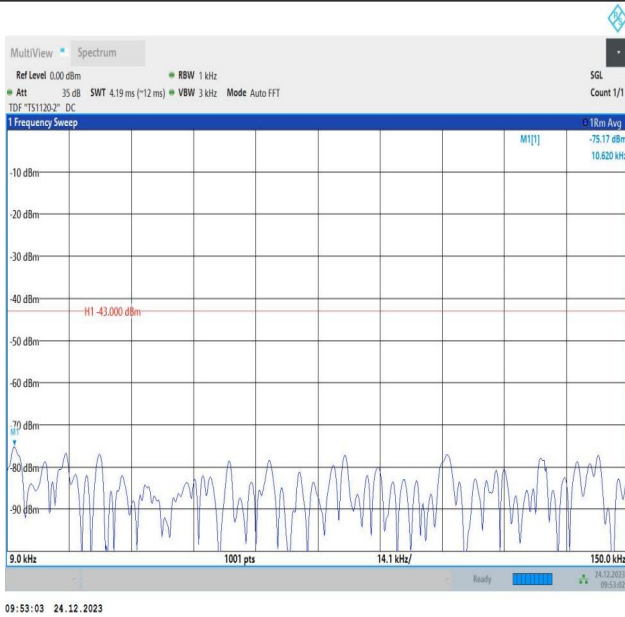
2-2-20MHz-10MHz-QPSK-QPSK-19001-19145-1RB#0-1RB#4 9-0.009~0.15MHz-PASS
