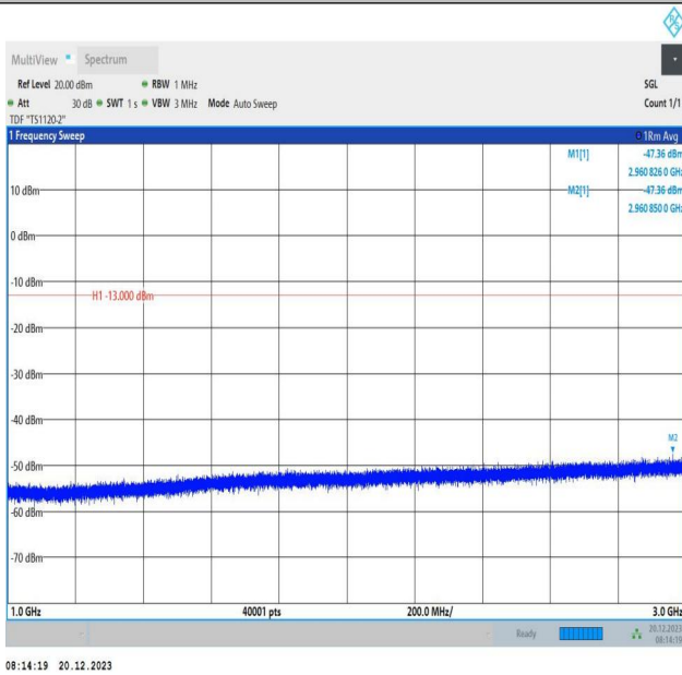
2-2-20MHz-10MHz-64QAM-64QAM-18851-18995-100RB#0-4 ORB#0-1000~3000MHz-PASS
