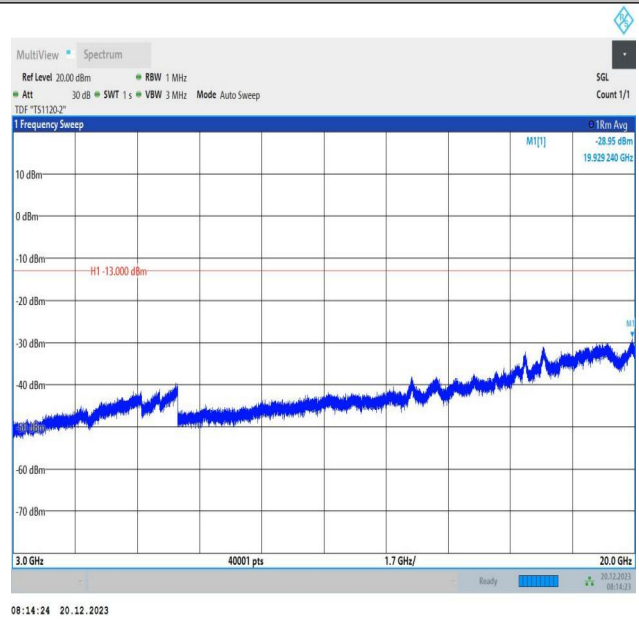
2-2-20MHz-10MHz-64QAM-64QAM-18851-18995-100RB#0-4 ORB#0-3000~20000MHz-PASS
