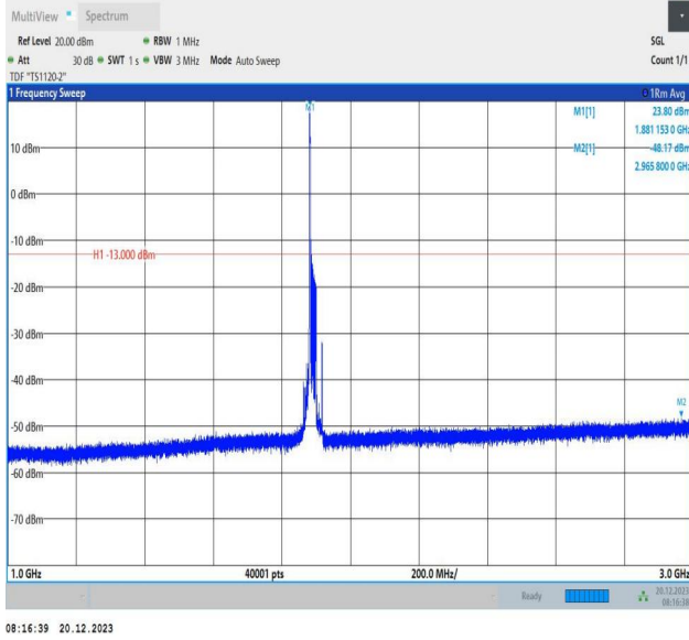
2-2-20MHz-10MHz-16QAM-16QAM-19001-19145-1RB#0-0RB #0-1000~3000MHz-PASS
