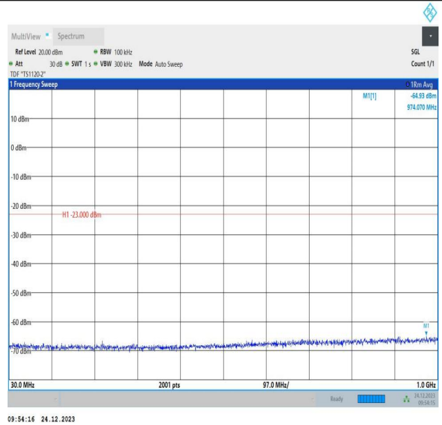
2-2-20MHz-10MHz-QPSK-QPSK-19001-19145-100RB#0-40R B#0-30~1000MHz-PASS
