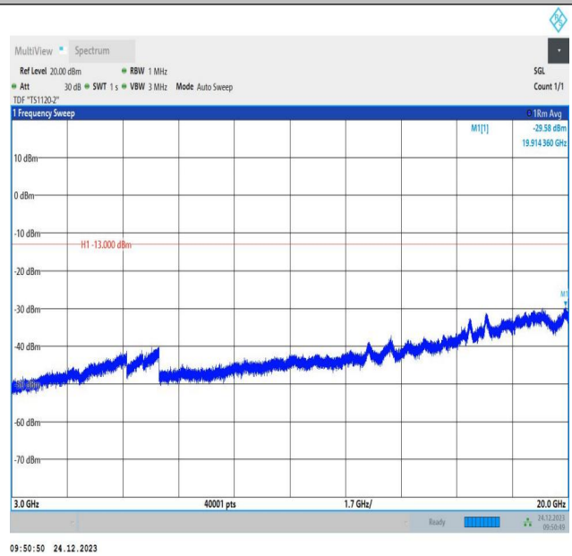
2-2-20MHz-10MHz-QPSK-QPSK-18851-18995-100RB#0-40R B#0-3000~20000MHz-PASS
