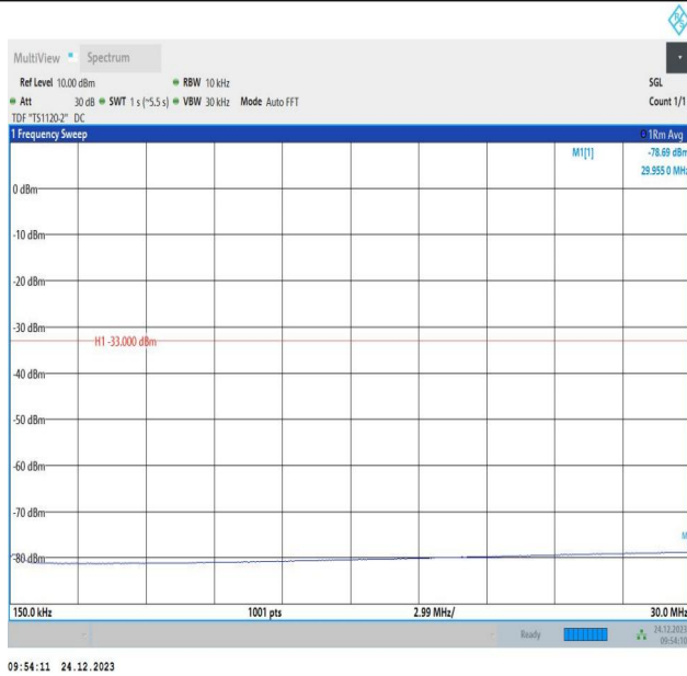
2-2-20MHz-10MHz-QPSK-QPSK-19001-19145-100RB#0-40R B#0-0.15~30MHz-PASS
