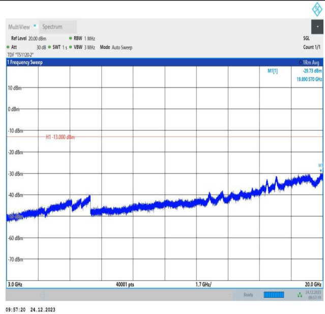
2-2-15MHz-10MHz-QPSK-QPSK-18675-18795-1RB#74-0RB# 0-3000~20000MHz-PASS
