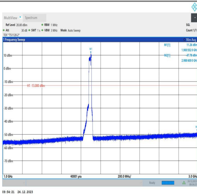
2-2-20MHz-10MHz-QPSK-QPSK-19001-19145-100RB#0-40R B#0-1000~3000MHz-PASS
