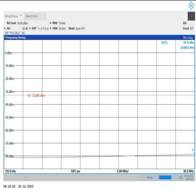
2-2-20MHz-10MHz-64QAM-64QAM-19001-19145-1RB#0-0RB #0-0.15~30MHz-PASS
