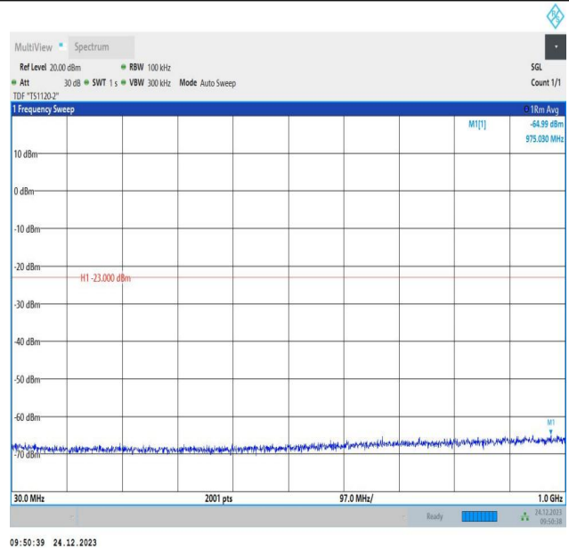
2-2-20MHz-10MHz-QPSK-QPSK-18851-18995-100RB#0-40R B#0-30~1000MHz-PASS
