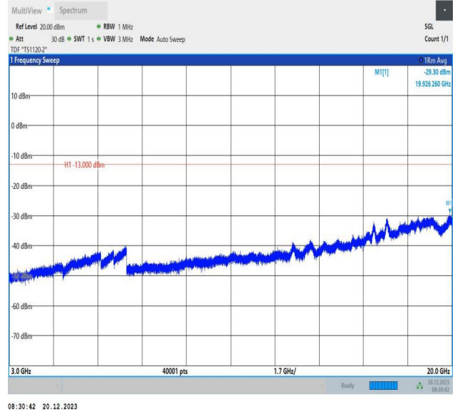
2-2-20MHz-10MHz-64QAM-64QAM-19001-19145-1RB#99-0R B#0-3000~20000MHz-PASS
