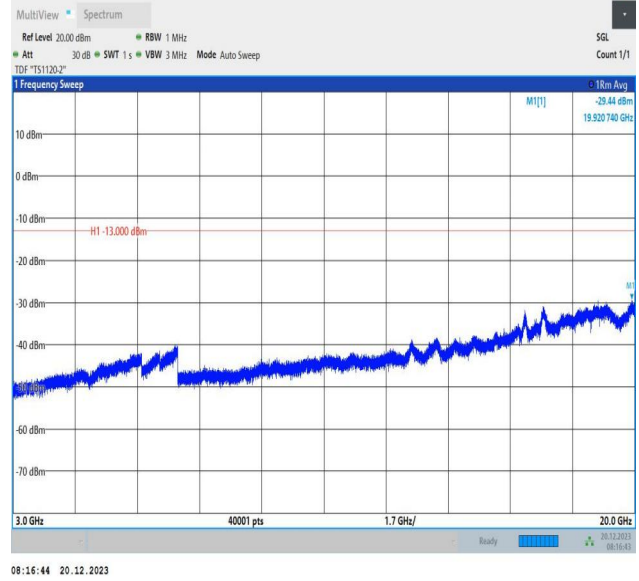
2-2-20MHz-10MHz-16QAM-16QAM-19001-19145-1RB#0-0RB #0-3000~20000MHz-PASS
