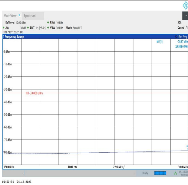
2-2-20MHz-10MHz-QPSK-QPSK-18851-18995-100RB#0-40R B#0-0.15~30MHz-PASS
