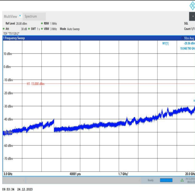
2-2-20MHz-10MHz-QPSK-QPSK-19001-19145-1RB#0-1RB#4 9-3000~20000MHz-PASS
