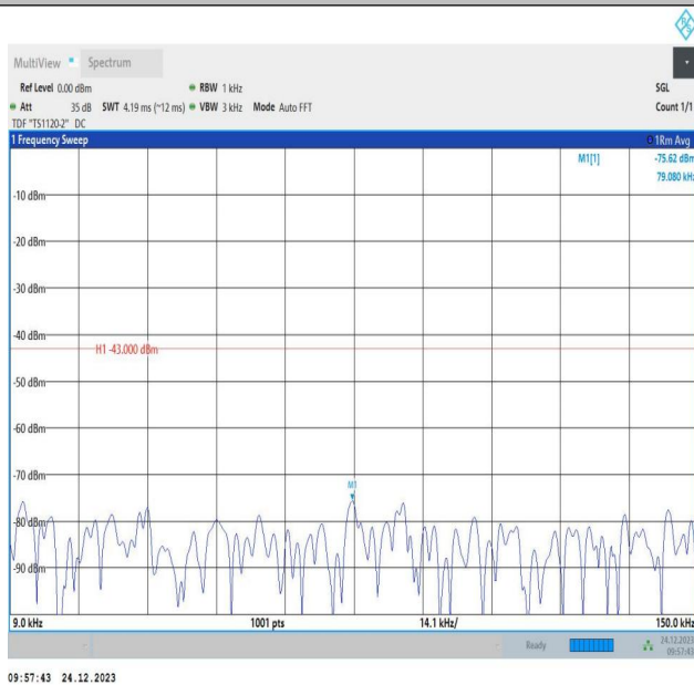
2-2-15MHz-10MHz-QPSK-QPSK-18675-18795-1RB#0-1RB#4 9-0.009~0.15MHz-PASS
