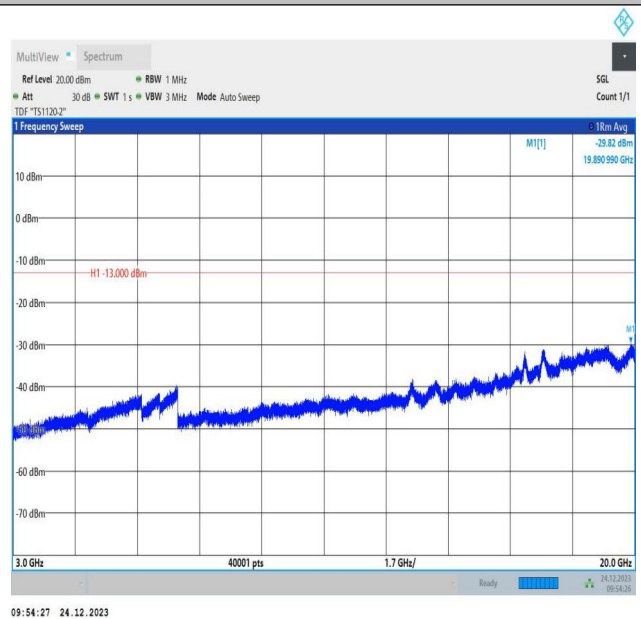
2-2-20MHz-10MHz-QPSK-QPSK-19001-19145-100RB#0-40R B#0-3000~20000MHz-PASS
