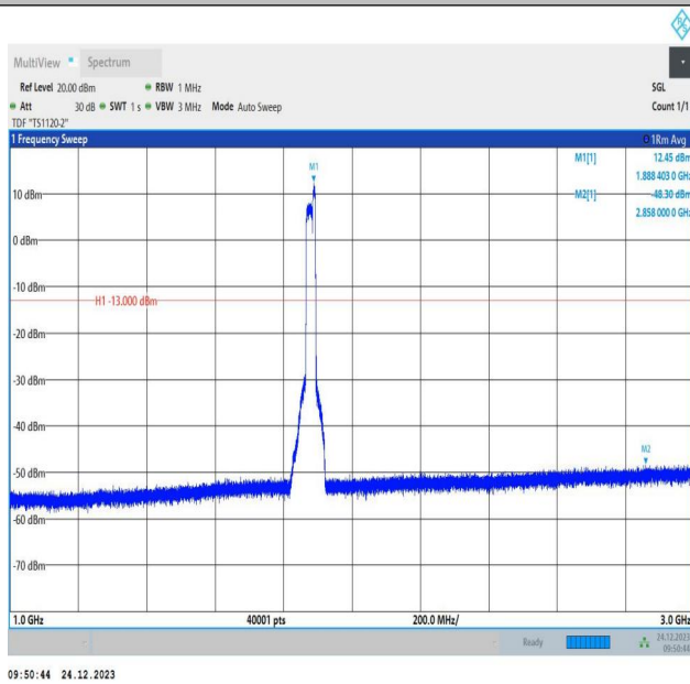
2-2-20MHz-10MHz-QPSK-QPSK-18851-18995-100RB#0-40R B#0-1000~3000MHz-PASS
