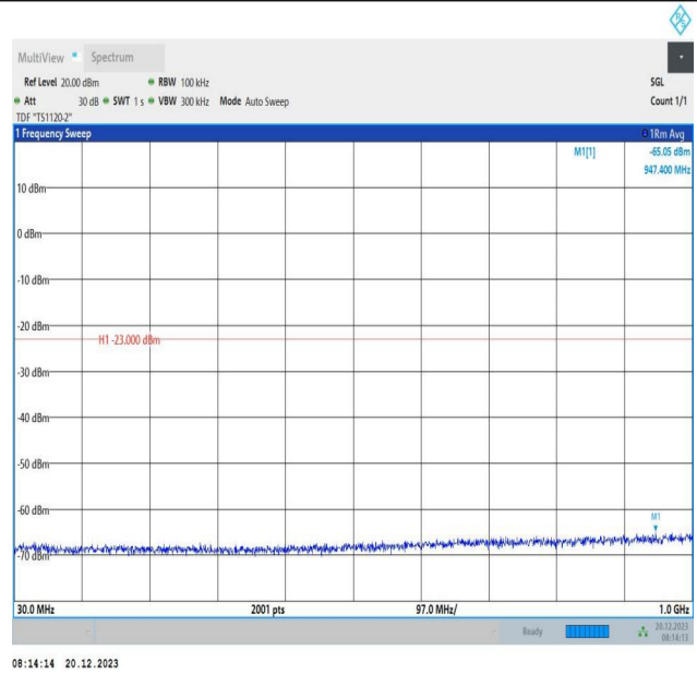
2-2-20MHz-10MHz-64QAM-64QAM-18851-18995-100RB#0-4 ORB#0-30~1000MHz-PASS
