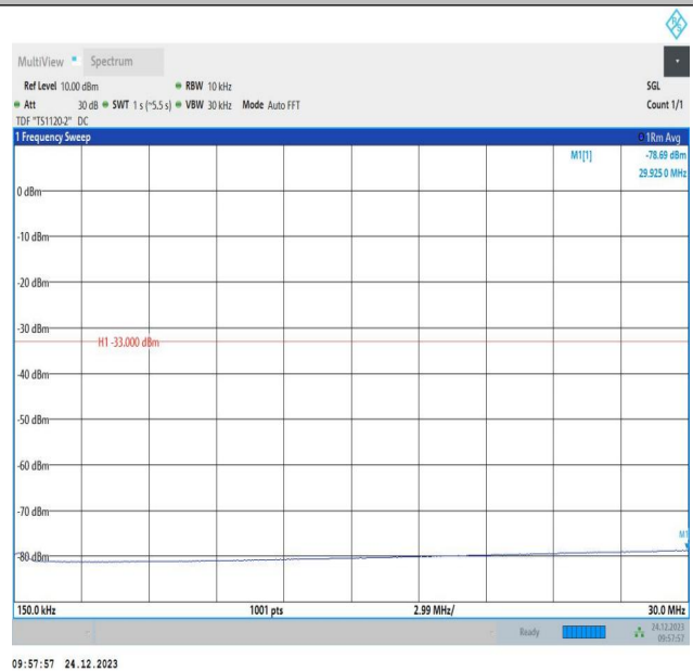
2-2-15MHz-10MHz-QPSK-QPSK-18675-18795-1RB#0-1RB#4 9-0.15~30MHz-PASS
