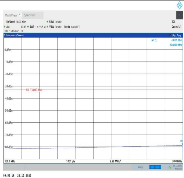
2-2-20MHz-10MHz-QPSK-QPSK-19001-19145-1RB#0-1RB#4 9-0.15~30MHz-PASS
