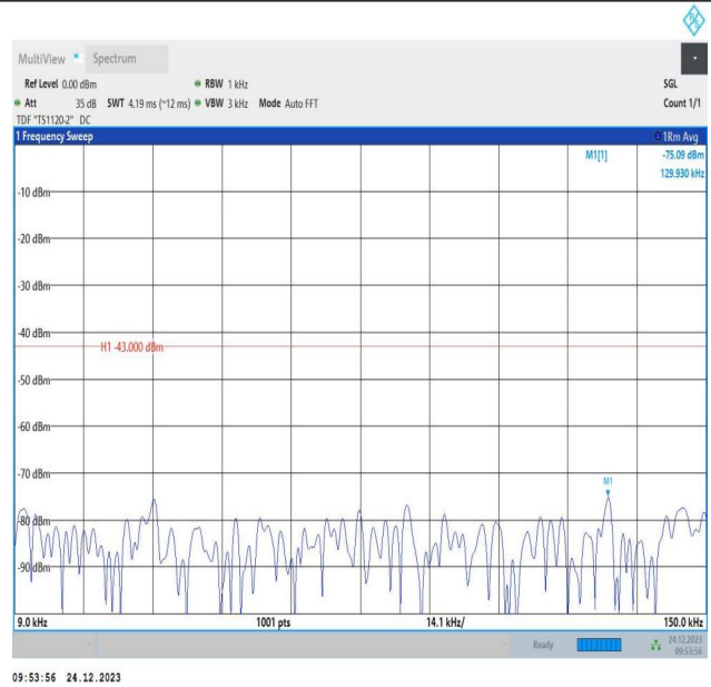
2-2-20MHz-10MHz-QPSK-QPSK-19001-19145-100RB#0-40R B#0-0.009~0.15MHz-PASS
