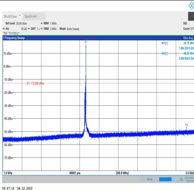
2-2-15MHz-10MHz-QPSK-QPSK-18675-18795-1RB#74-0RB# 0-1000~3000MHz-PASS
