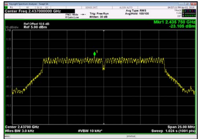
Power spectral density-802.11n(HT20) ,2437MHz
