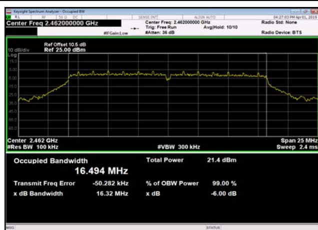
6dB Bandwidth-802.11g,2462MHz
