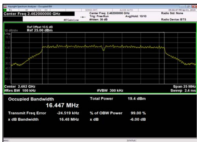
6dB Bandwidth-802.11n(HT20),2462MHz
