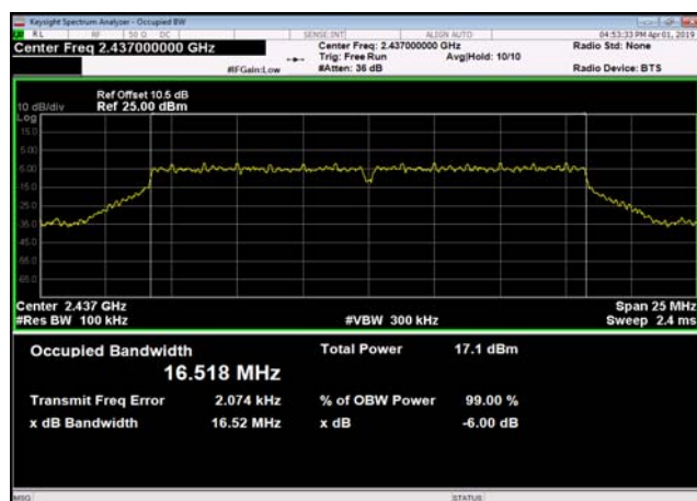
6dB Bandwidth-802.11n(HT20),2437MHz
