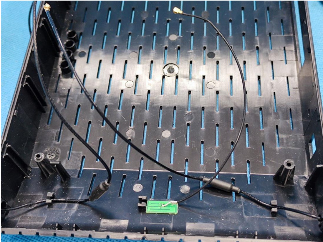
Antenna Inside
