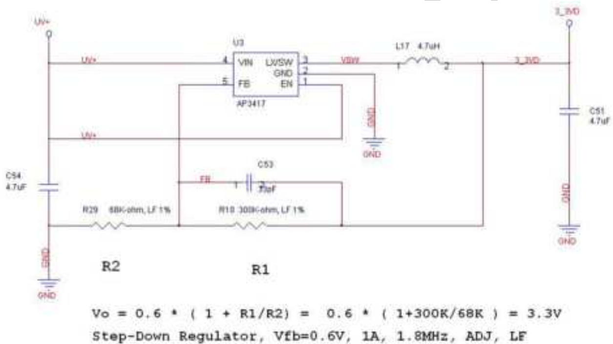
Fig 10 Power supply Circuit schematic
