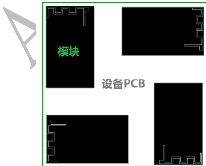
Fig 9 Recommended PCB layout
