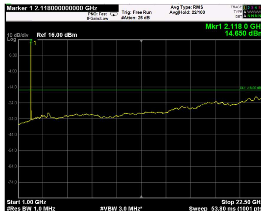
Channel: BOTTOM, Modulation: 256QAM, BW=15MHz, Range: Upper
