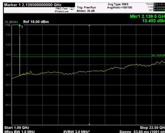
Channel: MIDDLE, Modulation: 256QAM, BW=15MHz, Range: Upper
