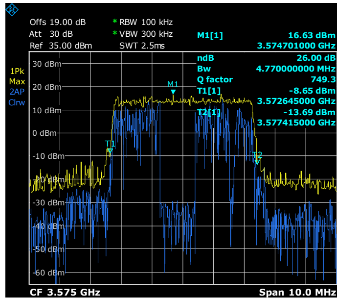
LTE Band 42_5 MHz BW / Middle Channel 3575 MHz / QPSK / 26dB BW
