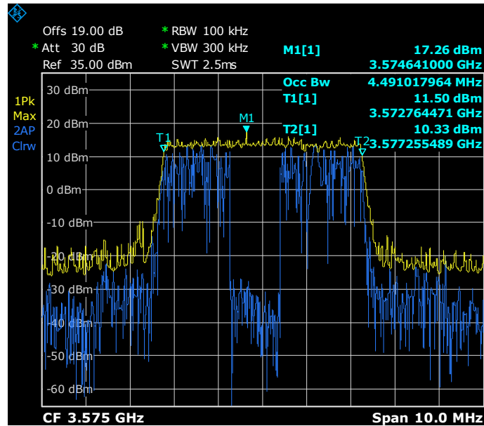
LTE Band 42_5 MHz BW / Middle Channel 3575 MHz / QPSK / 99%OBW
