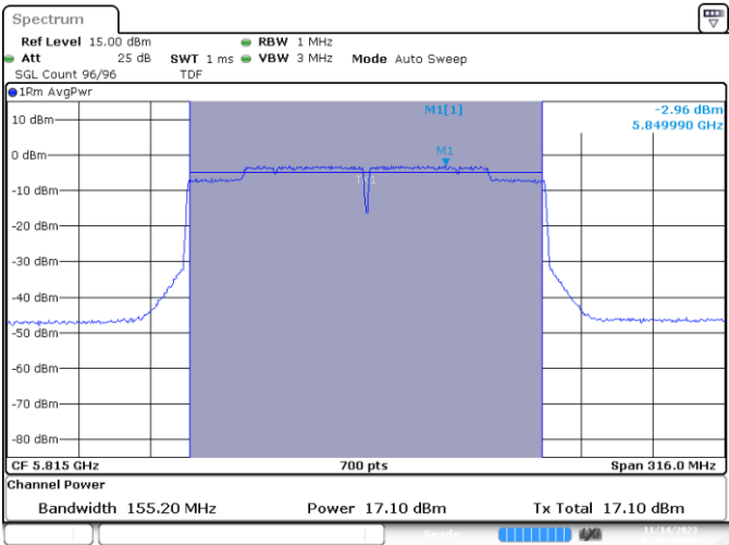
MIMO-A,802.11ax/be160,MCS0-CH163
