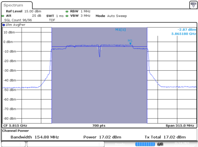
MIMO-B,802.11ax/be160,MCS0-CH163
