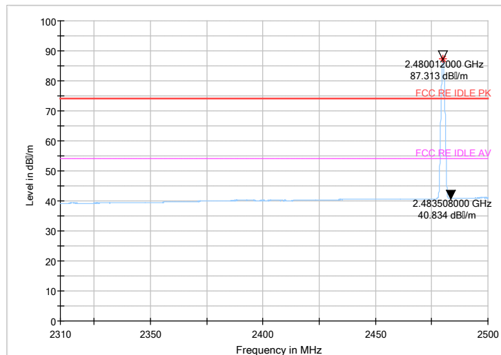
Fig.59 Radiated emission (Power): GFSK, high channel
