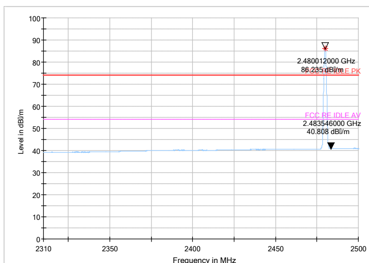
Fig.49 Radiated emission (Power): \pi/4 DQPSK, high channel
