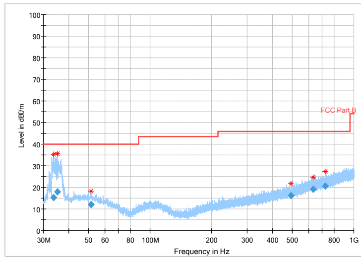
Fig.45 Radiated emission: \pi/4 DQPSK, Ch78, 30MHz~1GHz
