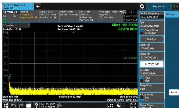
Band4-15MHz-QPSK-20325-1RB#74-0.15~30-PASS
