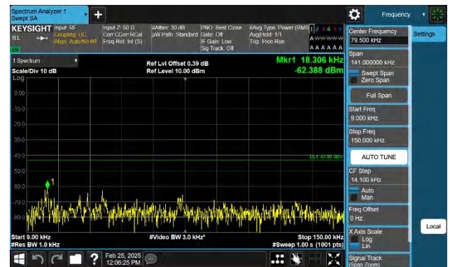
Band4-10MHz-QPSK-20175-1RB#49-0.009~0.15-PASS
