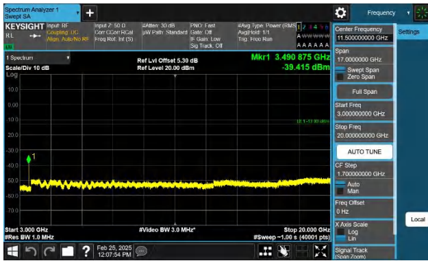
Band4-10MHz-QPSK-20350-1RB#0-3000~20000-PASS
