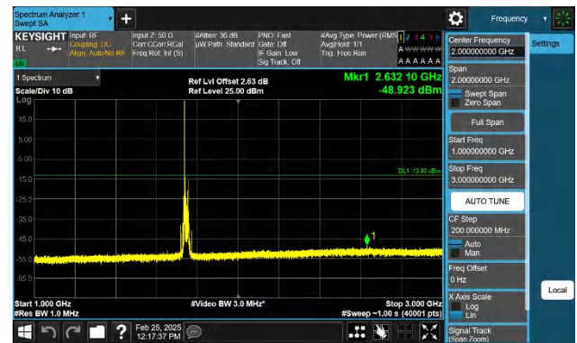
Band4-20MHz-QPSK-20300-1RB#0-1000~3000-PASS
