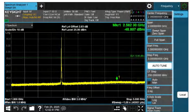
Band4-5MHz-QPSK-20375-1RB#0-1000~3000-PASS
