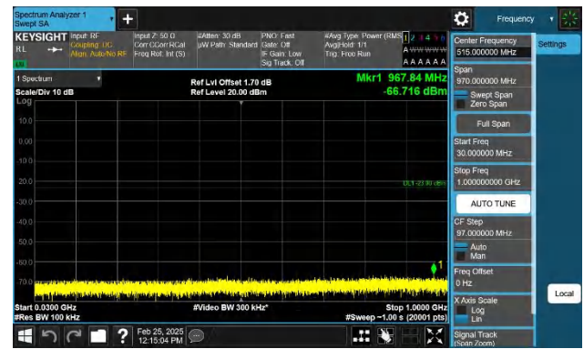
Band4-20MHz-QPSK-20050-1RB#99-30~1000-PASS
