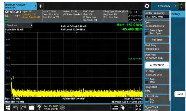
Band4-5MHz-QPSK-20375-1RB#0-0.15~30-PASS
