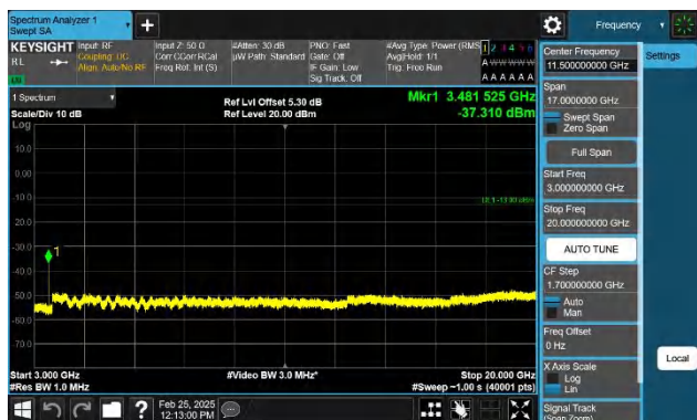
Band4-15MHz-QPSK-20325-1RB#0-3000~20000-PASS
