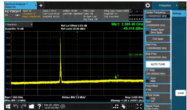
Band4-10MHz-QPSK-20350-1RB#0-1000~3000-PASS
