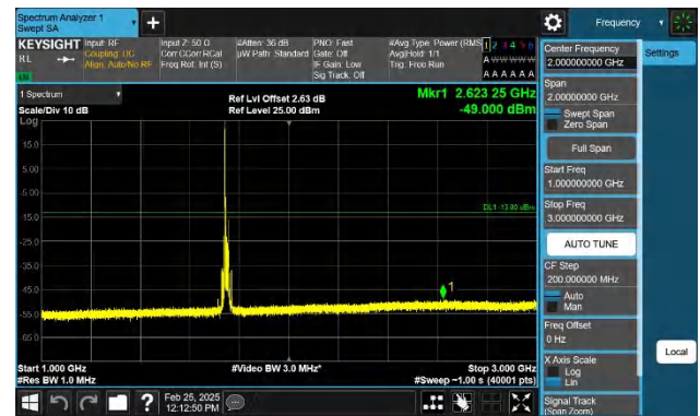
Band4-15MHz-QPSK-20325-1RB#0-1000~3000-PASS
