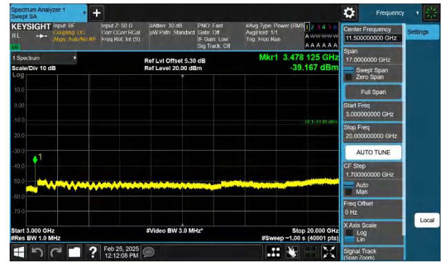
Band4-15MHz-QPSK-20175-1RB#74-3000~20000-PASS
