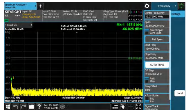
Band4-10MHz-QPSK-20350-1RB#0-0.15~30-PASS
