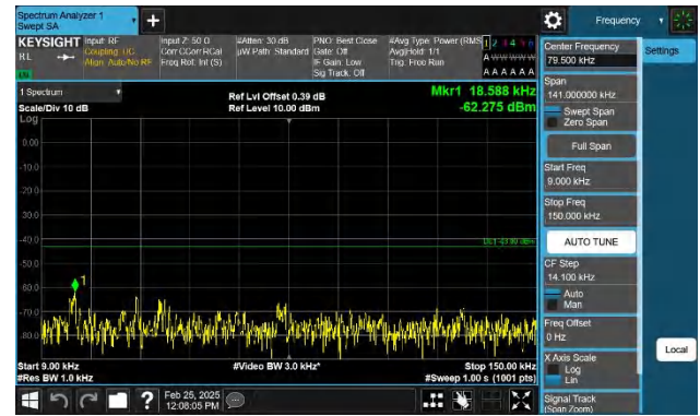
Band4-10MHz-QPSK-20350-1RB#49-0.009~0.15-PASS
