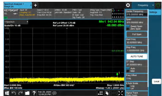
Band4-10MHz-QPSK-20350-1RB#49-30~1000-PASS
