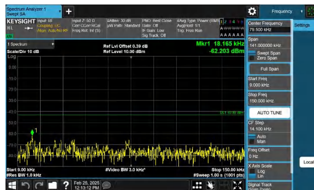
Band4-15MHz-QPSK-20325-1RB#74-0.009~0.15-PASS
