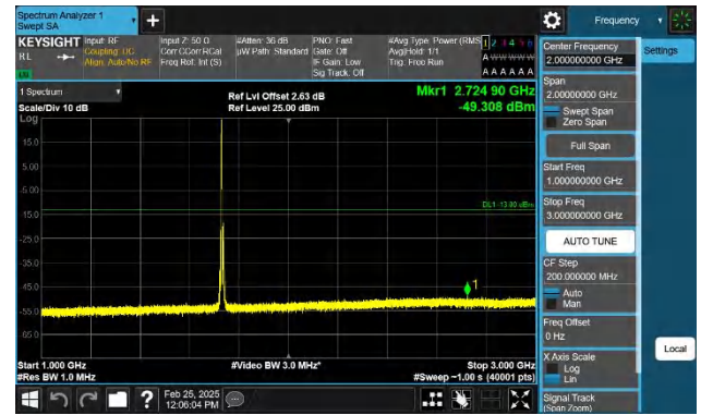
Band4-10MHz-QPSK-20175-1RB#0-1000~3000-PASS
