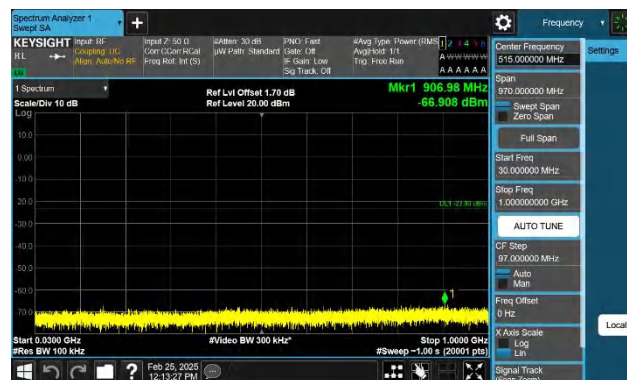
Band4-15MHz-QPSK-20325-1RB#74-30~1000-PASS
