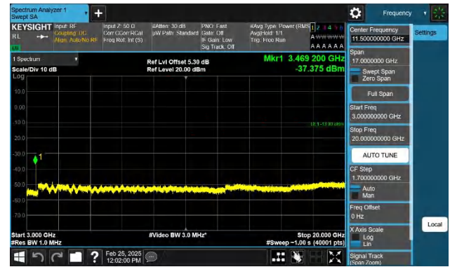
Band4-5MHz-QPSK-20175-1RB#24-3000~20000-PASS
