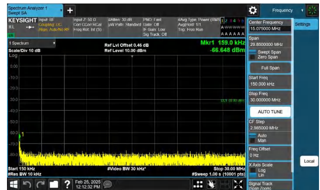
Band4-15MHz-QPSK-20325-1RB#0-0.15~30-PASS
