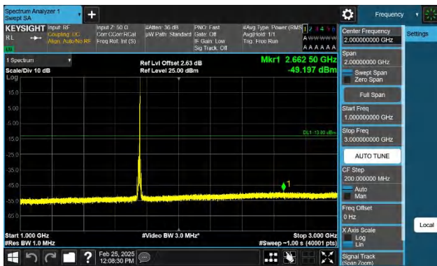
Band4-10MHz-QPSK-20350-1RB#49-1000~3000-PASS
