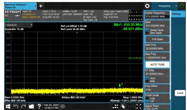
Band4-10MHz-QPSK-20175-1RB#49-30~1000-PASS
