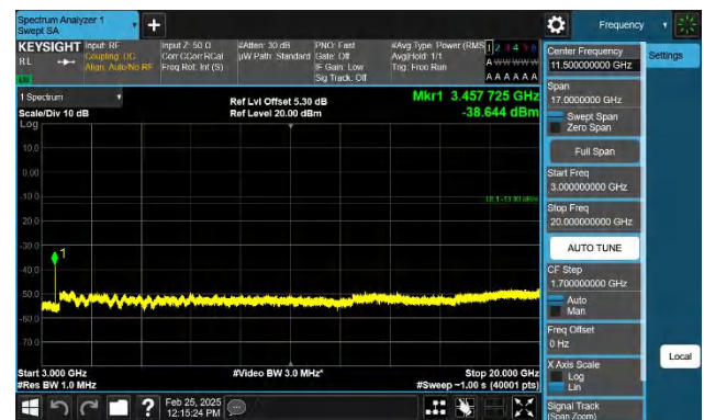
Band4-20MHz-QPSK-20050-1RB#99-3000~20000-PASS
