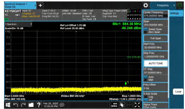
Band4-5MHz-QPSK-19975-1RB#24-30~1000-PASS
