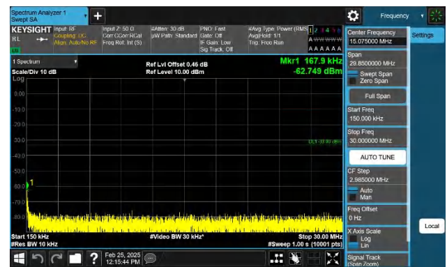
Band4-20MHz-QPSK-20175-1RB#0-0.15~30-PASS
