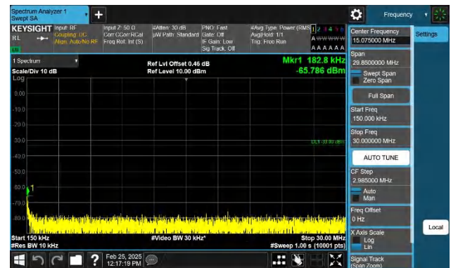
Band4-20MHz-QPSK-20300-1RB#0-0.15~30-PASS
