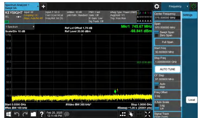
Band4-15MHz-QPSK-20175-1RB#74-30~1000-PASS
