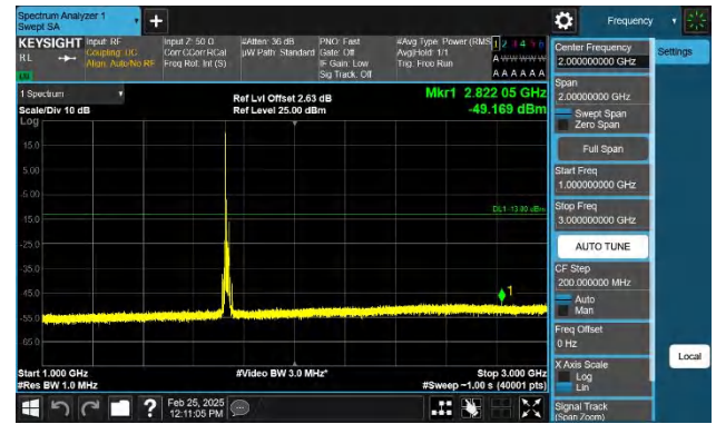
Band4-15MHz-QPSK-20175-1RB#0-1000~3000-PASS
