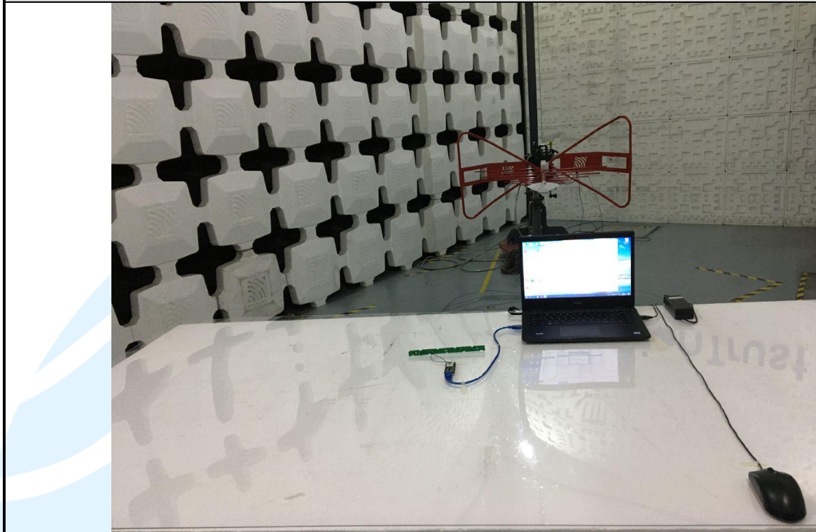
Radiated emission Test Setup (Below 1GHz)
