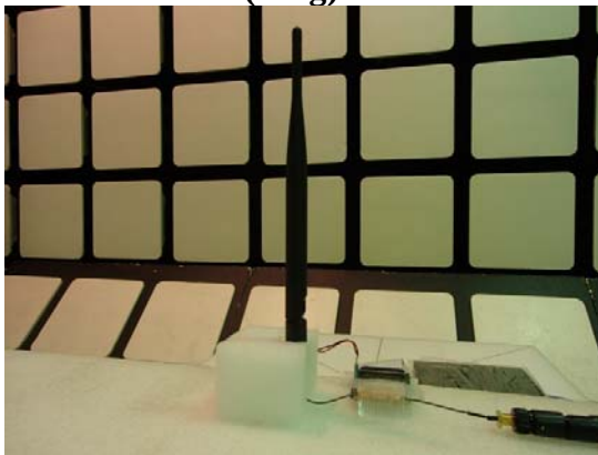
Z1(0deg)-axis
