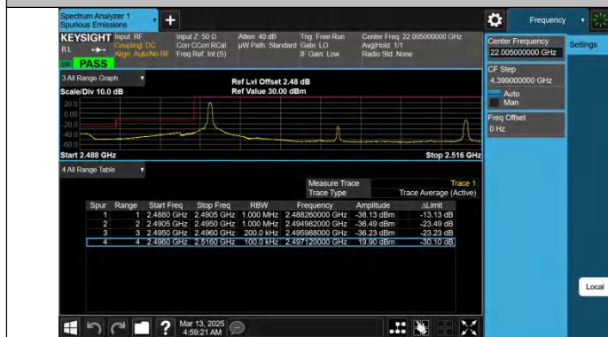
Band41-20MHz-QPSK-39750-1RB#0-PASS
