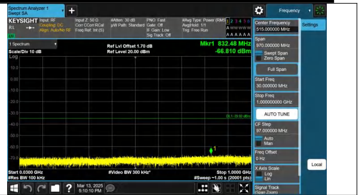
Band41-5MHz-QPSK-40620-1RB#24-30~1000-PASS
