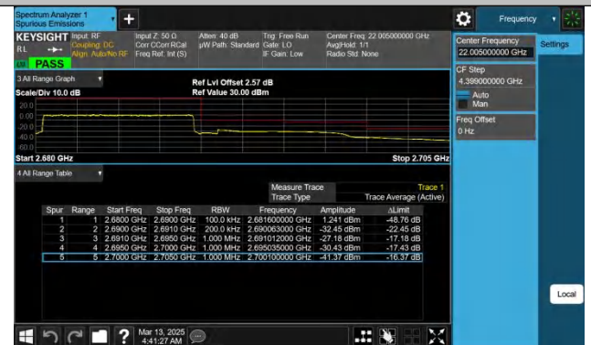
Band41-10MHz-QPSK-41540-50RB#0-PASS
