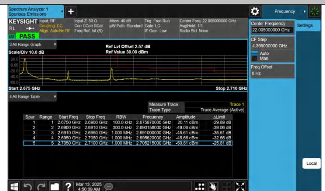
Band41-15MHz-QPSK-41515-1RB#0-PASS
