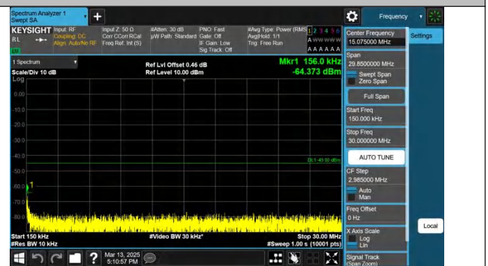
Band41-5MHz-QPSK-41565-1RB#0-0.15~30-PASS
