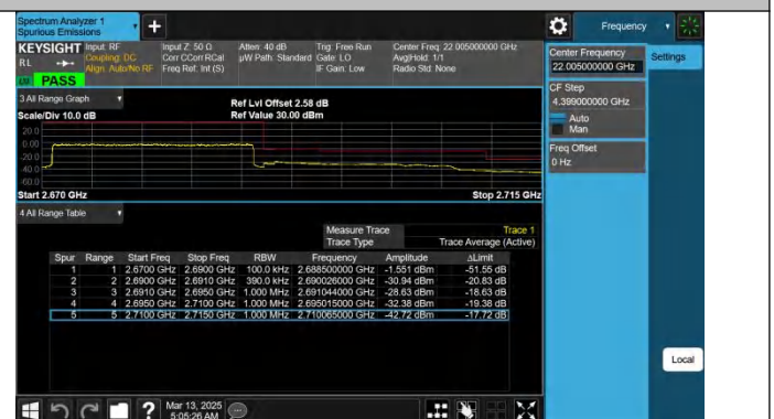
Band41-20MHz-QPSK-41490-100RB#0-PASS
