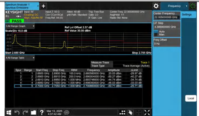
Band41-10MHz-QPSK-41540-1RB#0-PASS
