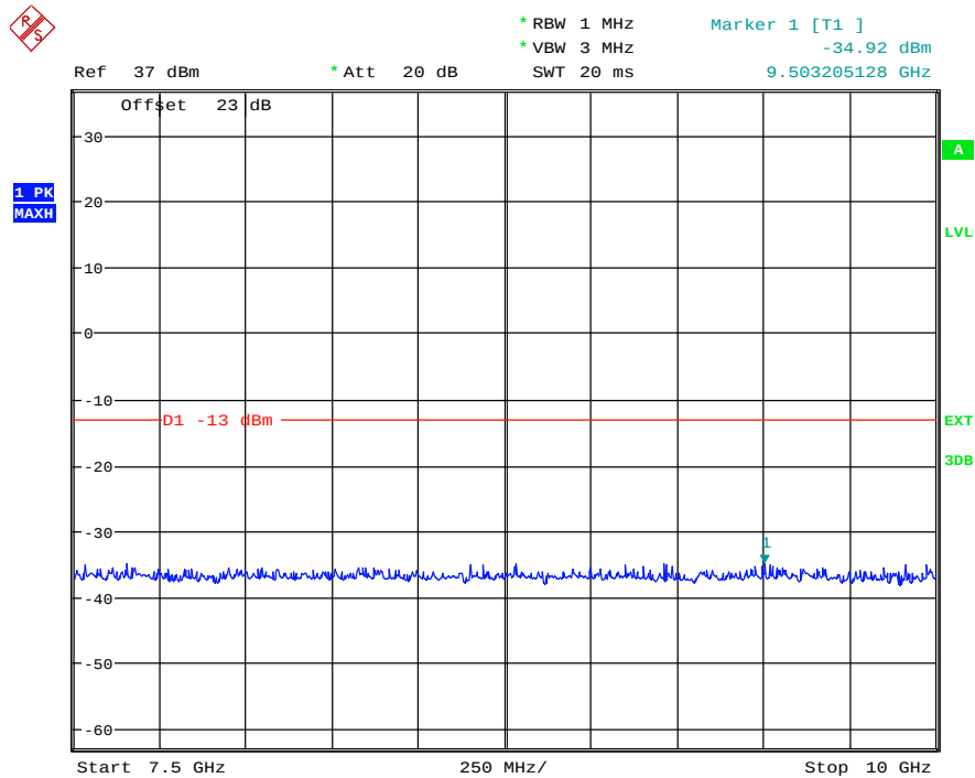
(Plot 4.6.1 D5: Idle @ GSM850)
