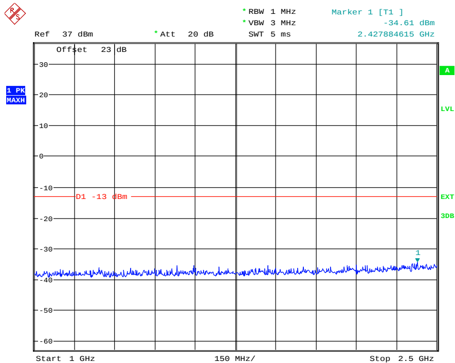
(Plot 4.6.1 D3: Idle @ GSM850)
