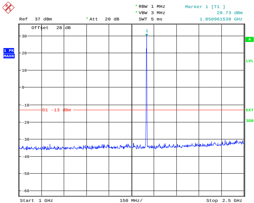
(Plot 4.6.2 A3: Channel 512: 1850.20MHz @ Traffic @ PCS1900)
