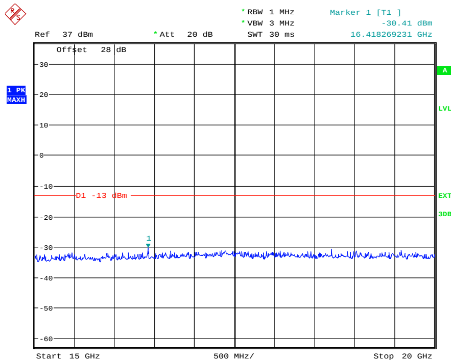
(Plot 4.6.2 A7: Channel 512: 1850.20MHz @ Traffic @ PCS1900)
