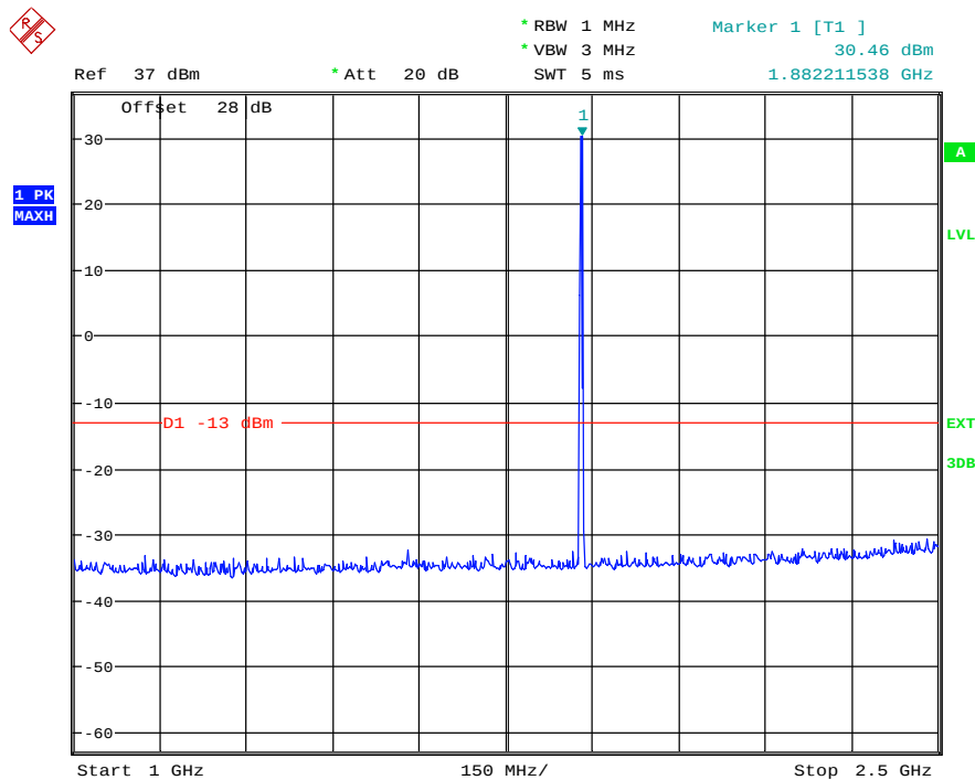
(Plot 4.6.2 B3: Channel 661: 1880.00MHz @ Traffic @ PCS1900)
