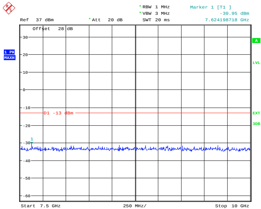
(Plot 4.6.2 A5: Channel 512: 1850.20MHz @ Traffic @ PCS1900)
