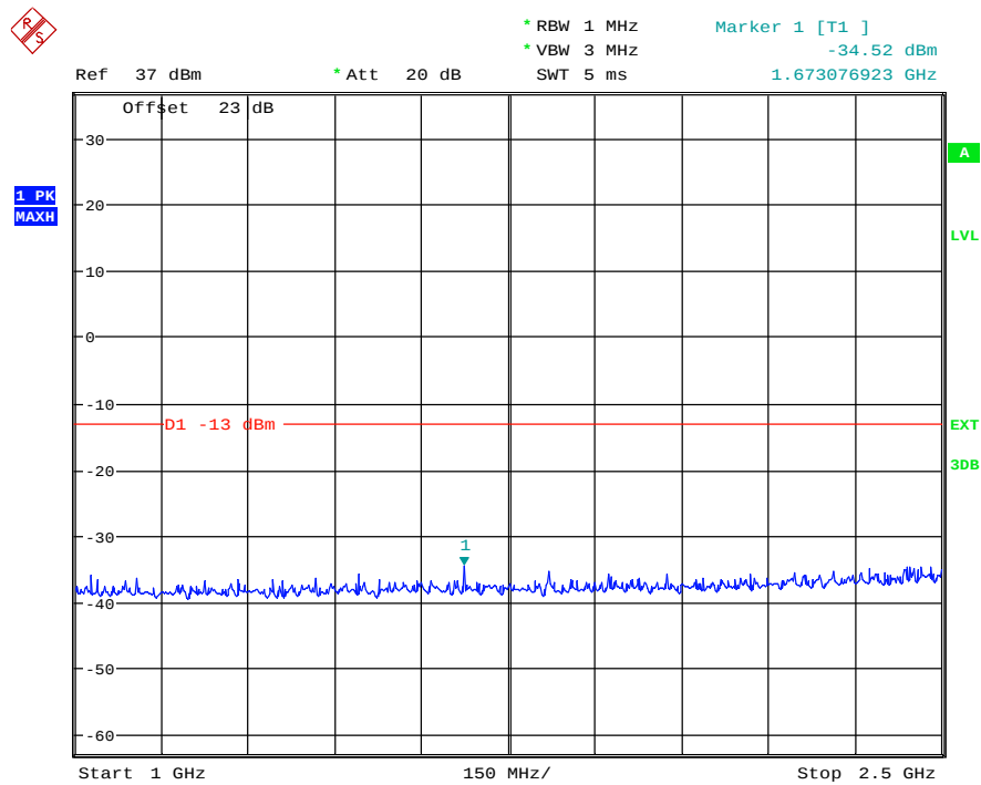
(Plot 4.6.1 B3: Channel 190: 836.60MHz @ Traffic @ GSM850)
