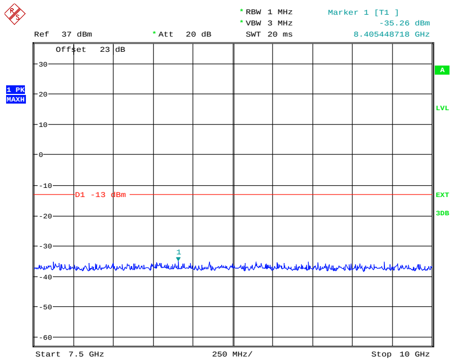
(Plot 4.6.1 B5: Channel 190: 836.60MHz @ Traffic @ GSM850)
