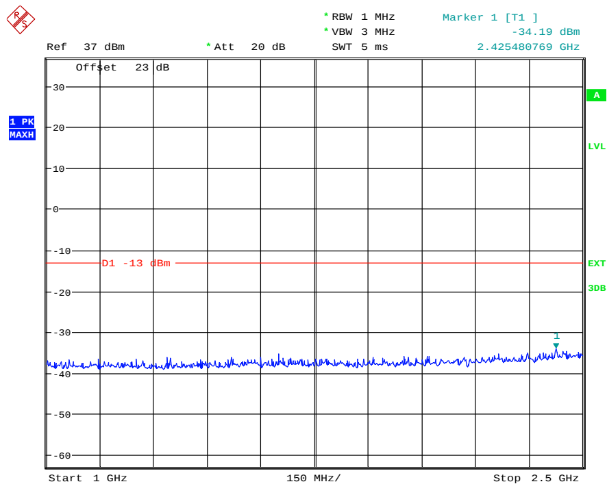
(Plot 5.5.1 A3: Channel 128: 824.20MHz @ Traffic @ GSM850)
