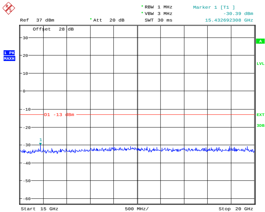
(Plot 4.6.2 D7: Idle @ PCS1900)
