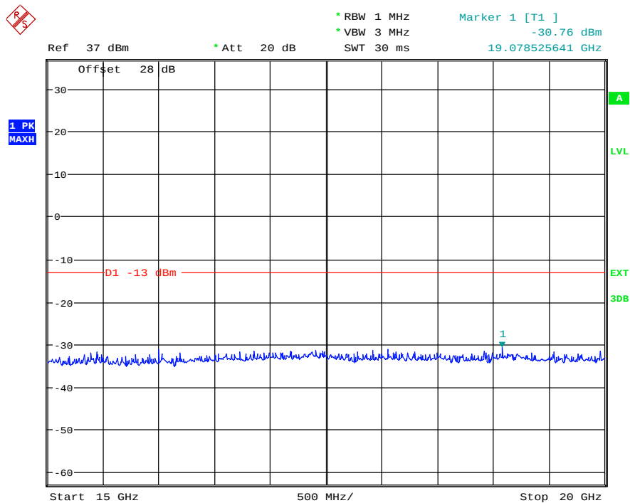
(Plot 4.6.2 B7: Channel 661: 1880.00MHz @ Traffic @ PCS1900)
