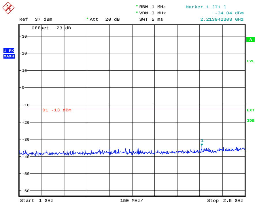
(Plot 4.6.1 C3: Channel 251: 848.80MHz @ Traffic @ GSM850)
