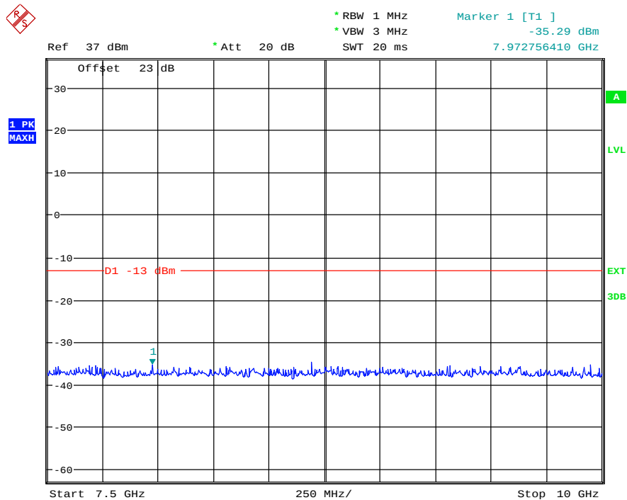
(Plot 4.6.1 C5: Channel 251: 848.80MHz @ Traffic @ GSM850)
