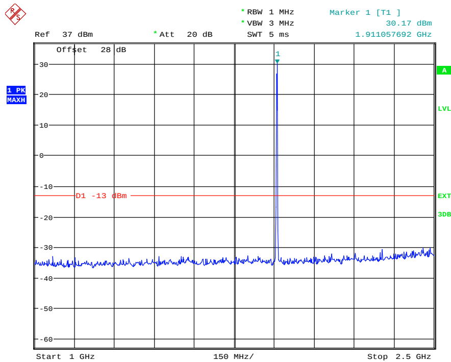
(Plot 4.6.2 C3: Channel 810: 1909.80MHz @ Traffic @ PCS1900)
