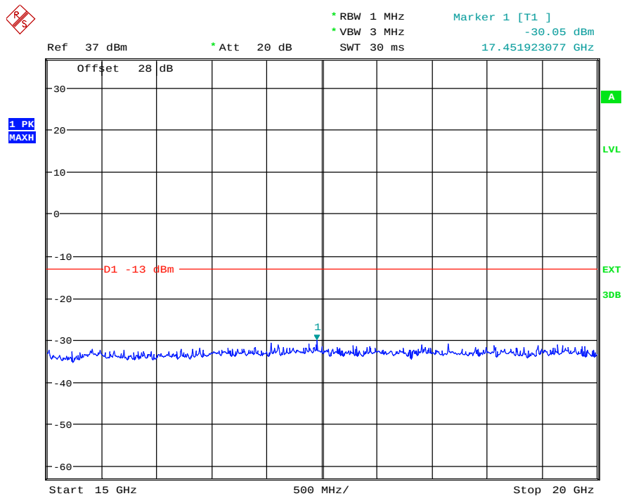
(Plot 4.6.2 C7: Channel 810: 1909.80MHz @ Traffic @ PCS1900)
