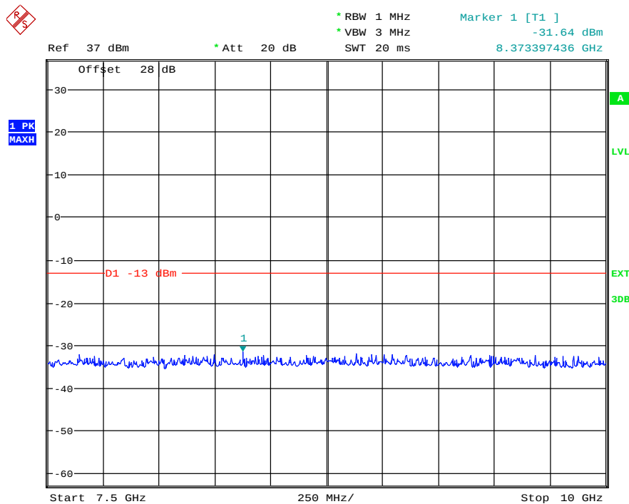
(Plot 4.6.2 C5: Channel 810: 1909.80MHz @ Traffic @ PCS1900)
