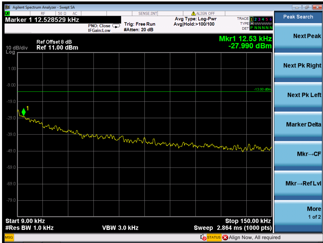
(Plot 4.6.2 C1: Channel 810: 1909.80MHz @ Traffic @ PCS1900)
