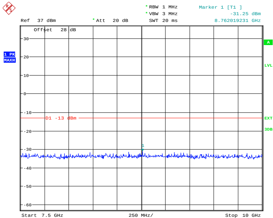
(Plot 4.6.2 D5: Idle @ PCS1900)
