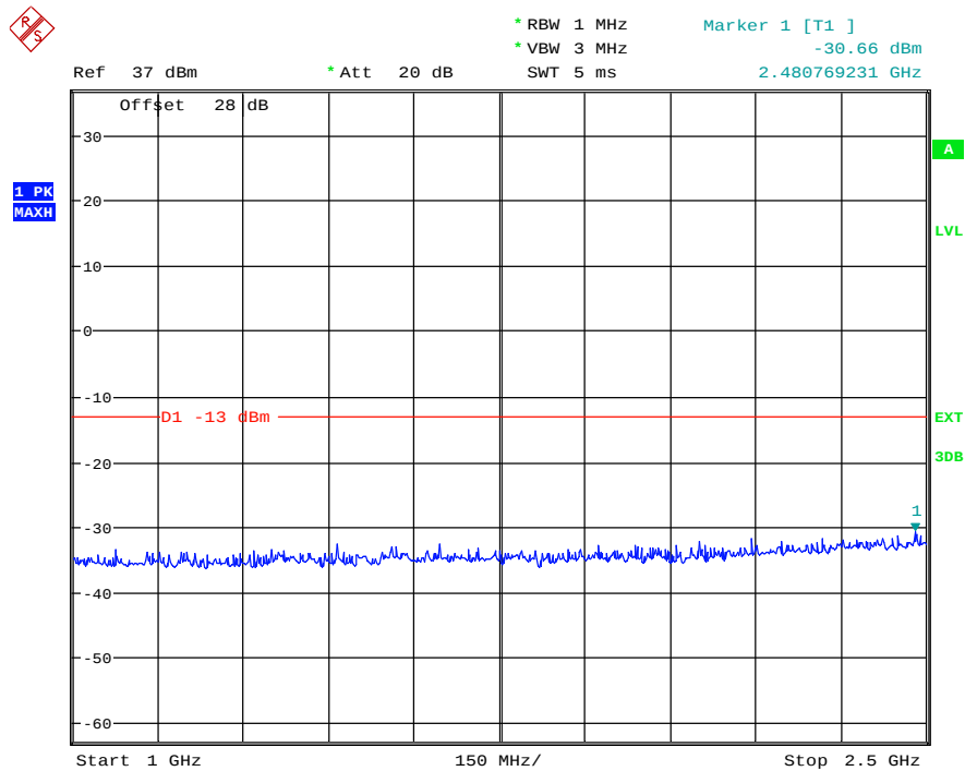
(Plot 4.6.2 D3: Idle @ PCS1900)
