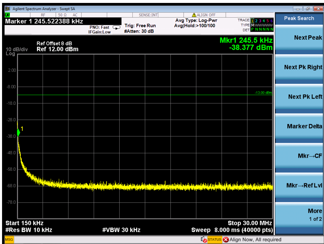
(Plot 4.6.2 C2: Channel 810: 1909.80MHz @ Traffic @ PCS1900)
