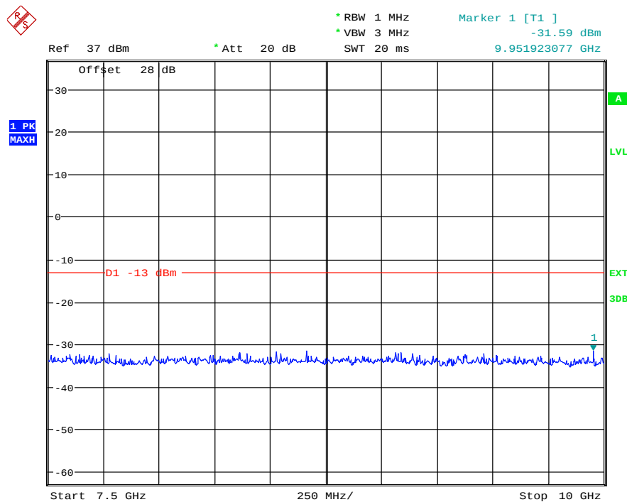
(Plot 4.6.2 B5: Channel 661: 1880.00MHz @ Traffic @ PCS1900)
