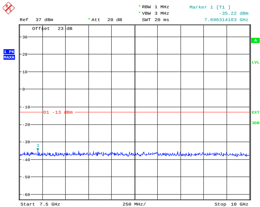
(Plot 4.6.1 A5: Channel 128: 824.20MHz @ Traffic @ GSM850)
