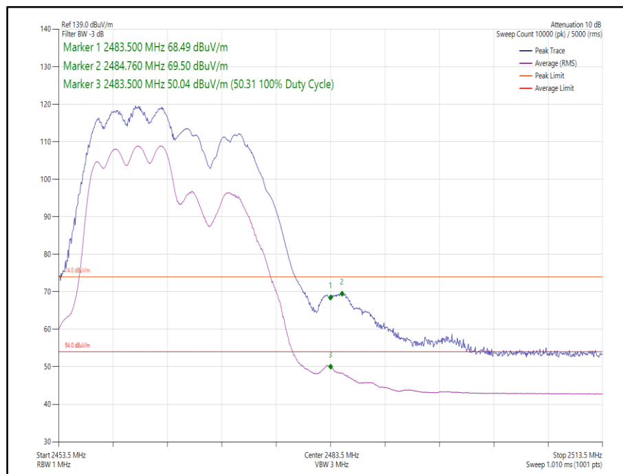
Figure 50 - 802.11ax, HE20, RU 106-53, CDD, Core 0-1 - 2467 MHz, Band Edge Frequency 2483.5 MHz
