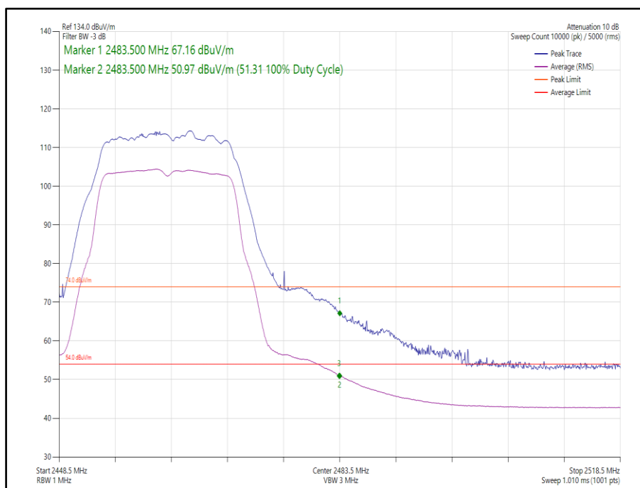
Figure 29 - 802.11g, SISO, Core 1 - 2462 MHz, Band Edge Frequency 2483.5 MHz
