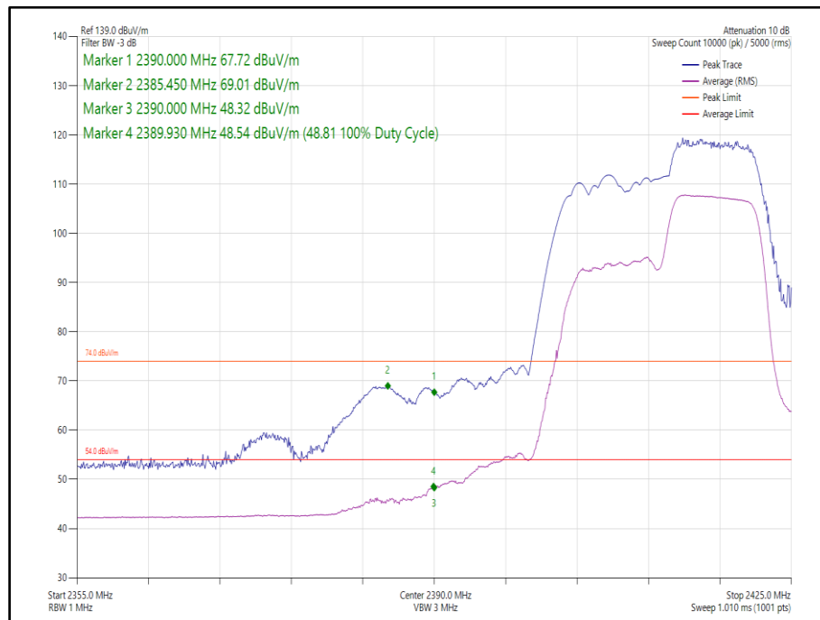
Figure 25 - 802.11ax, HE20, RU 106-54, SISO, Core 1 - 2412 MHz, Band Edge Frequency 2390 MHz
