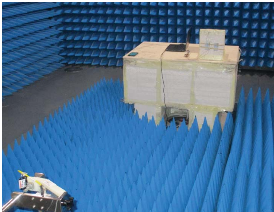
Photo 3 Photograph radiated emissions 18 – 26.5 GHz
