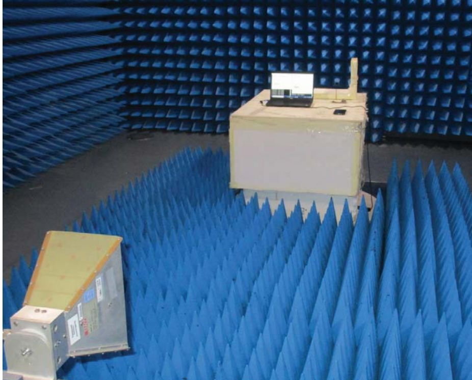
Photo 2 Photograph radiated emissions 1 – 18 GHz
